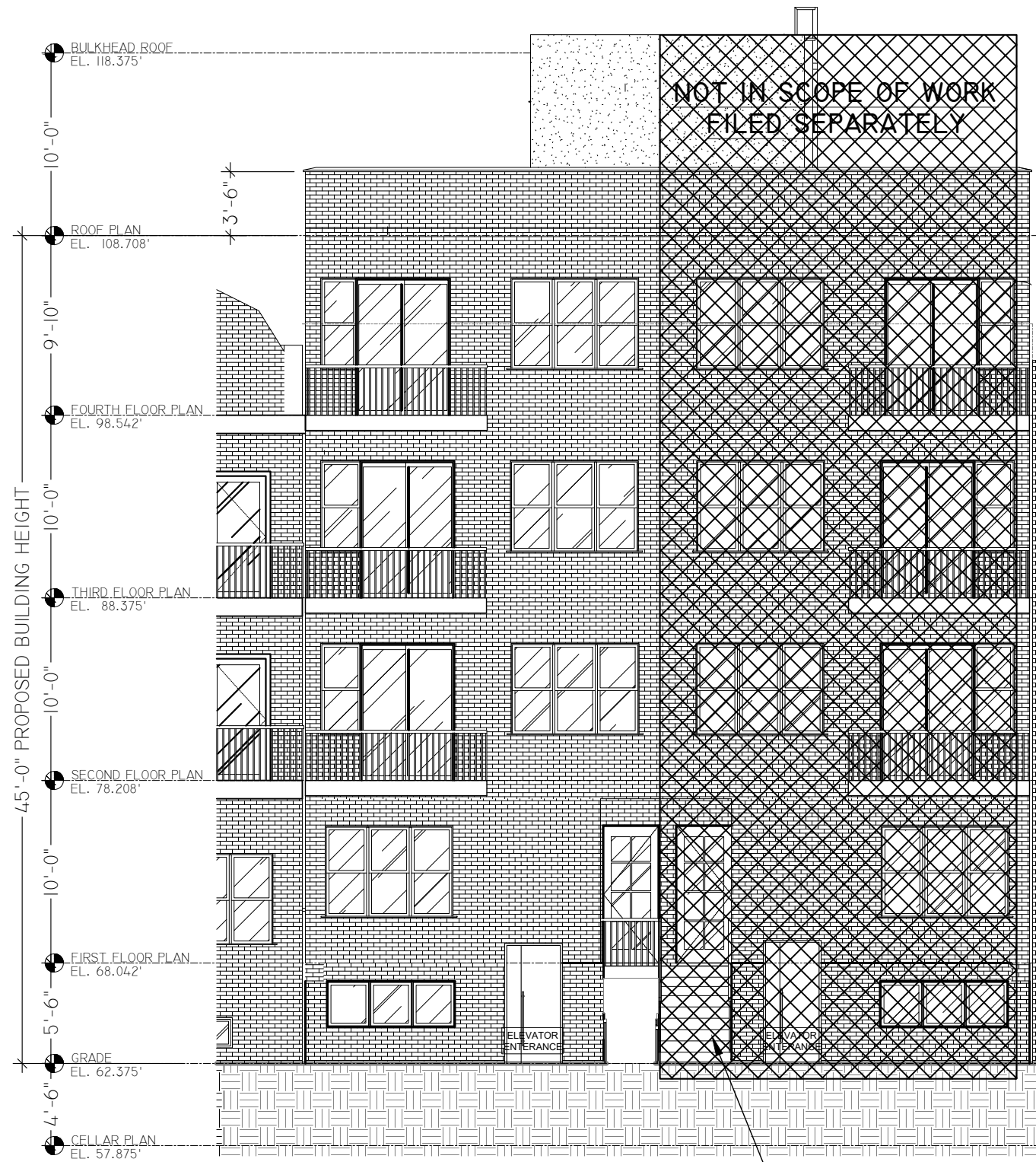
FRONT ELEVATION
