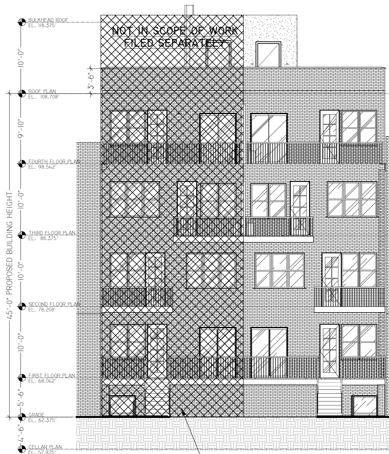
REAR ELEVATION
