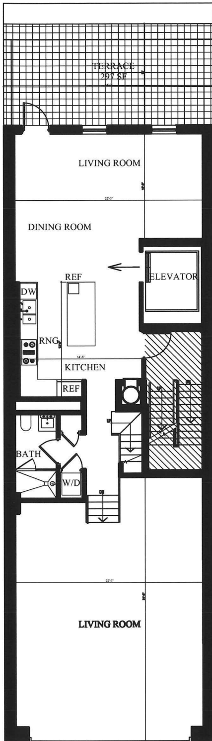
6TH FLOOR PLAN
