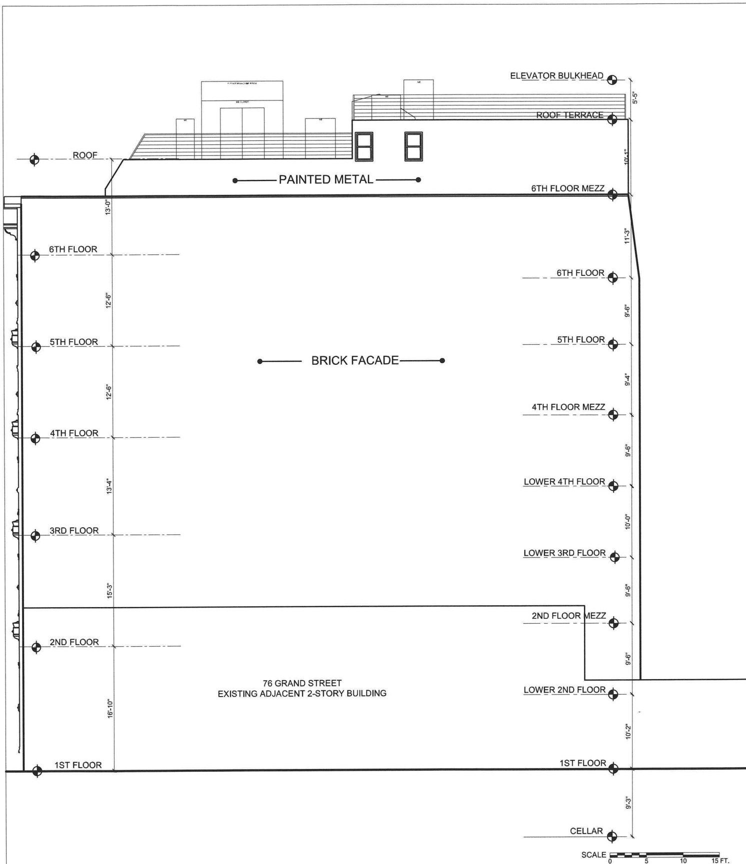
EAST ELEVATION
