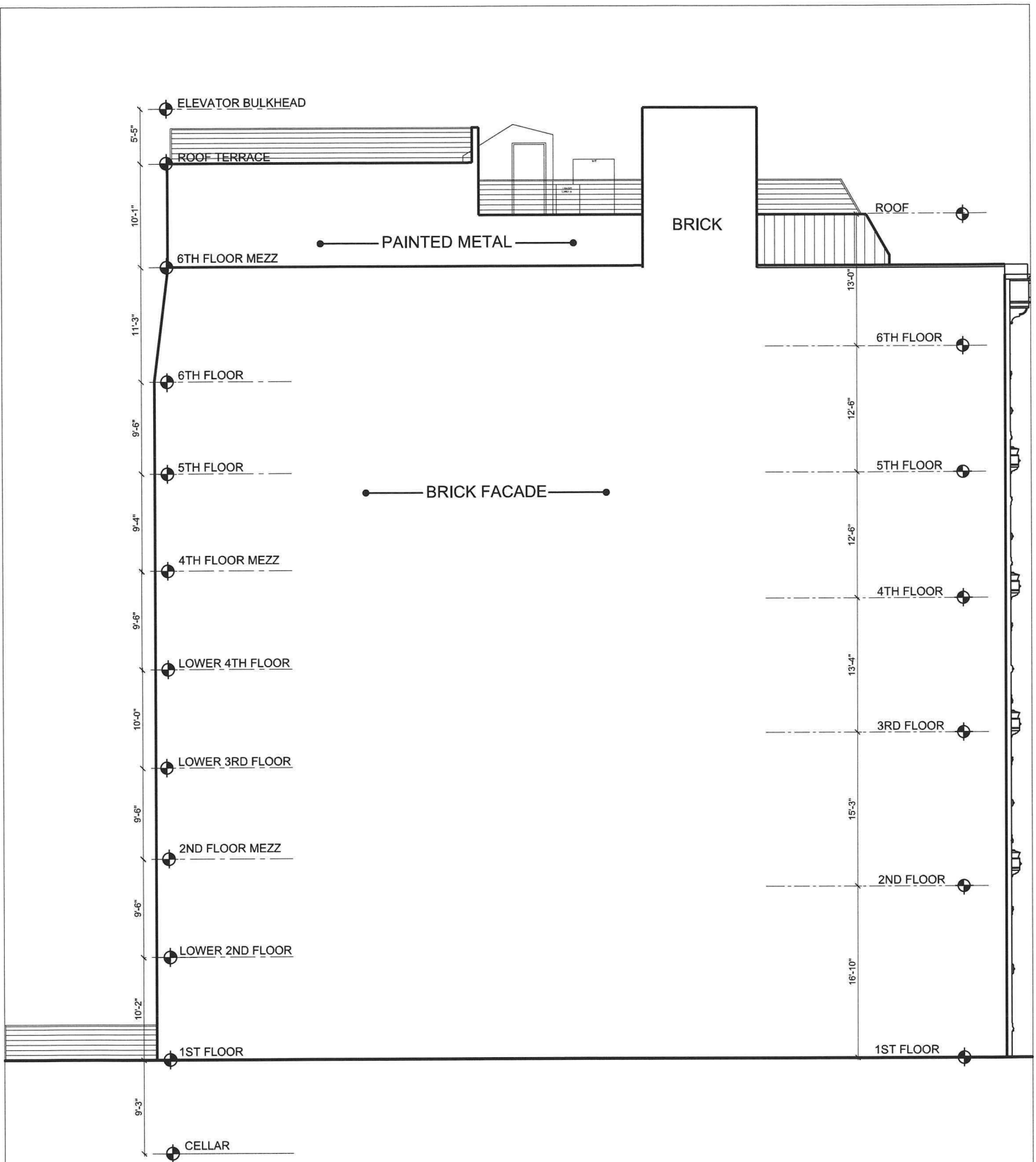
WEST ELEVATION
