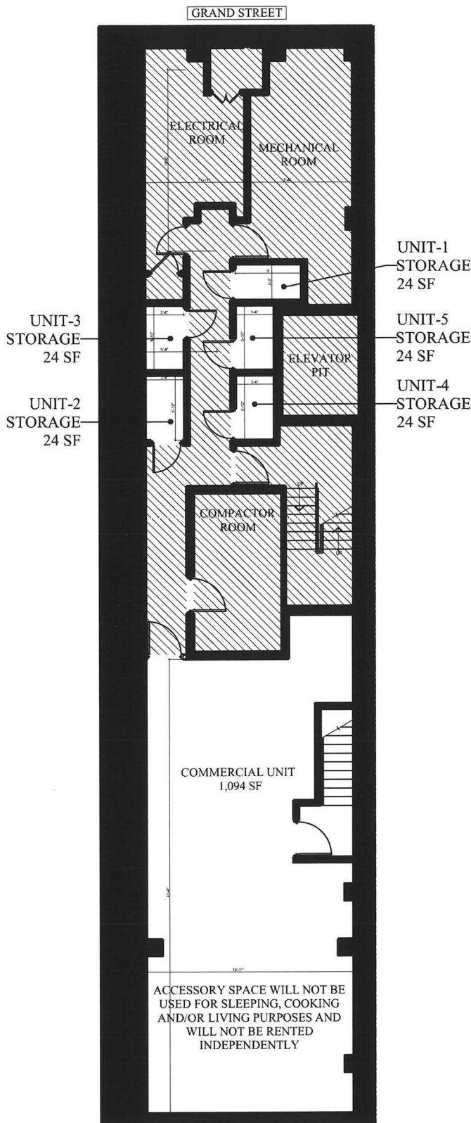
CELLAR PLAN
