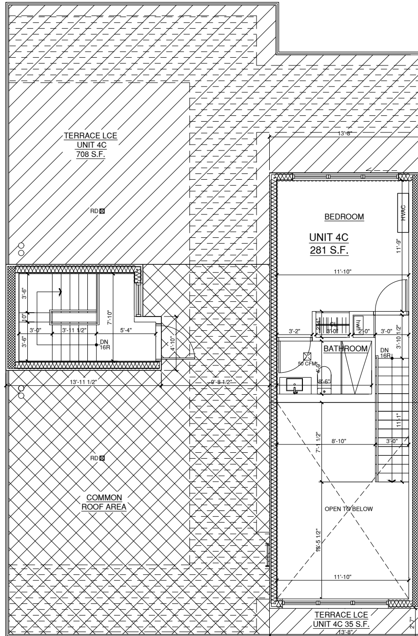
PENTHOUSE FLOOR PLAN
