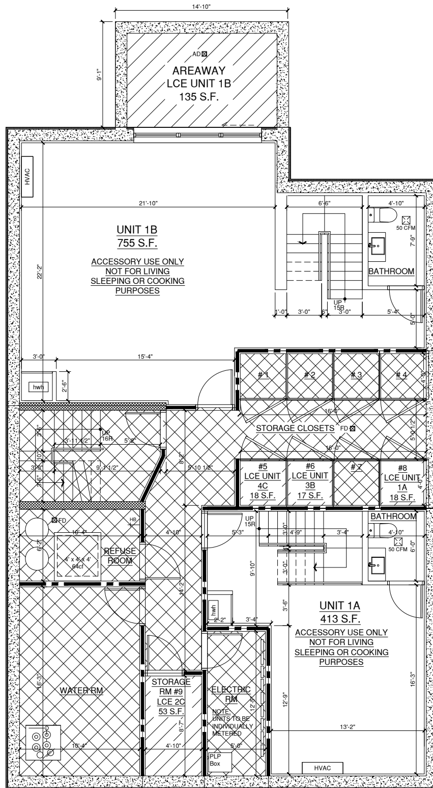
CELLAR FLOOR PLAN
