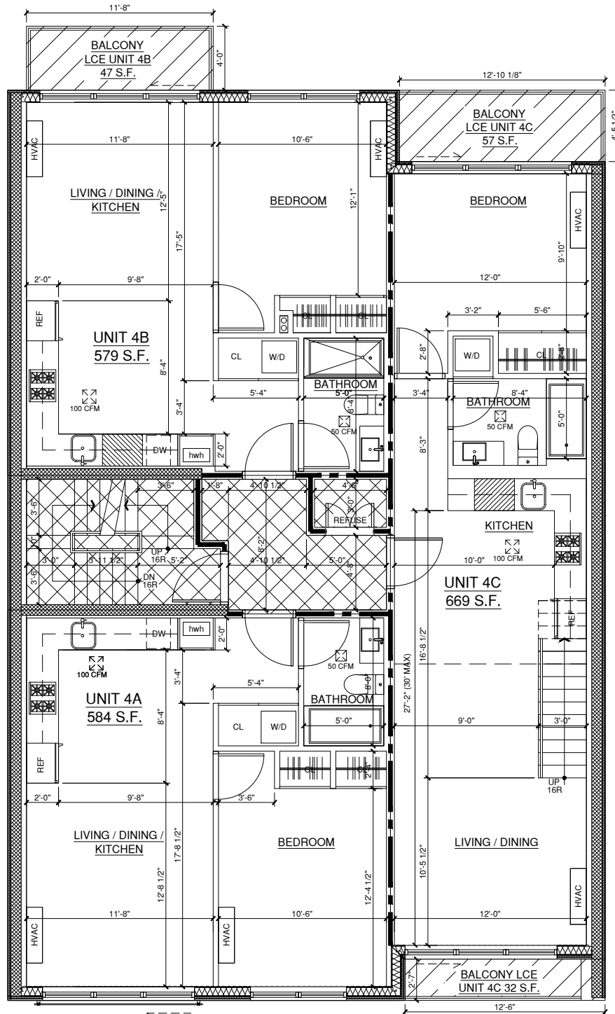
FOURTH FLOOR PLAN
