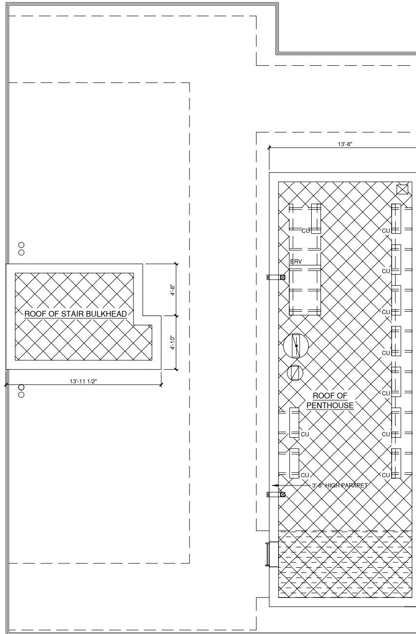
ROOF FLOOR PLAN
