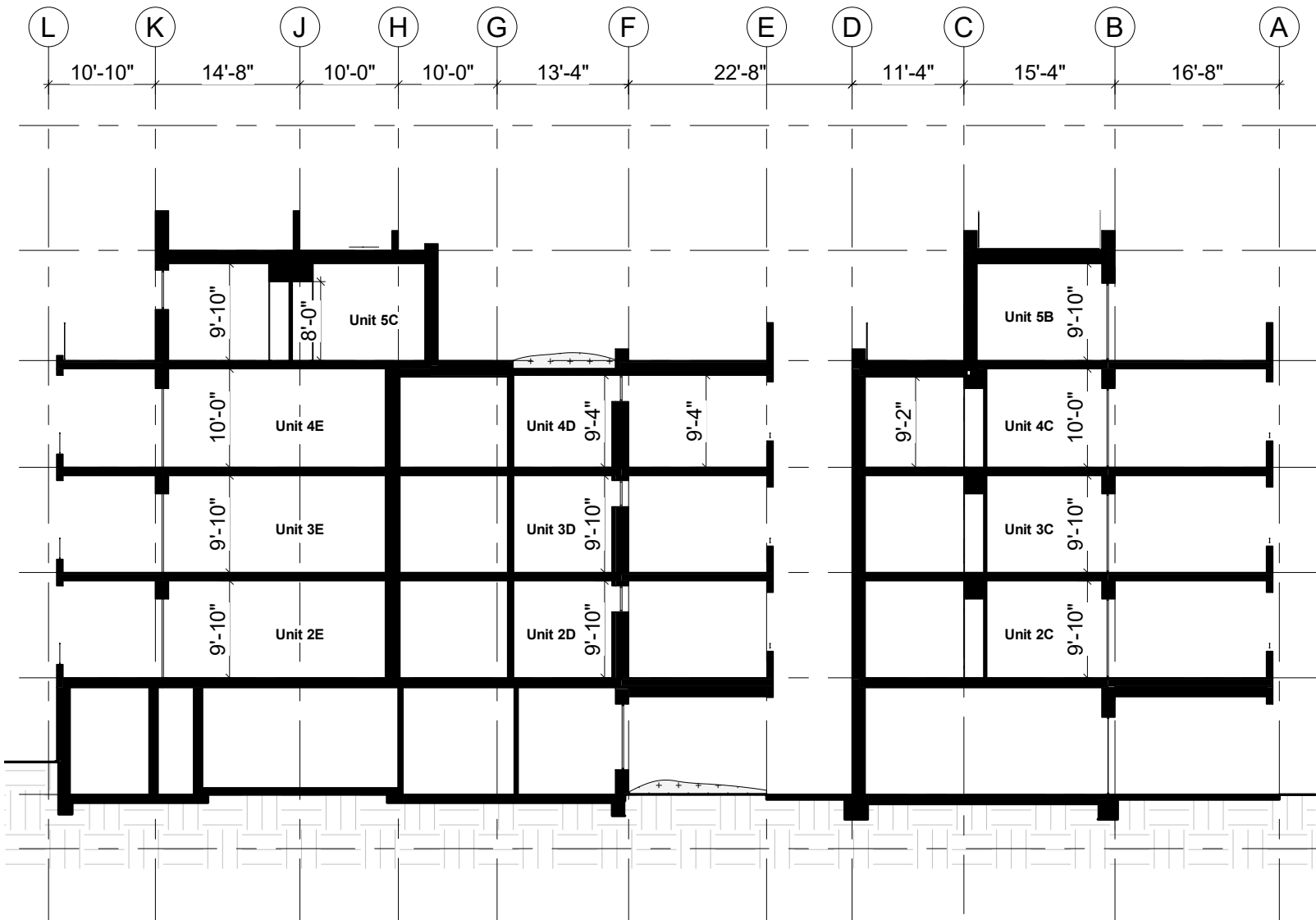
1 Section 1-1 1/16" = 1'-0"
