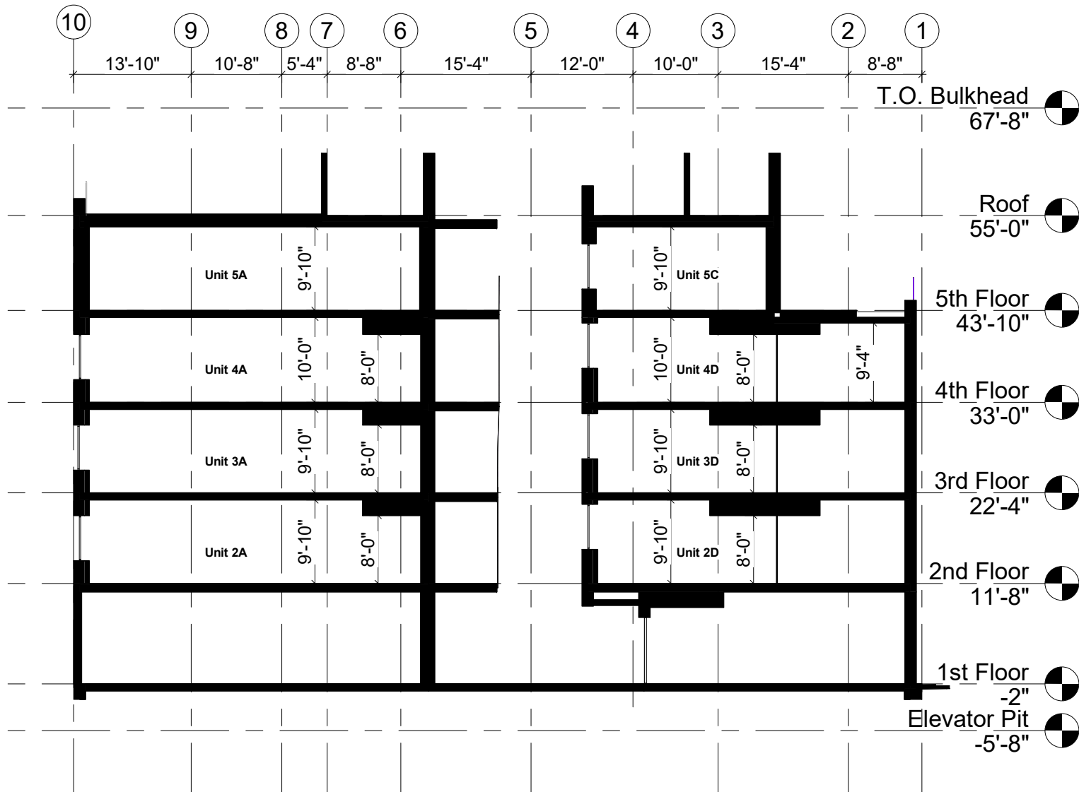
2 Section 2-2 1/16" = 1'-0"
