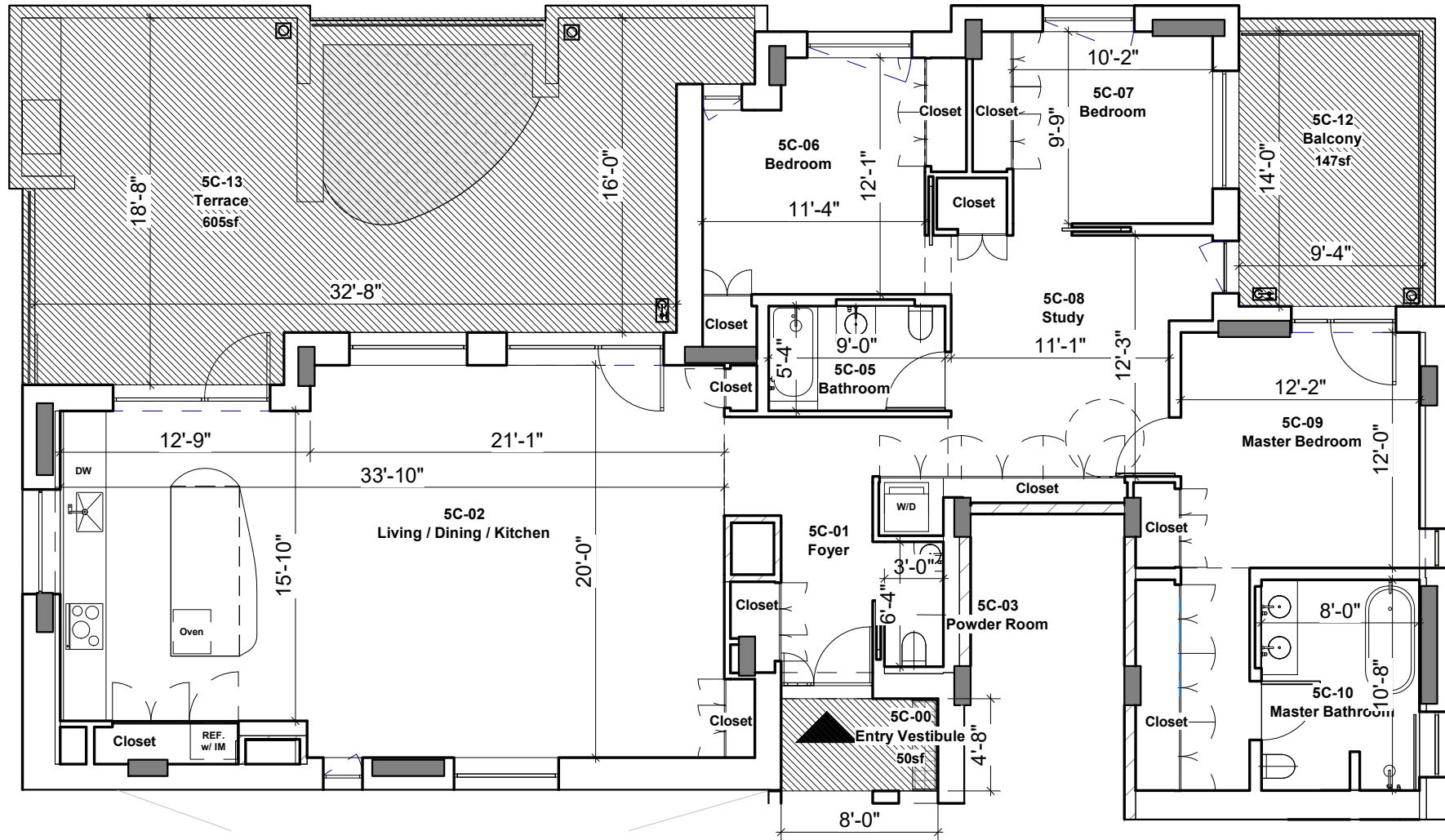
1 Unit Enlarged Floor Plan - 5C 1/8" = 1'-0"
