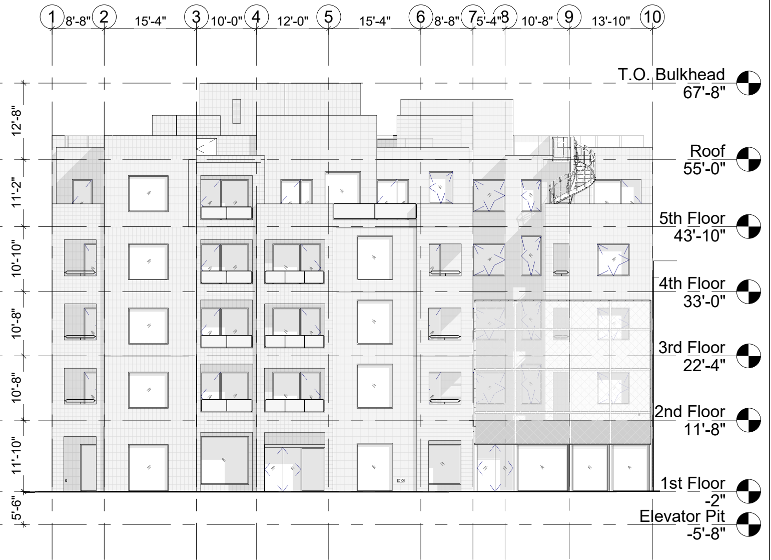
② West Elevation 1/16" = 1'-0"
