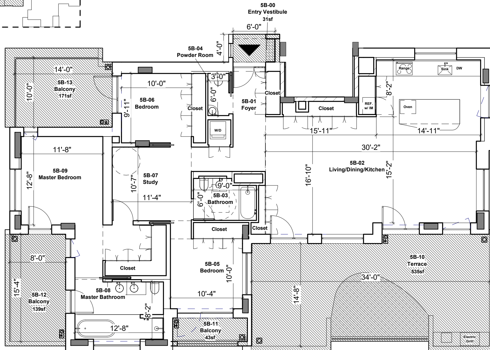
1 Unit Enlarged Floor Plan - 5B 1/8" = 1'-0"
