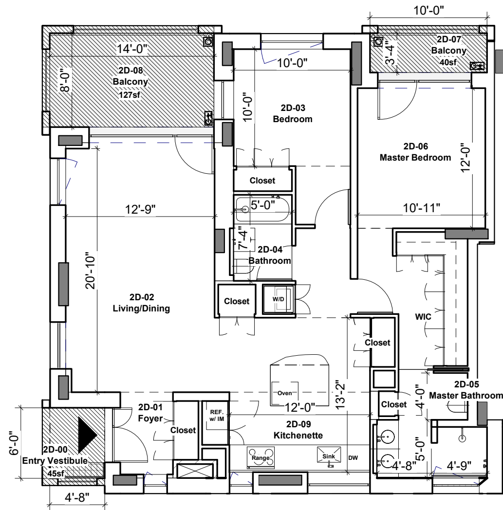
1 Unit Enlarged Floor Plan - 2D,3D,4D 1/8" = 1'-0"
