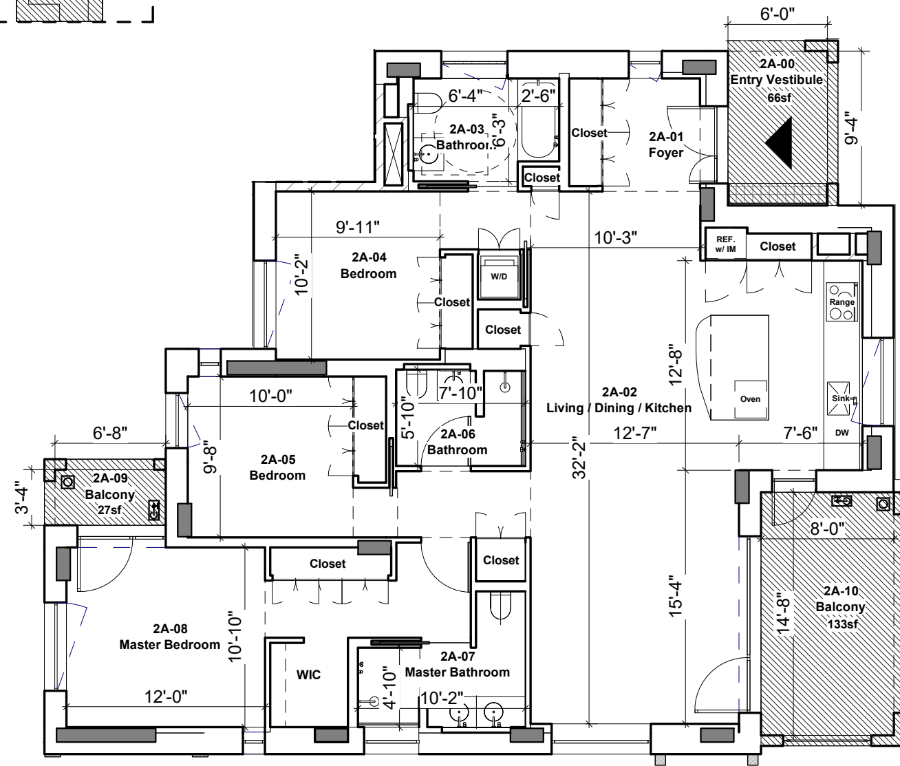
1 Unit Enlarged Floor Plan - 2A,3A,4A 1/8" = 1'-0"
