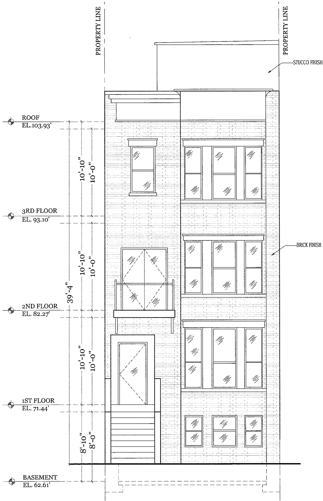
FRONT ELEVATION NOT SCALE
