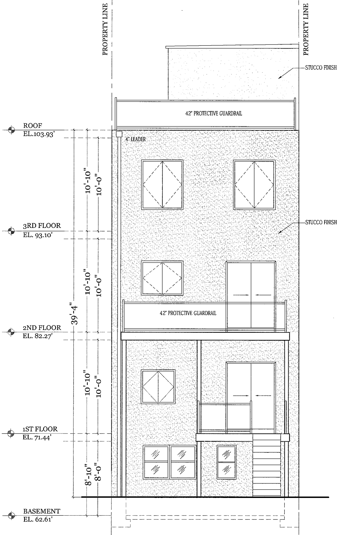
REAR ELEVATION NOT SCALE
