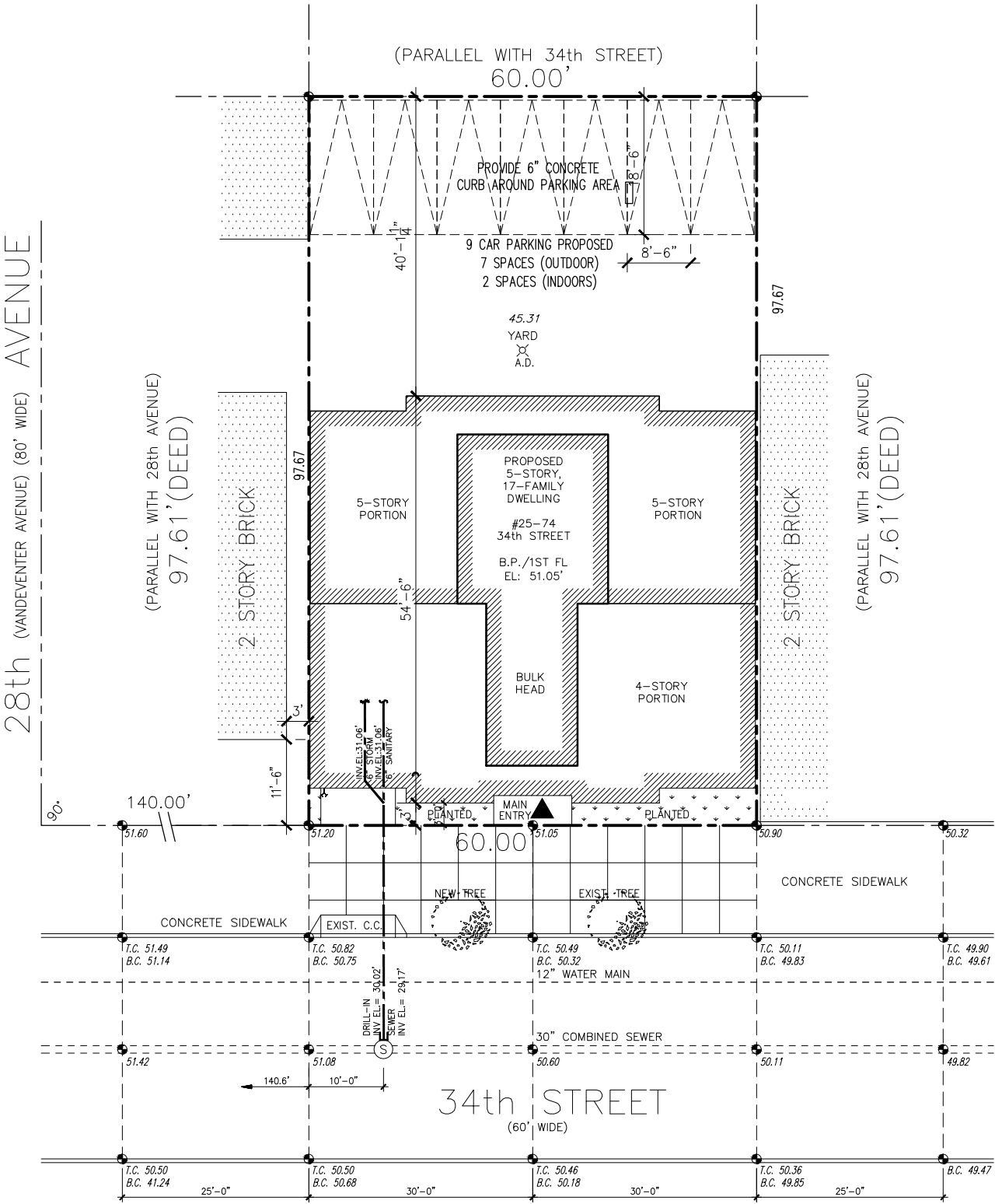
PLOT PLAN SCALE: 1"=20'-0"
