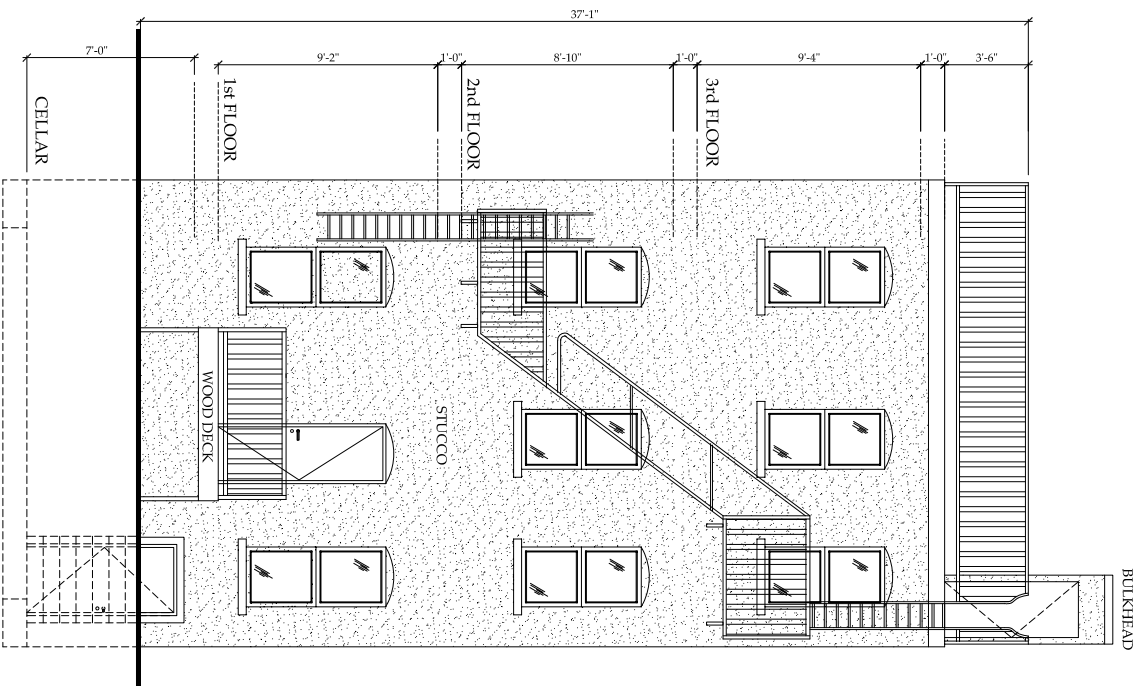
REAR ELEVATION
