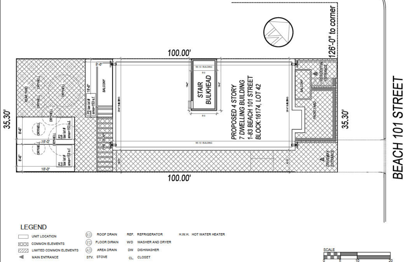
PLOT PLAN
