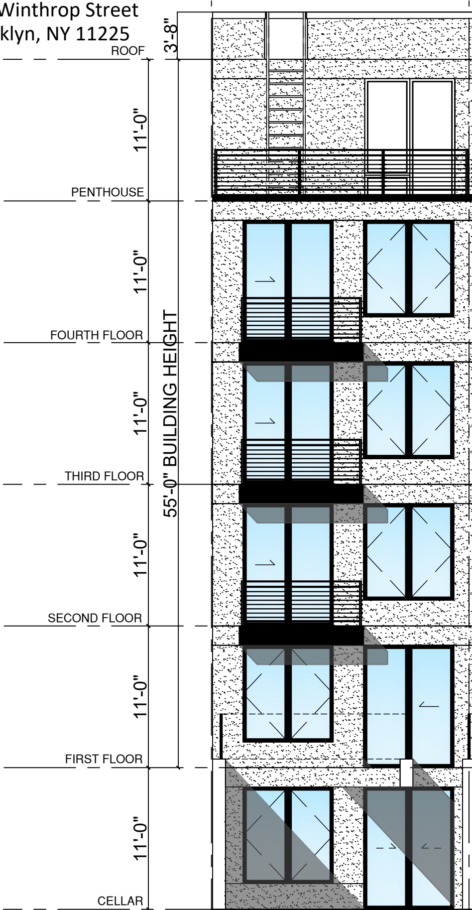
REAR ELEVATION
