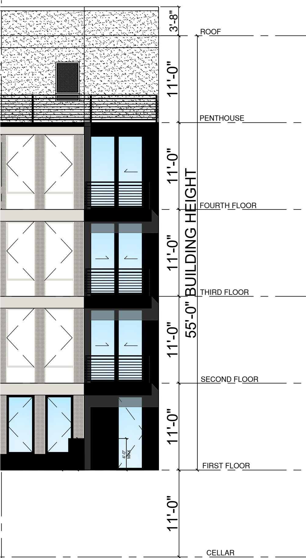
FRONT ELEVATION
