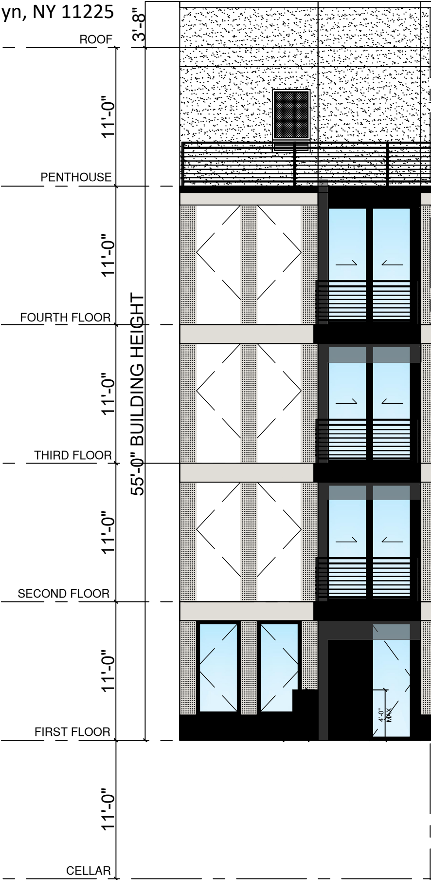
FRONT ELEVATION
