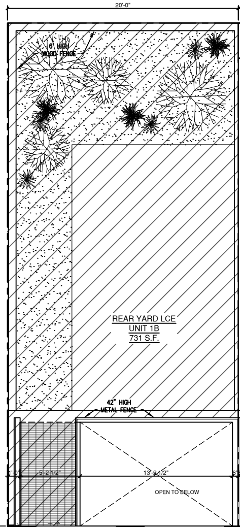
FIRST FLOOR PLAN REAR YARD CONTINUED
