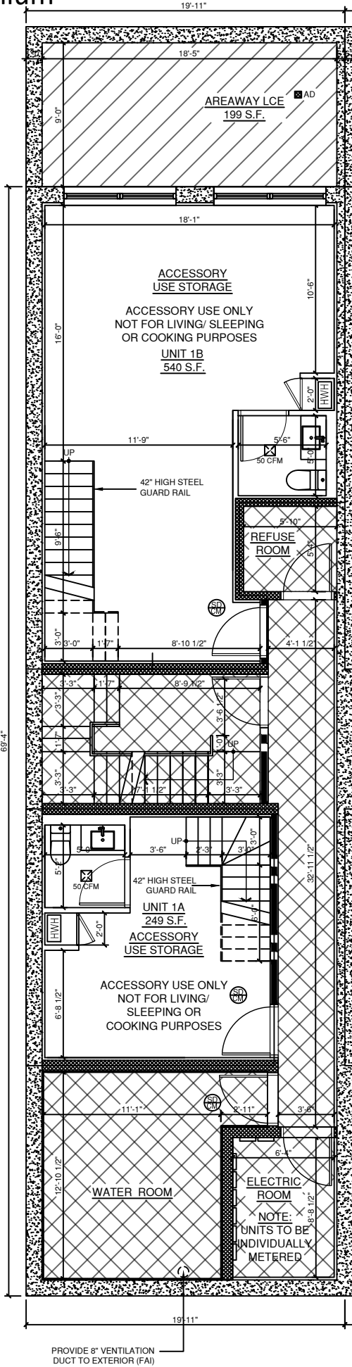
CELLAR FLOOR PLAN
