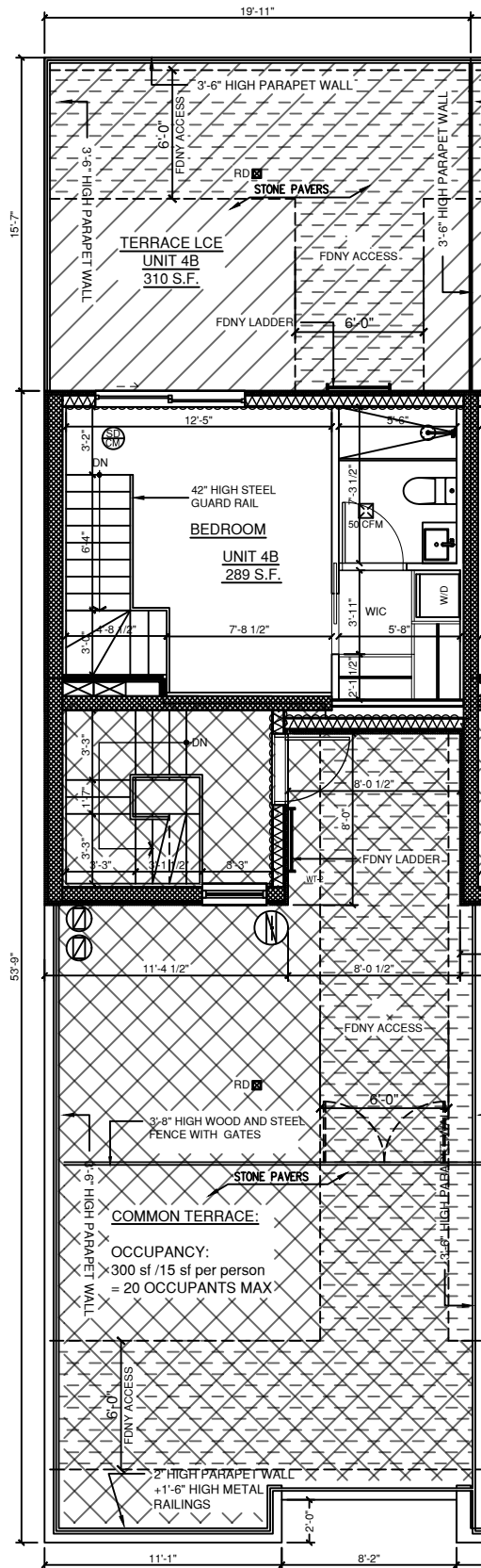
PENTHOUSE FLOOR PLAN
