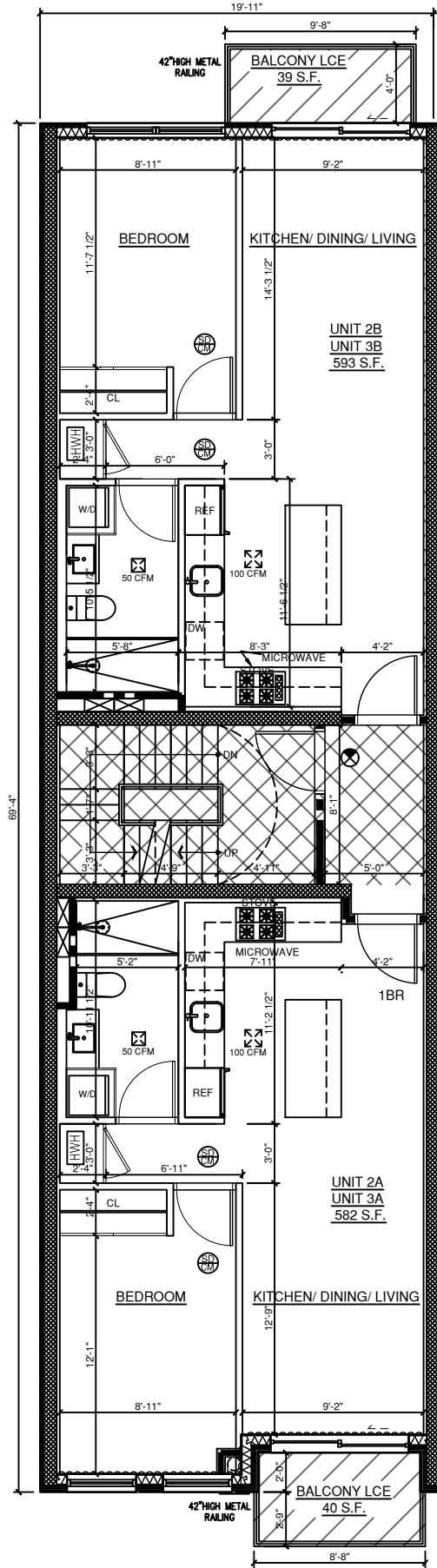
SECOND & THIRD FLOOR PLAN
