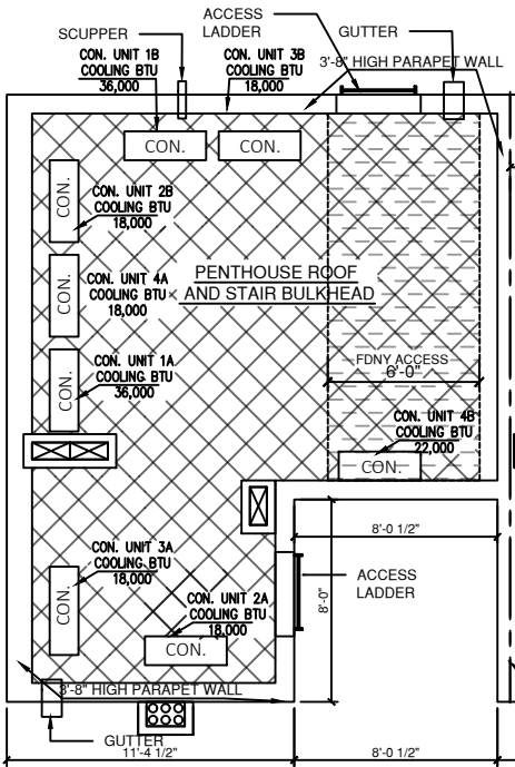
ROOF FLOOR PLAN
