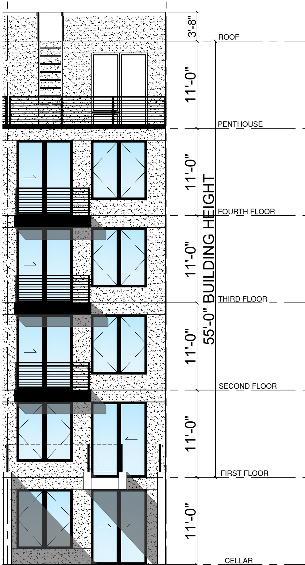
REAR ELEVATION
