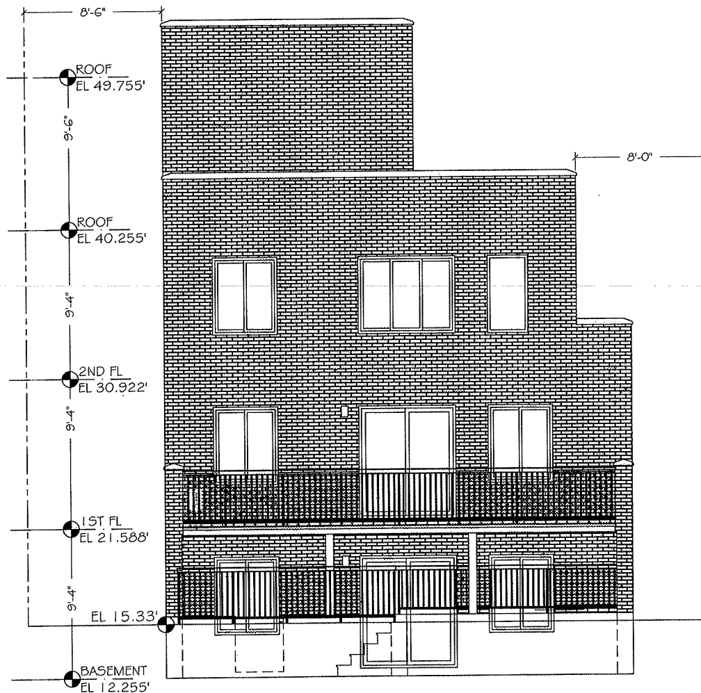
REAR ELEVATION
