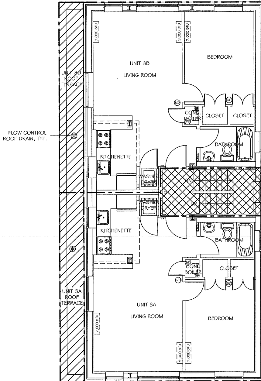
SECOND FLOOR KEY PLAN
