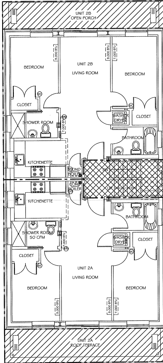
FIRST FLOOR KEY PLAN
