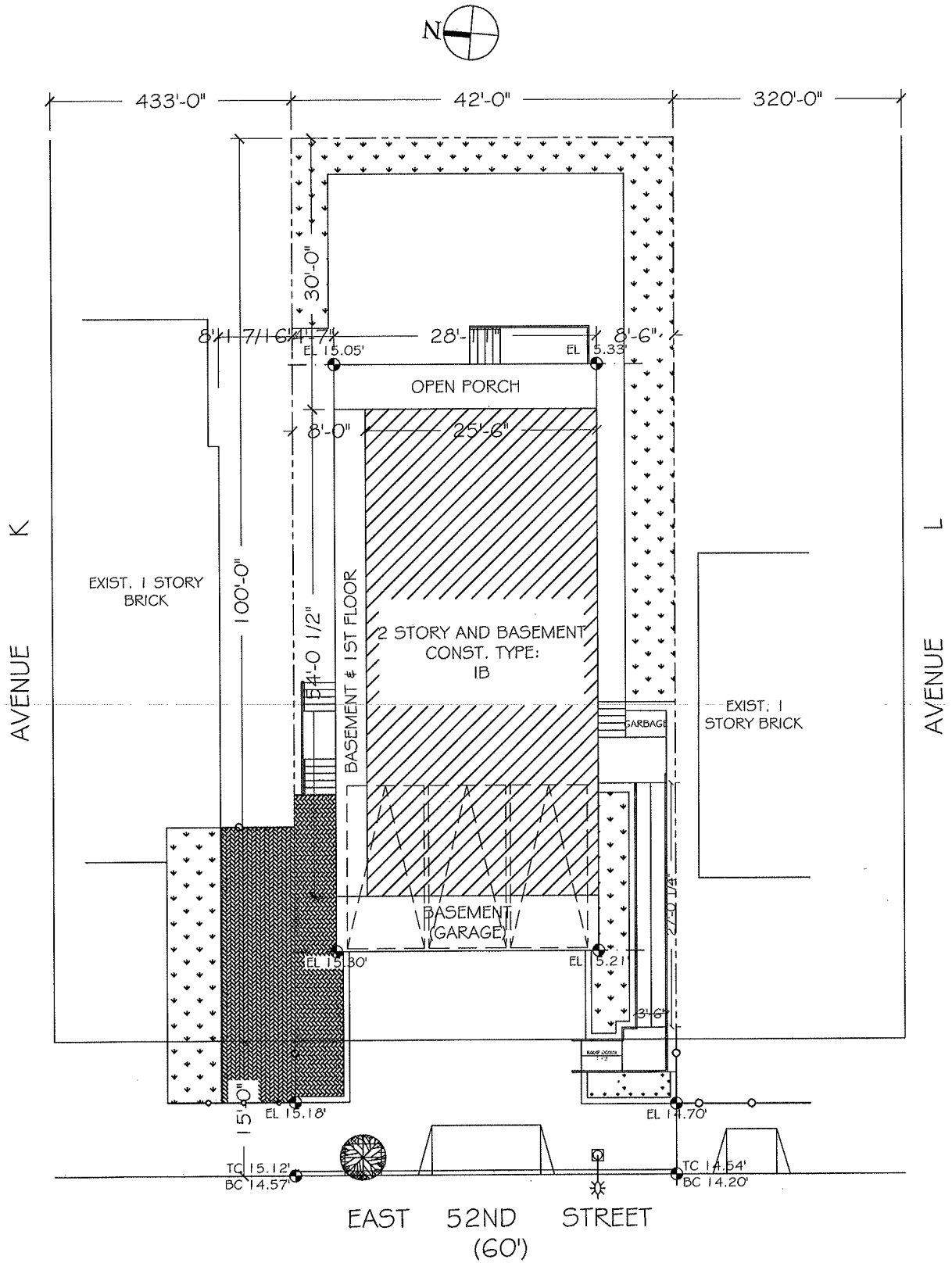
SITE PLAN
