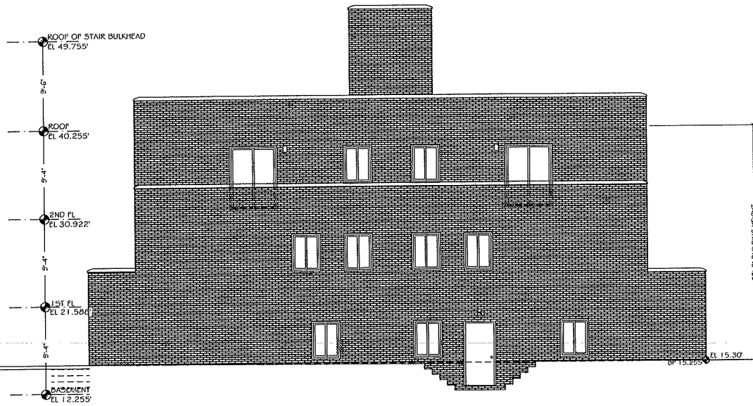
NORTH WALL ELEVATION
