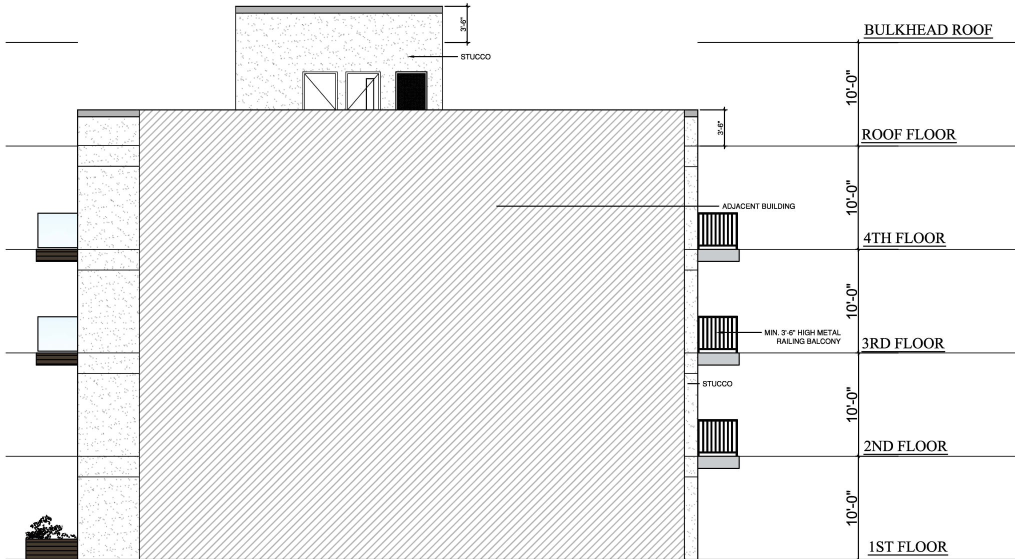
WEST ELEVATION
