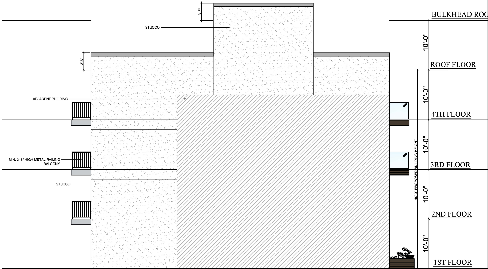
EAST ELEVATION
