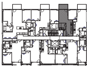
KEY PLAN 1/64" = 1'-0"
