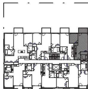
KEY PLAN 1/64" = 1'-0"
