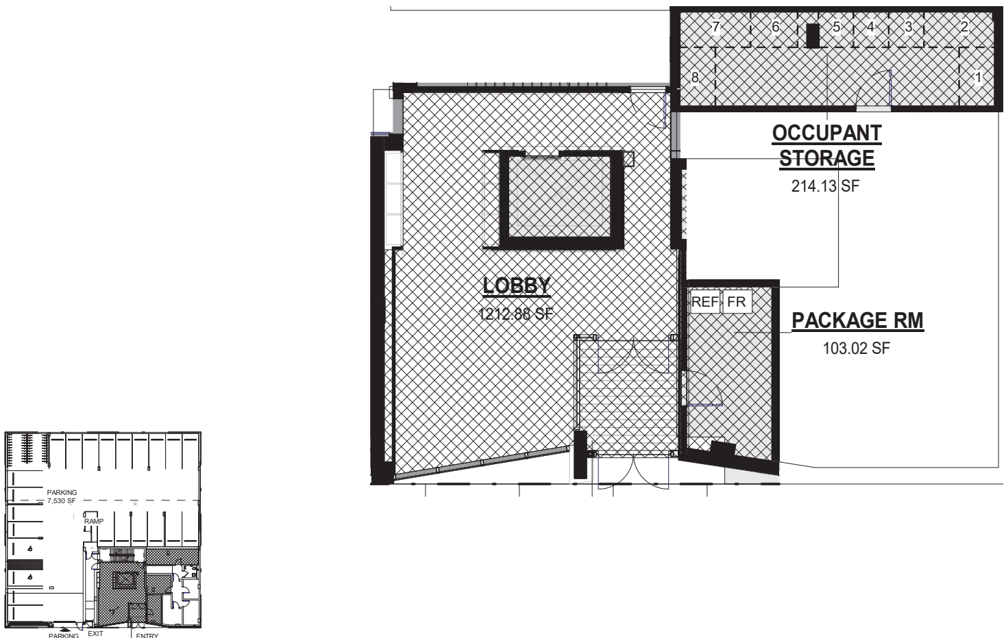
KEY PLAN 1/64" = 1'-0"
