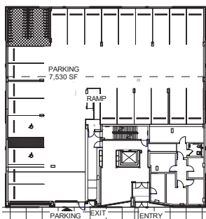
KEY PLAN 1/64" = 1'-0"
