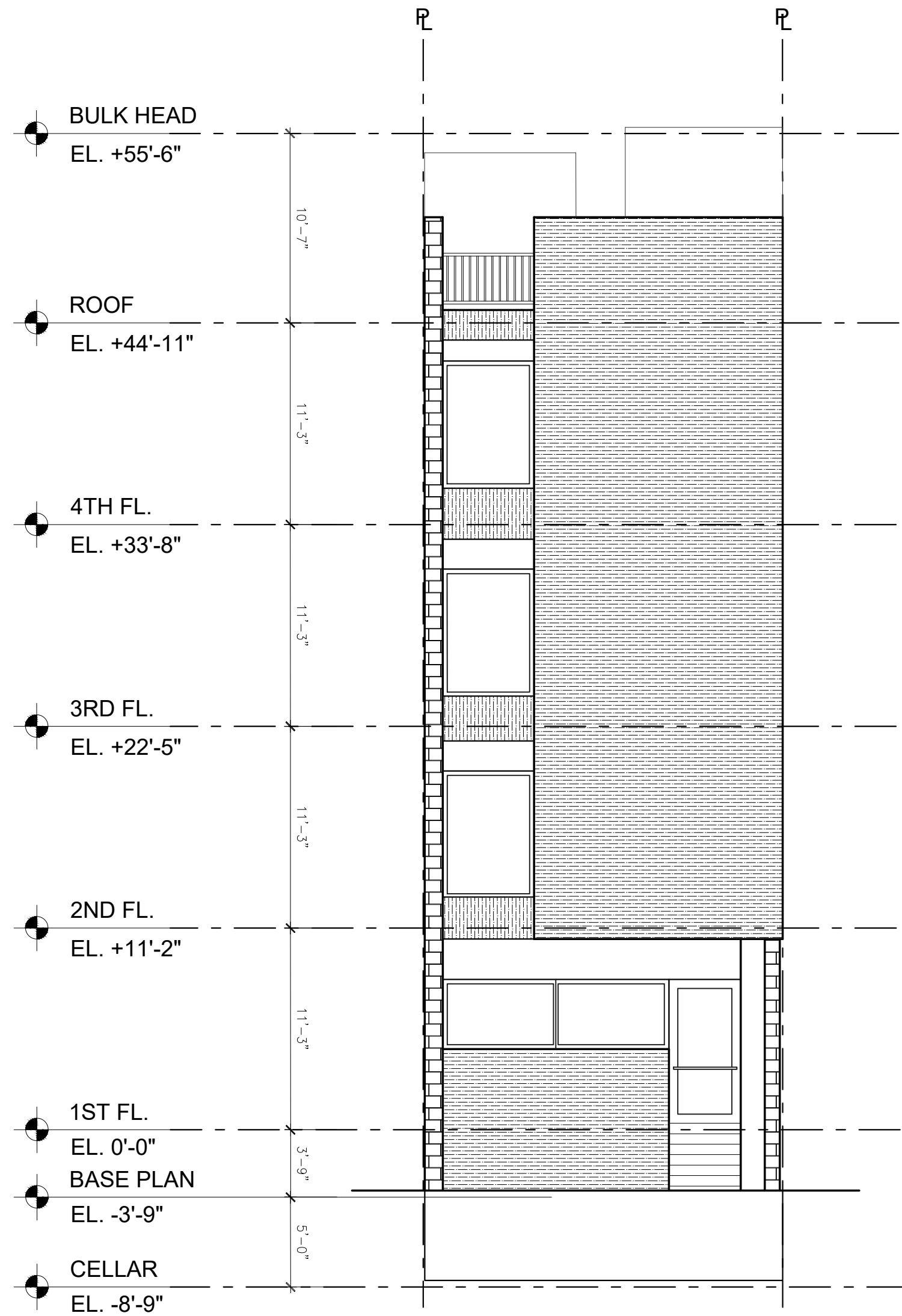
NORTH ELEVATION (34 STREET)
