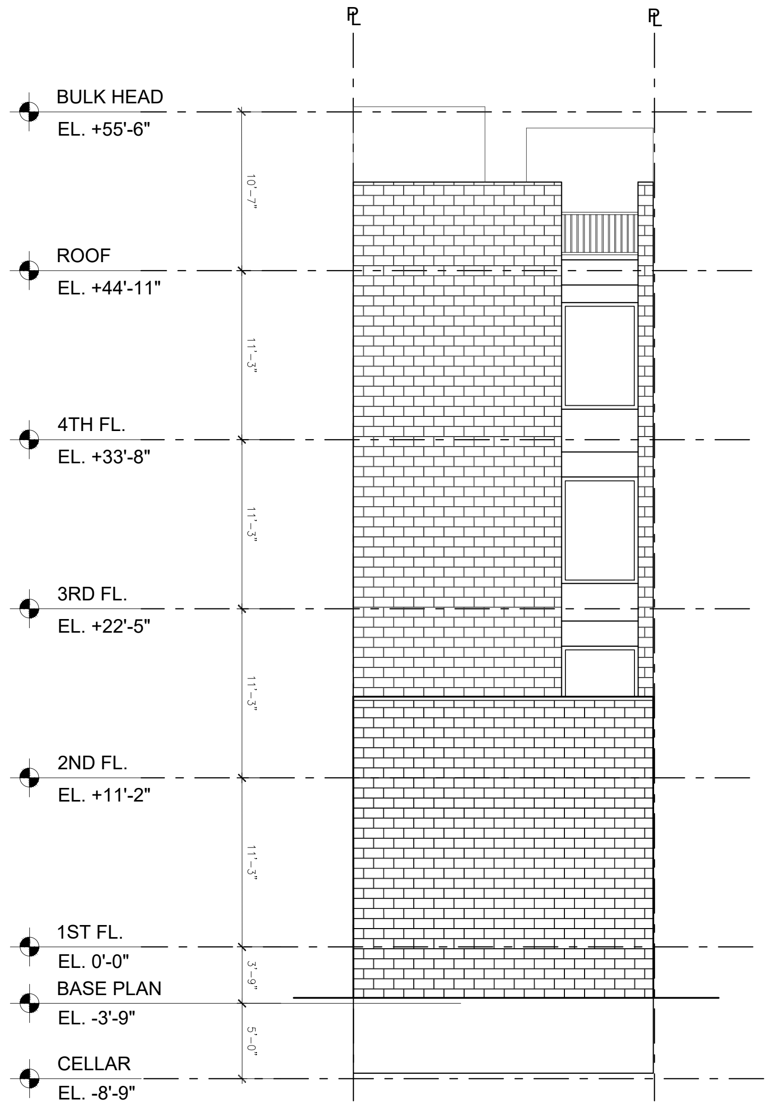
SOUTH ELEVATION
