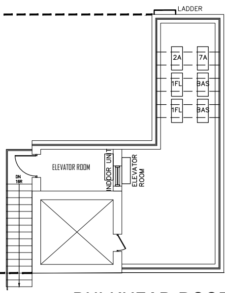
BULKHEAD ROOF SCALE: 3/32" = 1'-0"
