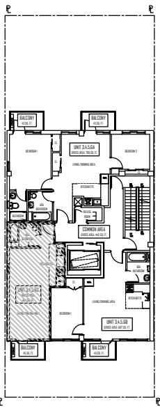
3RD THRU 6TH FL KEYPLAN
