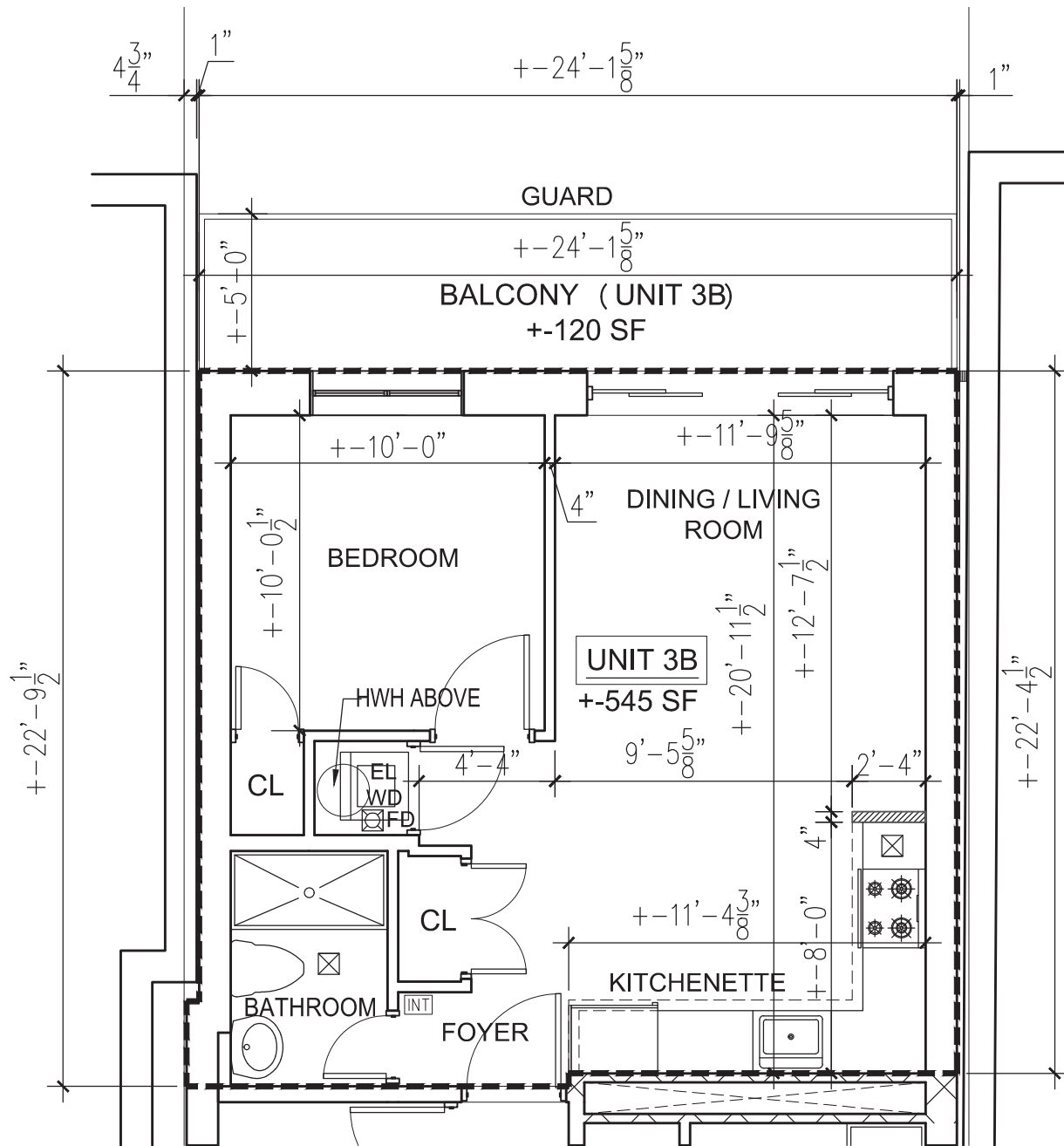
UNIT 3B. THIRD FLOOR SCALE: 3/16"=1'-0"
