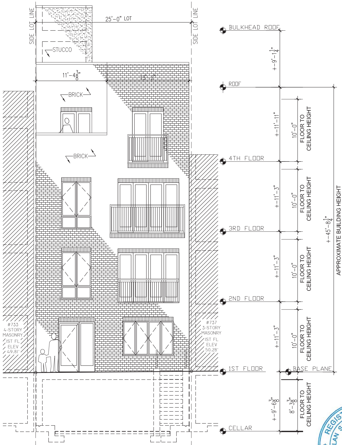
FRONT ELEVATION (SOUTH)
