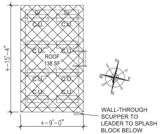
STAIR BULKHEAD ROOF PLAN
