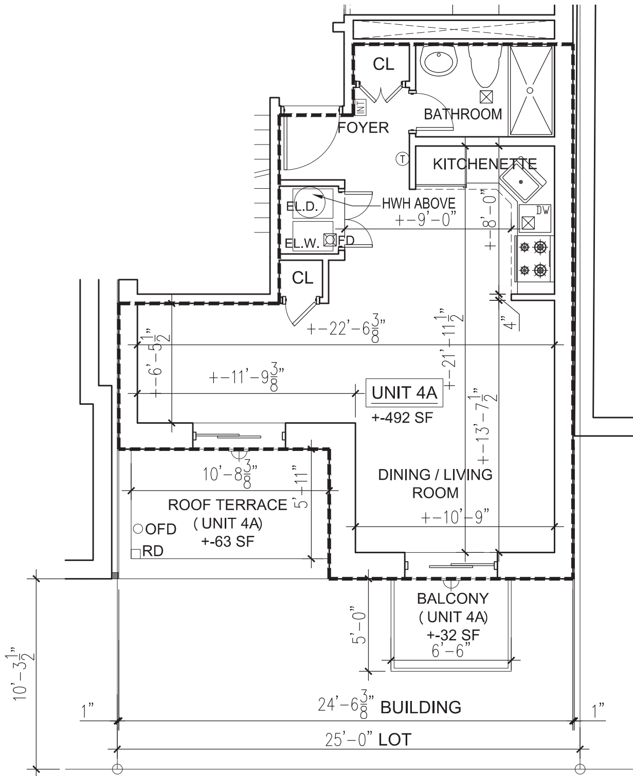
UNIT 4A. FOURTH FLOOR SCALE: 3/16"=1'-0"
