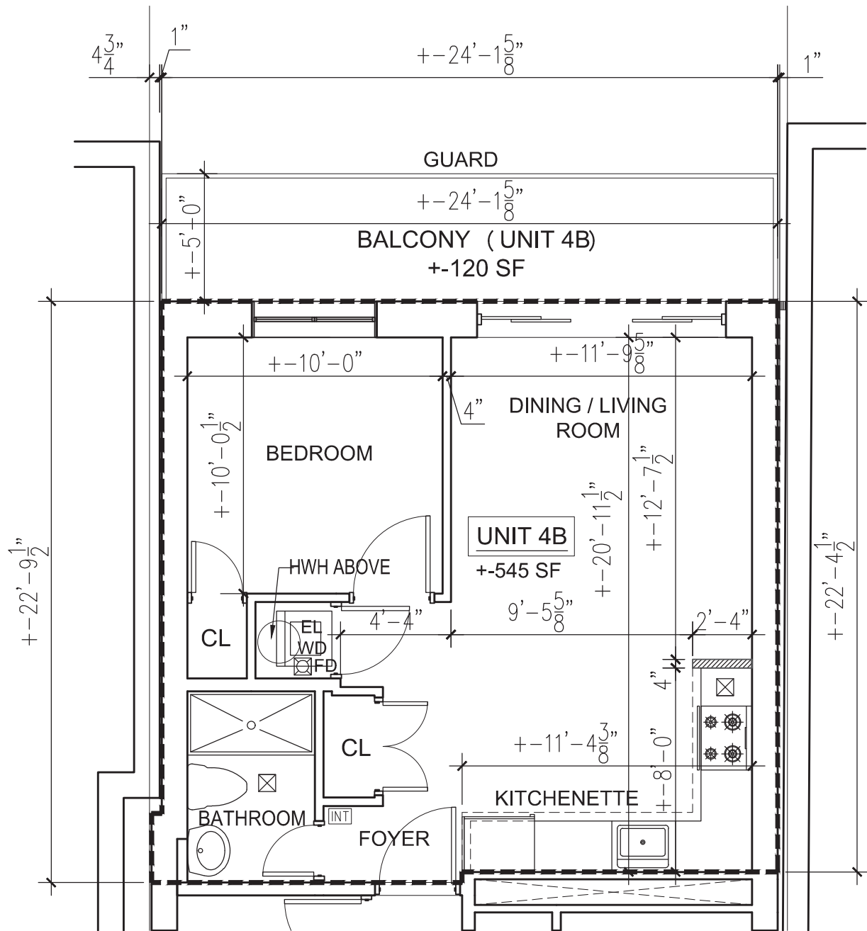
UNIT 4B. FOURTH FLOOR SCALE: 3/16"=1'-0"
