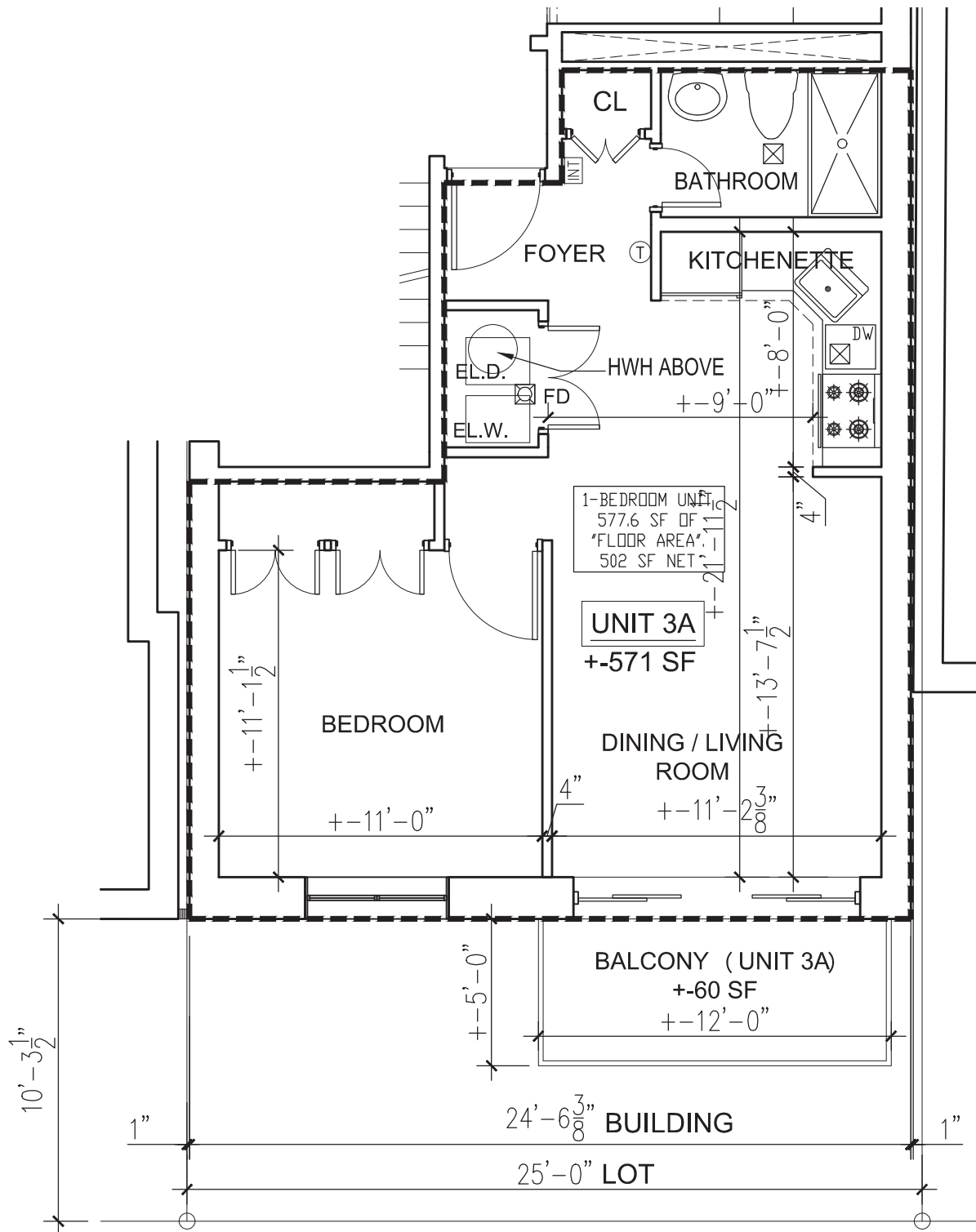
UNIT 3A. THIRD FLOOR SCALE: 3/16"=1'-0"
