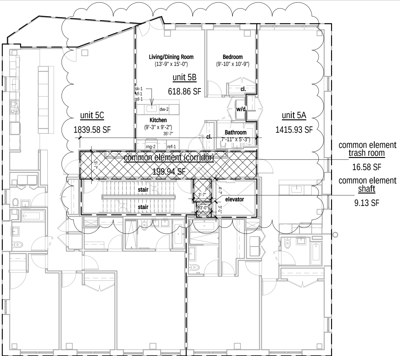
Fifth Floor Unit 5B Plan
