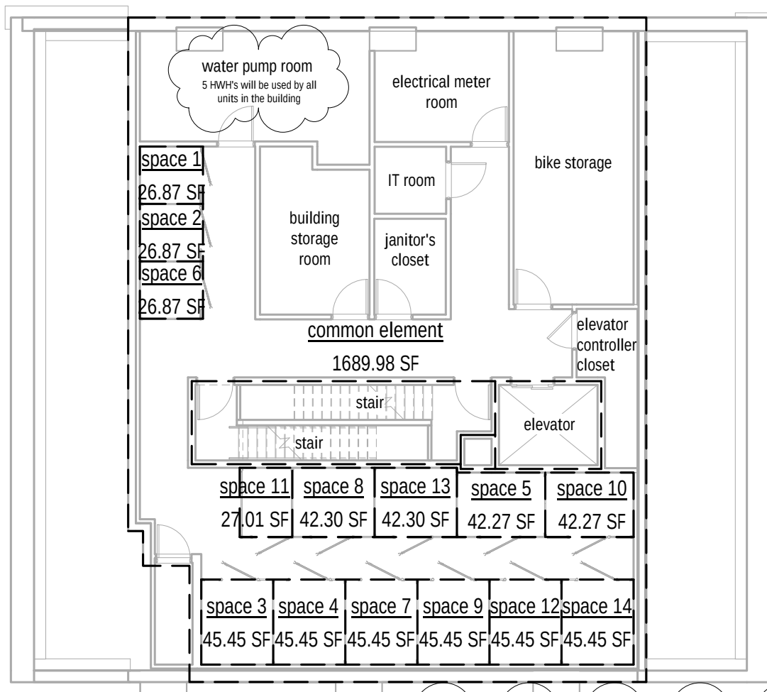
Cellar Floor Plan
