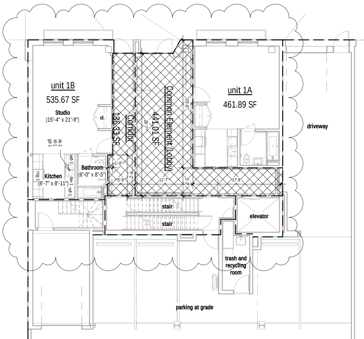
First Floor Plan - Unit 1B
