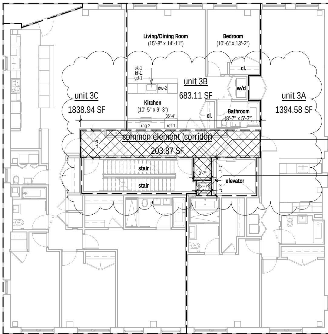
Third Floor Unit 3B Plan
