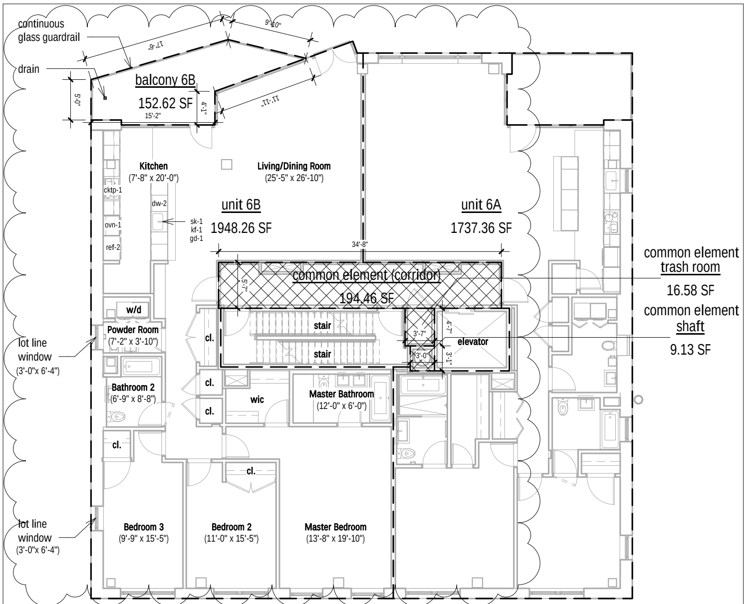
Sixth Floor Unit 6B Plan
