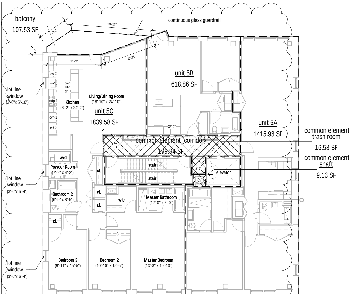
Fifth Floor Unit 5C Plan
