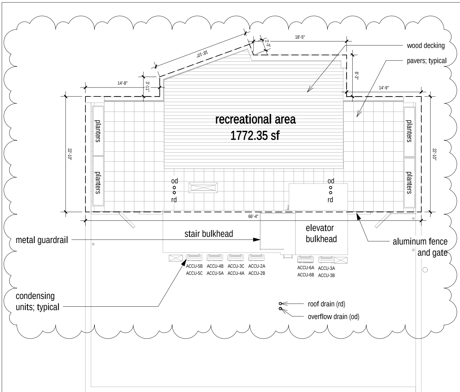
Roof and Bulkhead Plans
