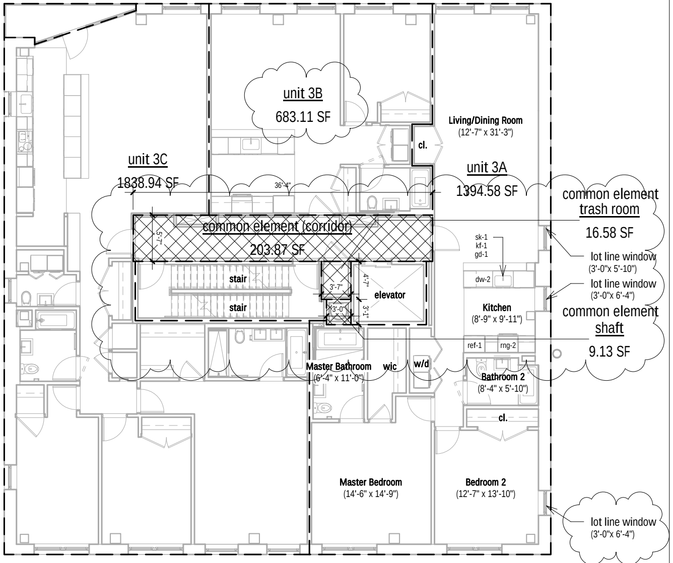
Third Floor Unit 3A Plan
