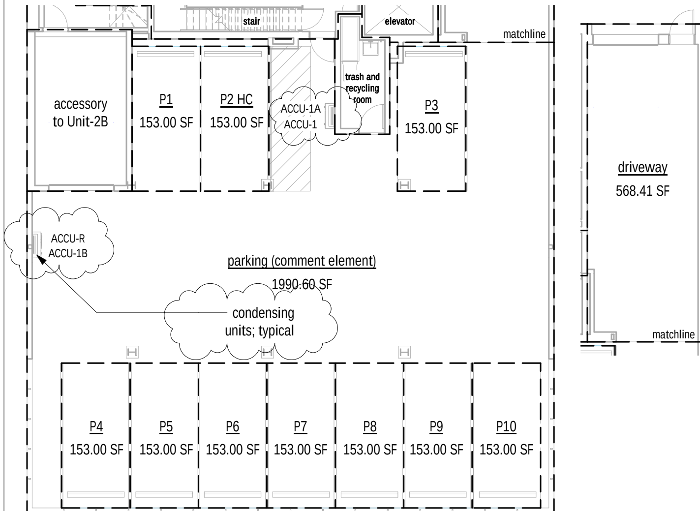
First Floor Plan - Parking
