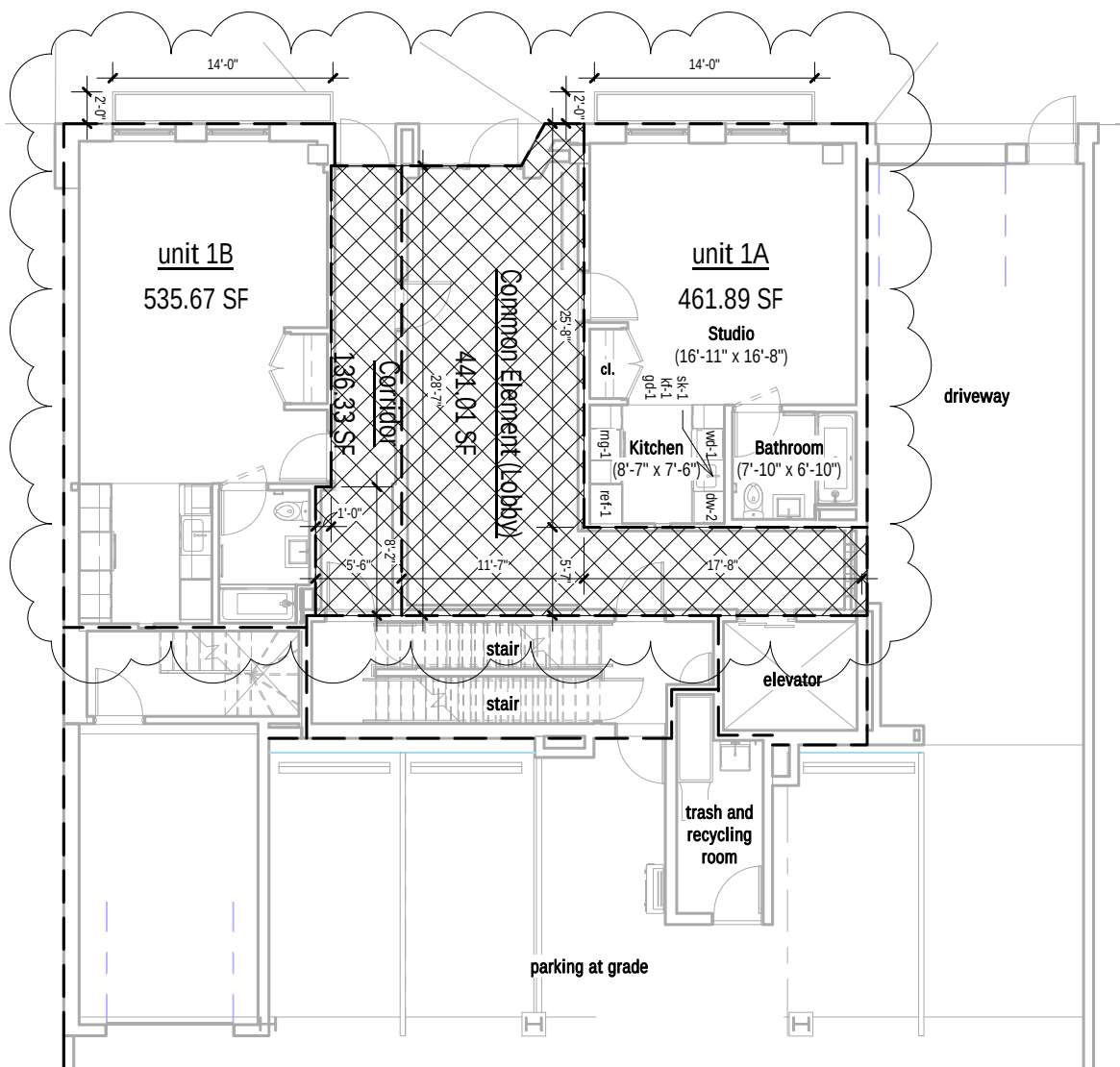
First Floor Plan - Unit 1A
