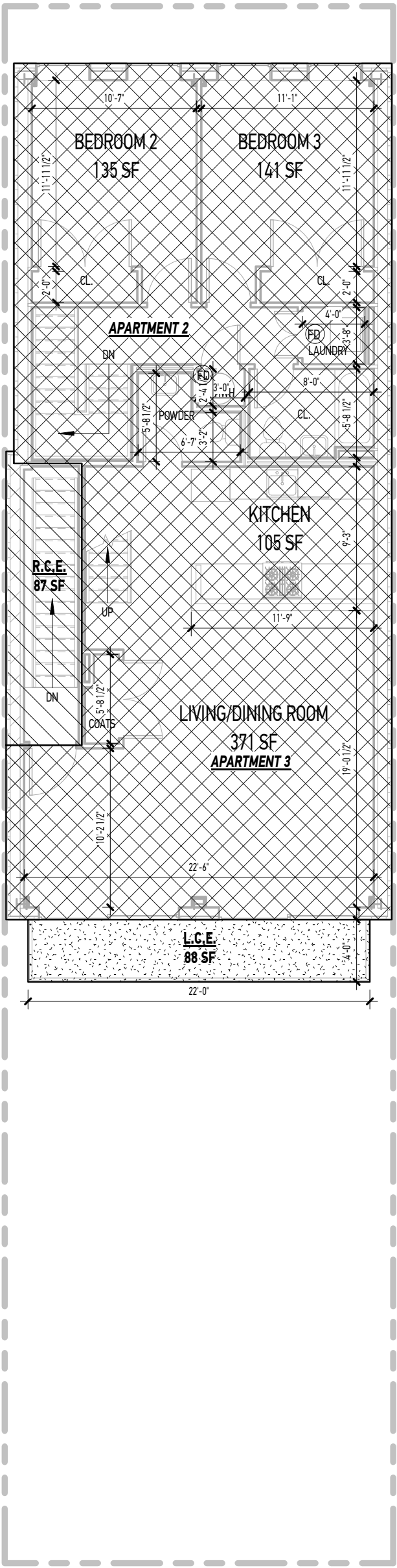
1 3RD FLOOR CONDOMINIUM PLAN 1/8" = 1'-0"
