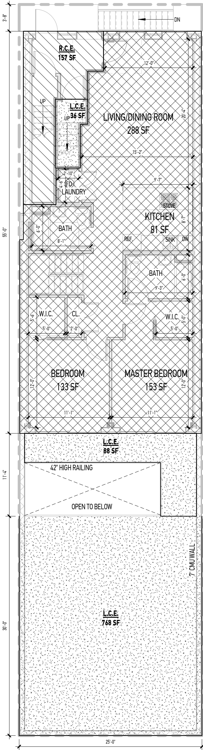
1 1ST FLOOR CONDOMINIUM PLAN 1/8" = 1'-0"
