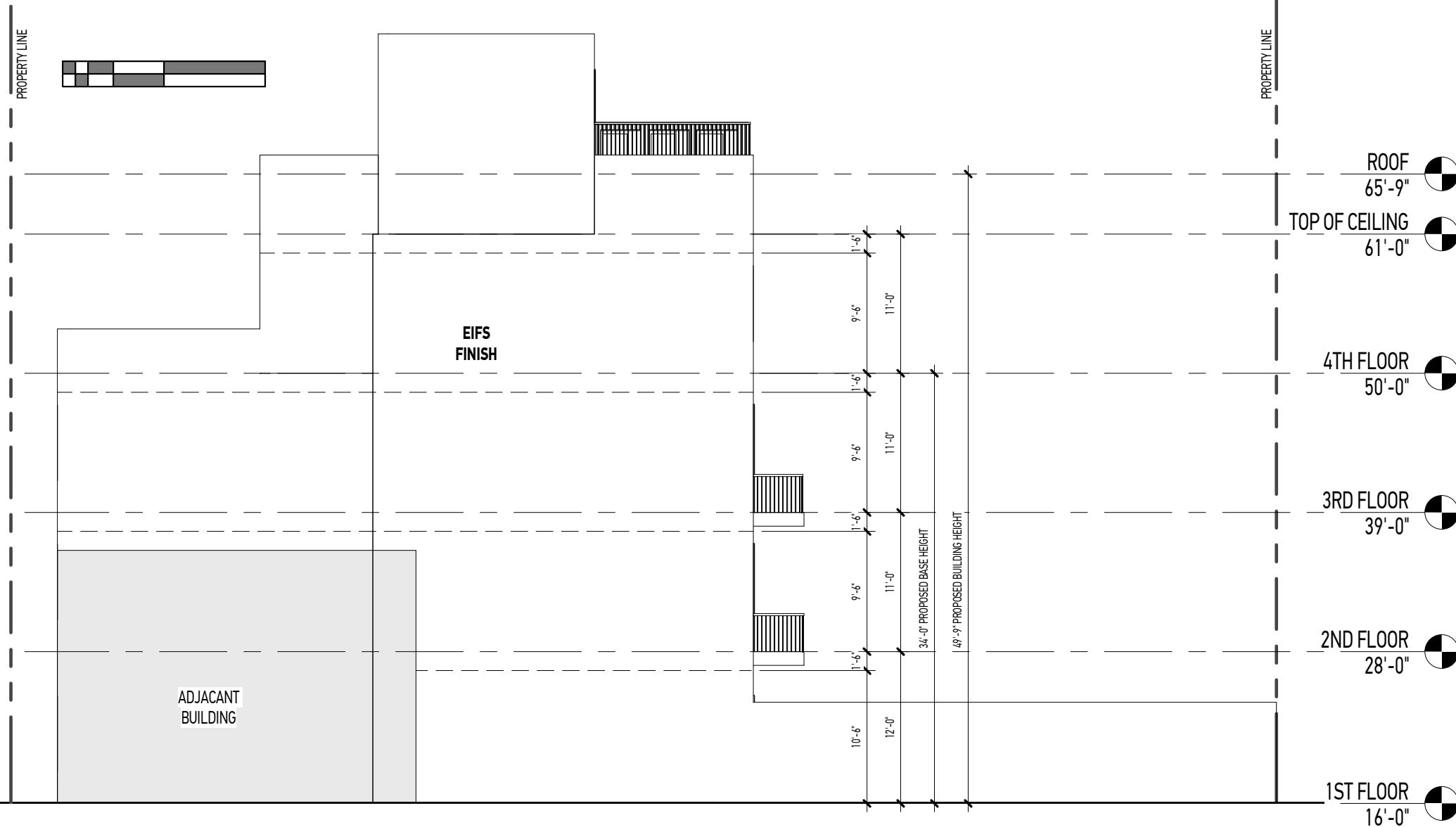
1 East Elevation 3/32" = 1'-0"
