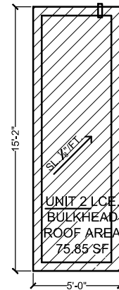
BULKHEAD ROOF PLAN
