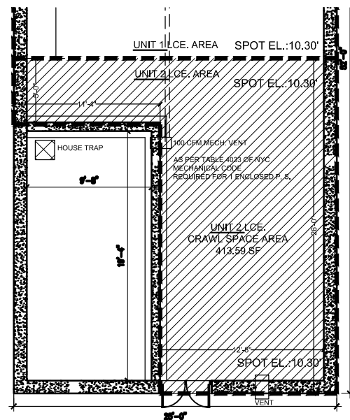
FOOTING & FOUNDATION PLAN
