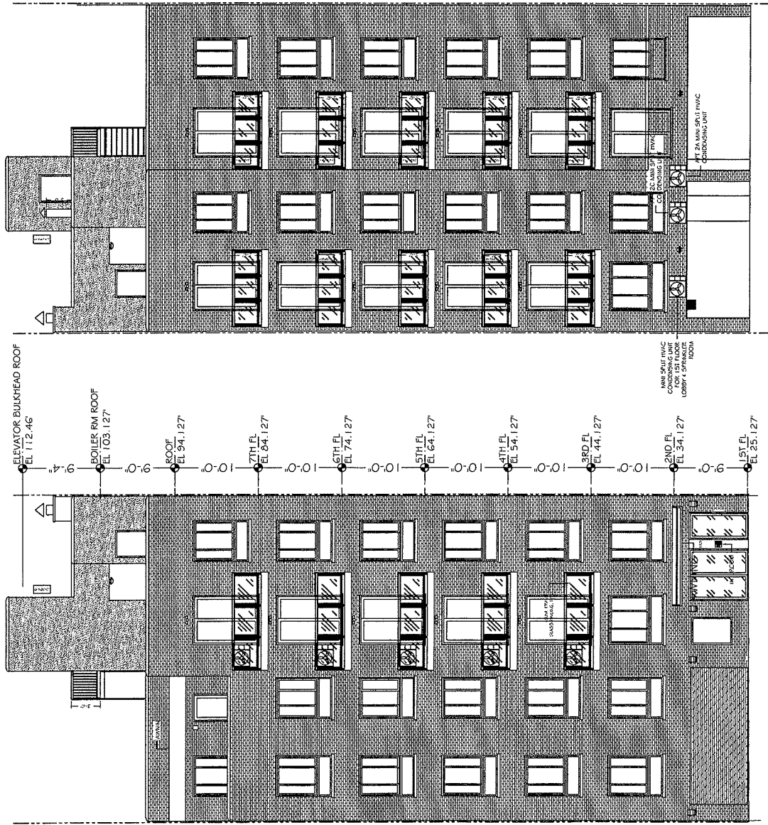
REAR ELEVATION
