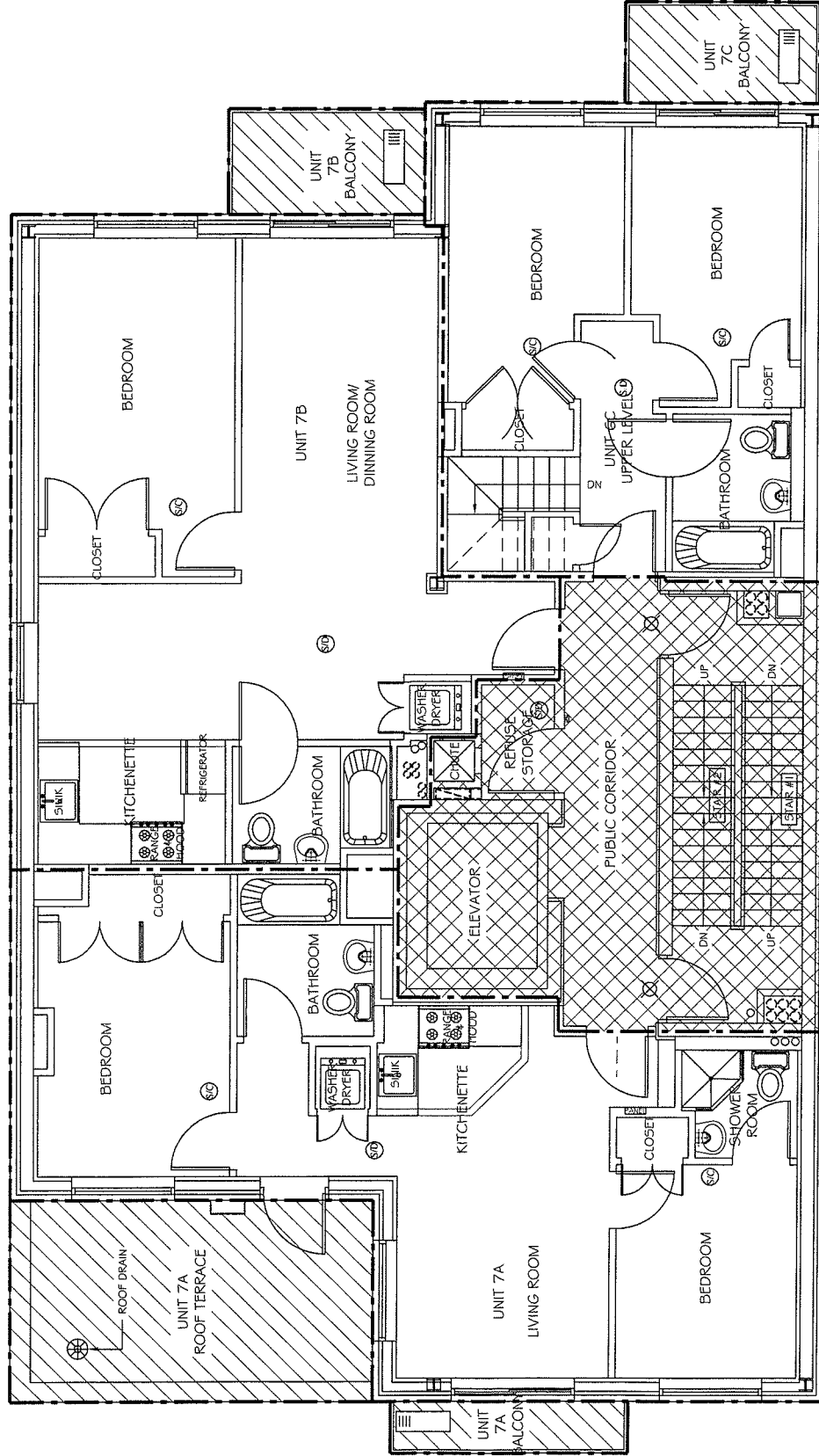
SEVENTH FLOOR KEY PLAN
