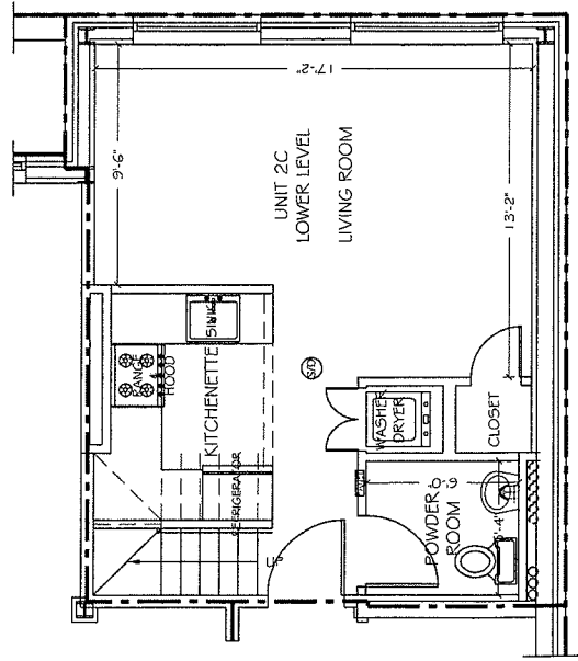
SECOND FLOOR-UNIT 2C LOWER LEVEL
