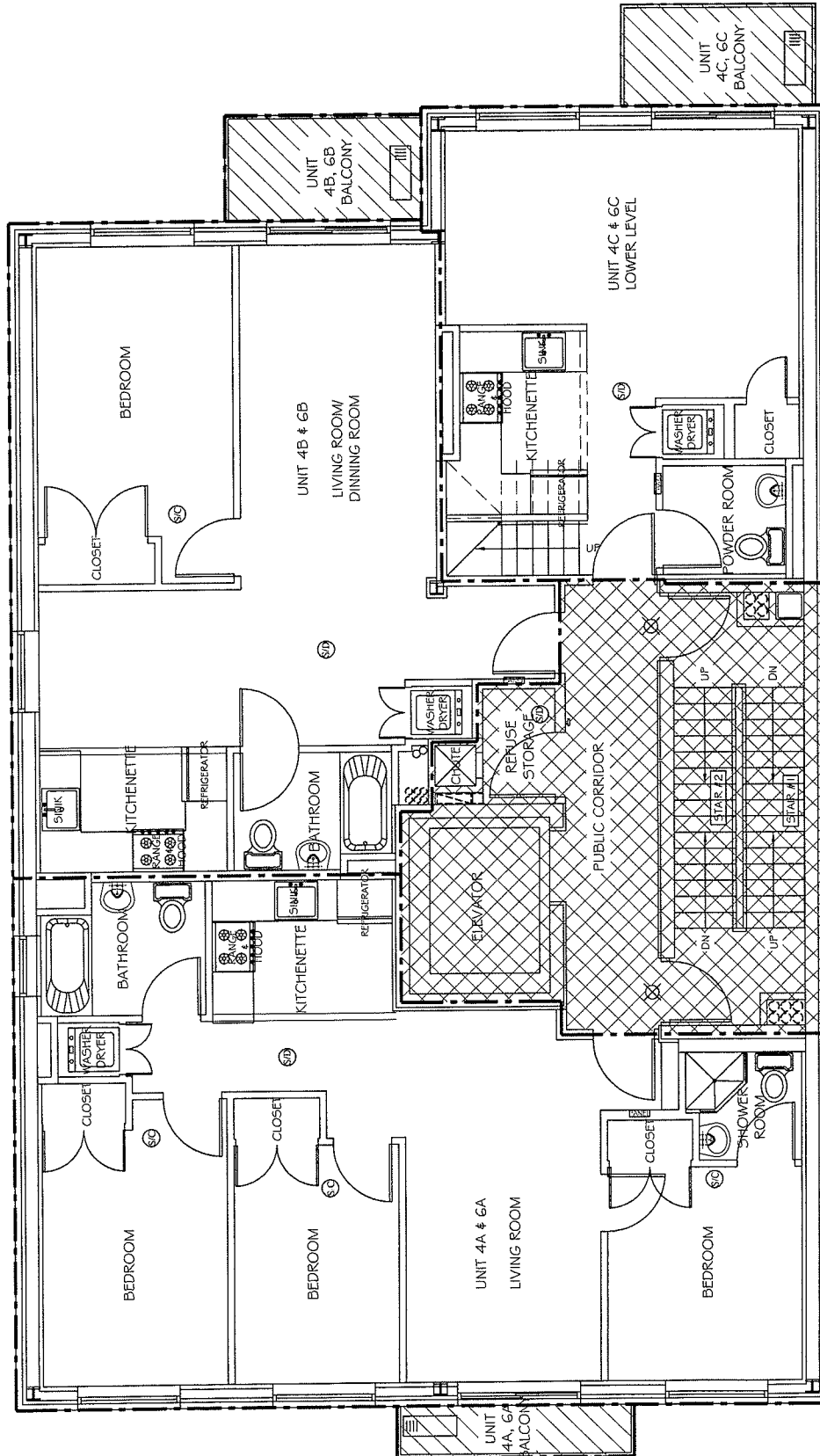
FOURTH & SIXTH FLOOR KEY PLAN
