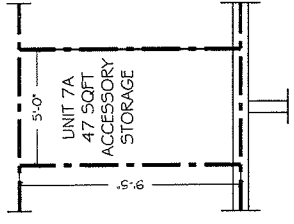
CELLAR FLOOR-UNIT 7A AREA: 47 SQFT
