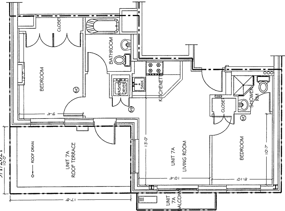
SEVENTH FLOOR-UNIT 7A AREA: 714 SQFT ROOF TERRACE: 177 SQFT BALCONY: 29 SQFT
