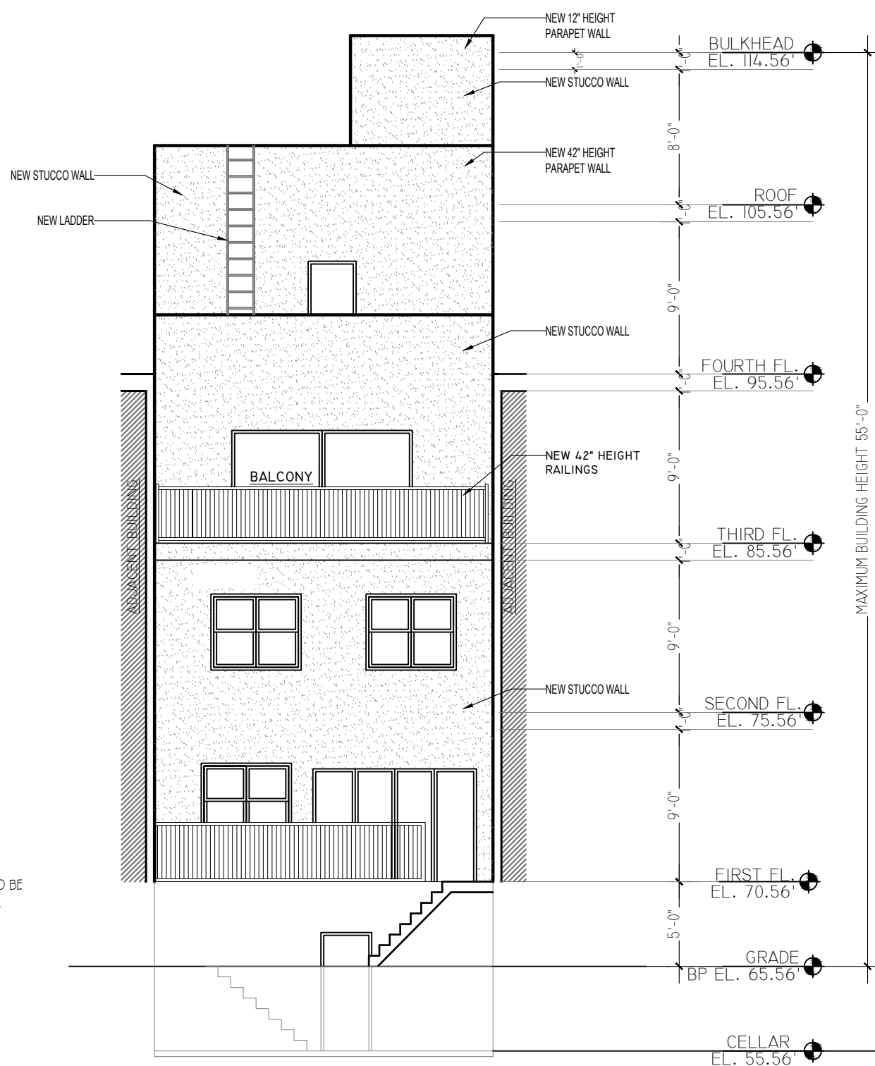
REAR ELEVATION
