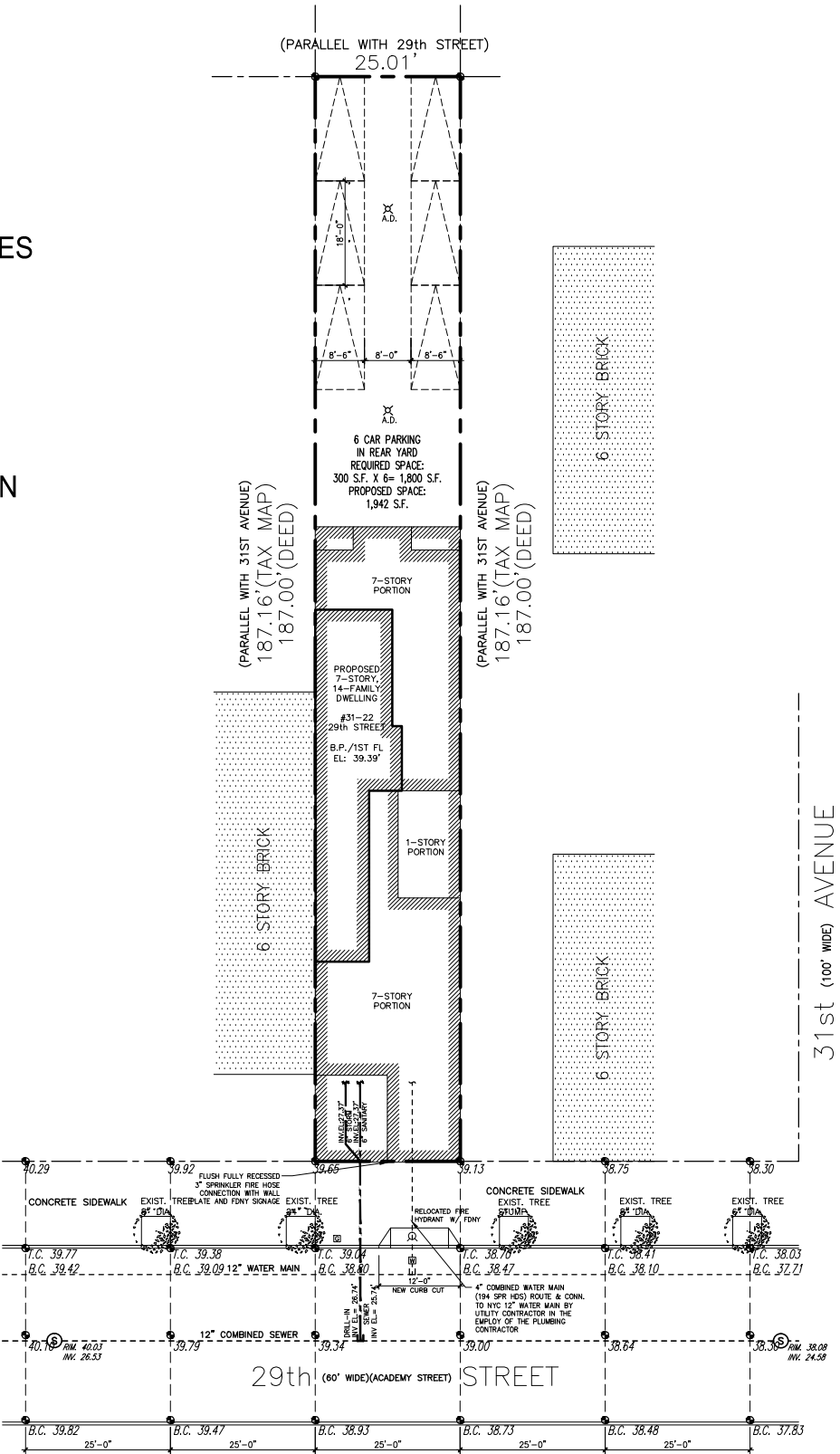
PLOT PLAN SCALE: 1"=30'-0"
