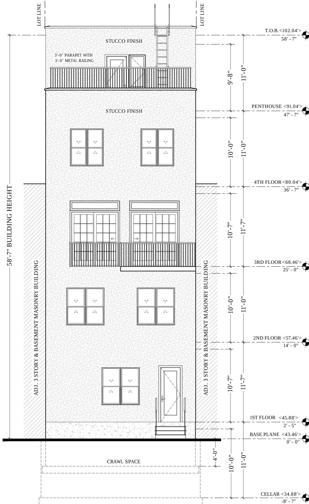
REAR ELEVATION SCALE 1/8" = 1'-0"
