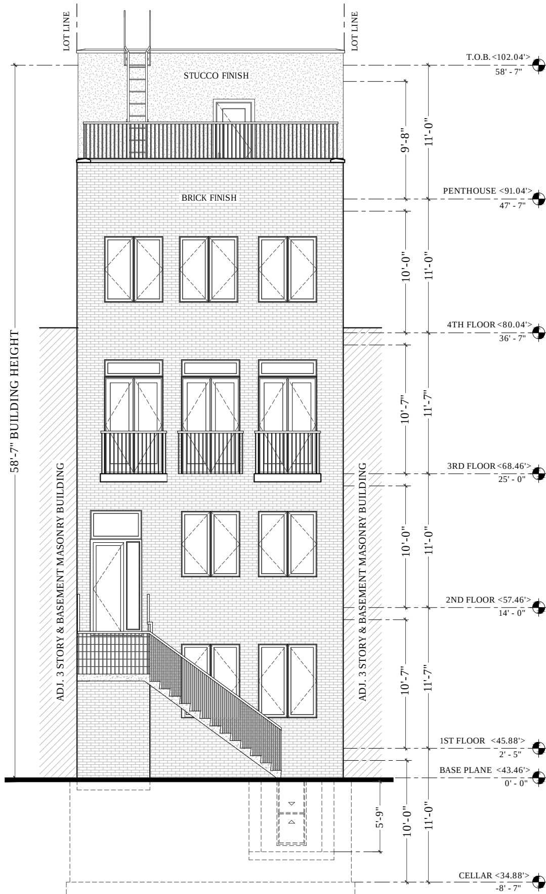
FRONT ELEVATION SCALE 1/8" = 1'-0"
