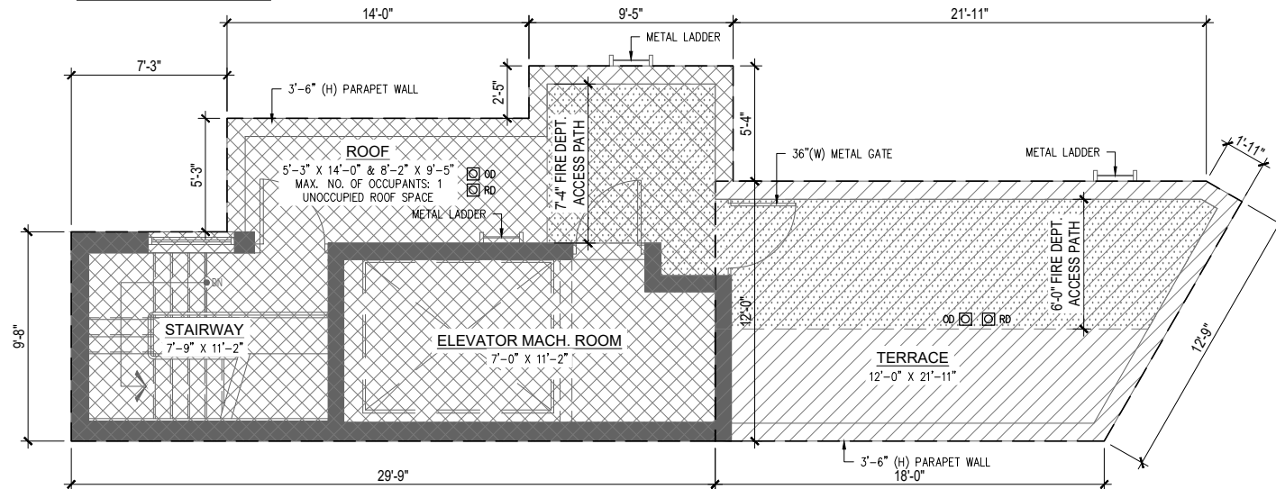
BULKHEAD ROOF
