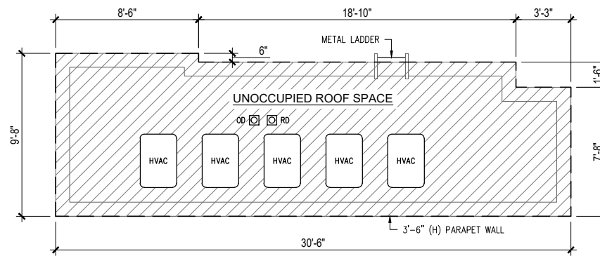
BULKHEAD ROOF
