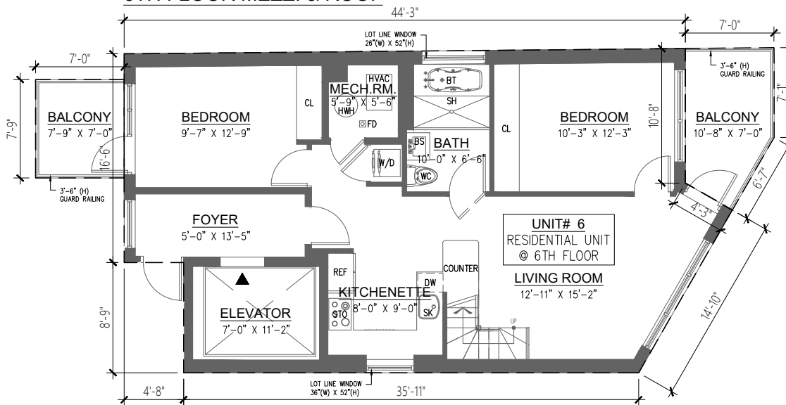
6TH FLOOR
