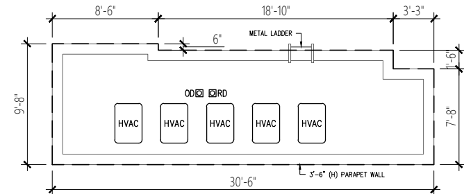
BULKHEAD ROOF
