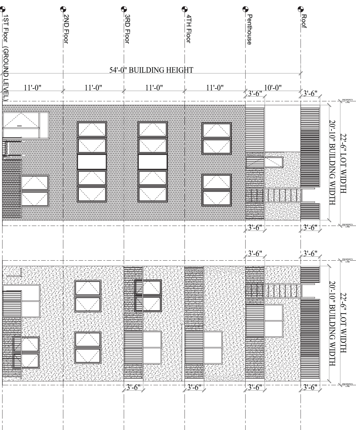
FRONT ELEVATION
