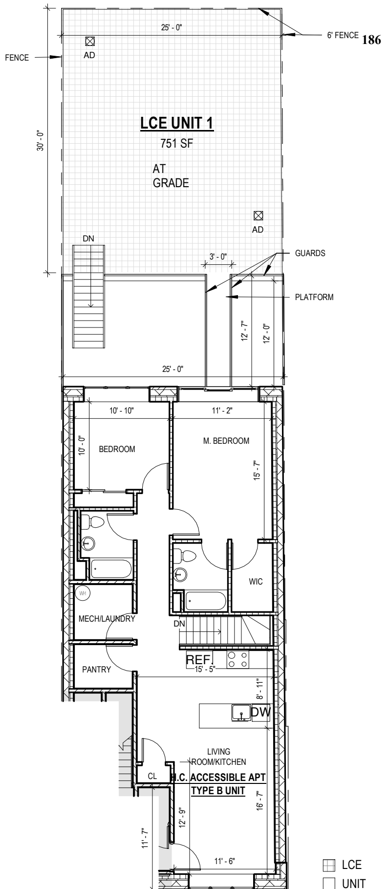
2 UNIT 1 - UPPER 3/32" = 1'-0"
