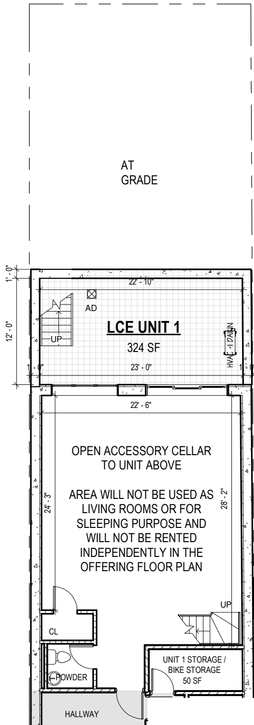
1 UNIT 1 - LOWER 3/32" = 1'-0"
