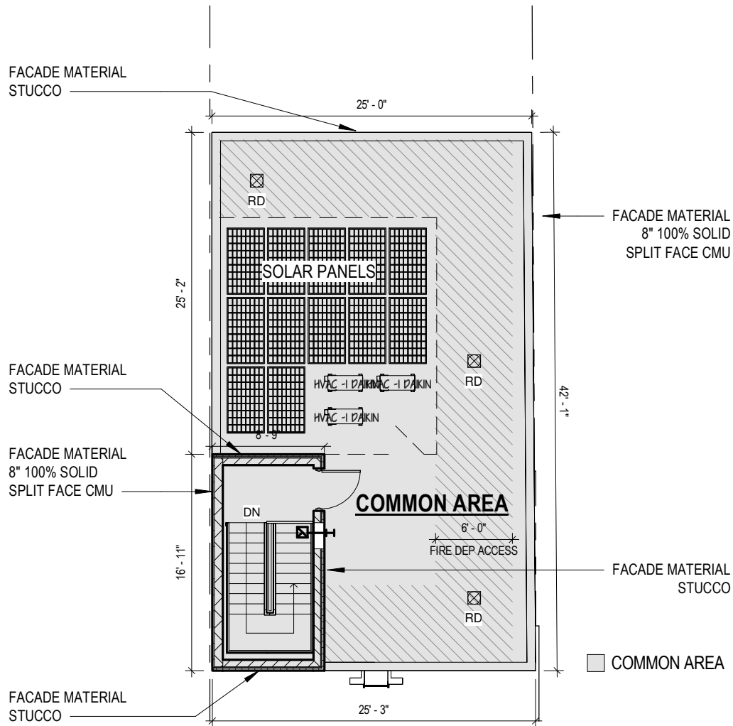
1 ROOF 3/32" = 1'-0"
