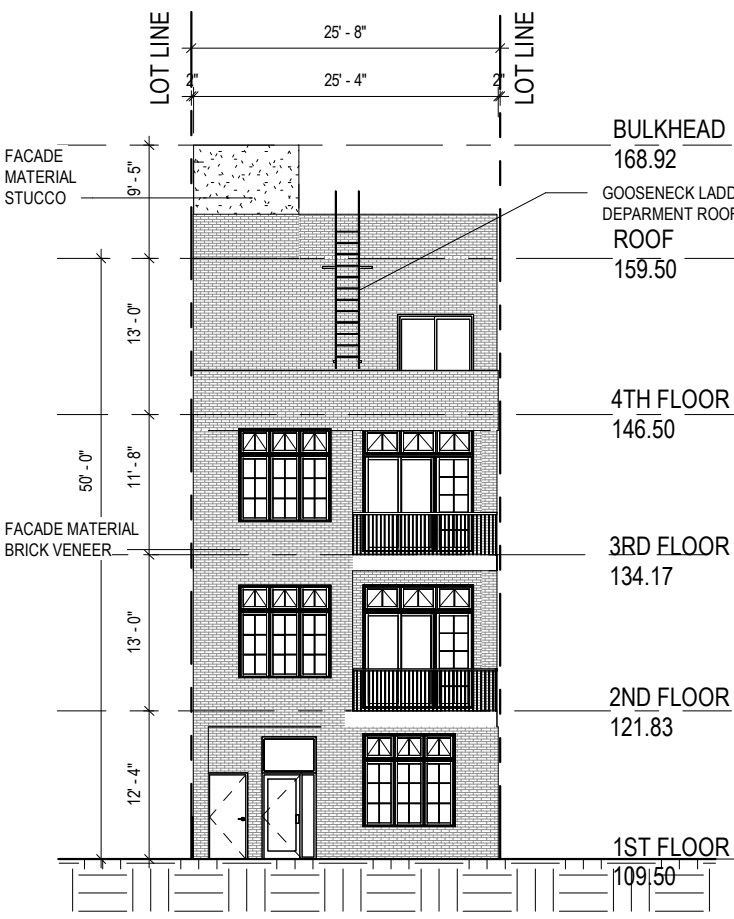
1 FRONT SOUTH ELEVATION 1/16" = 1'-0"
