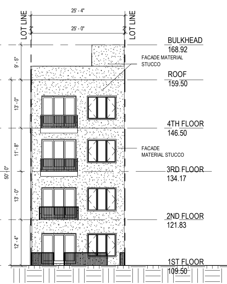
2 REAR NORTH ELEVATION 1/16" = 1'-0"
