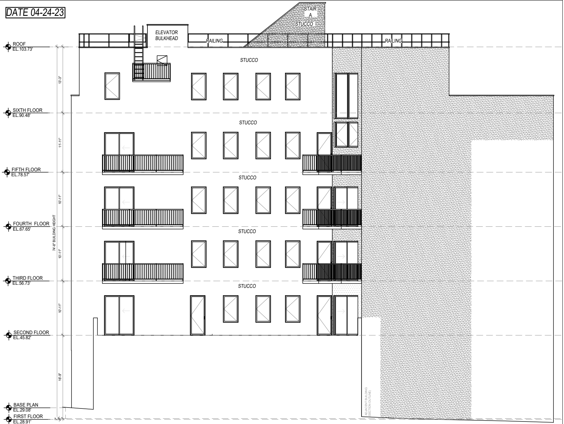
A10 REAR ELEVATION
