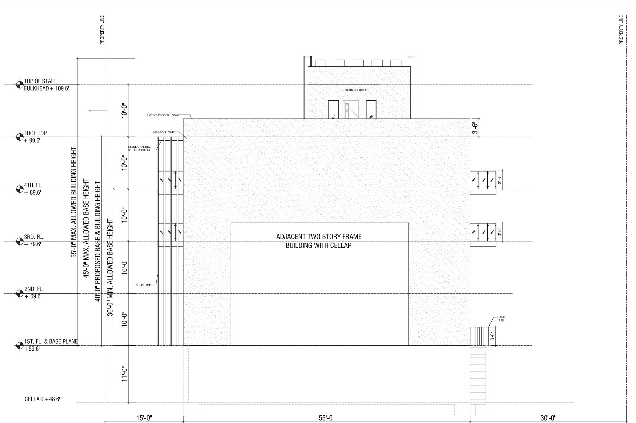
EAST SIDE ELEVATION
