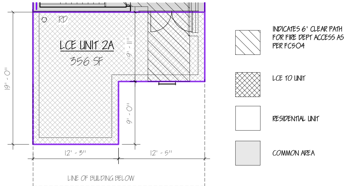
1 UNIT 2A - ROOF 1/8" = 1'-0"
