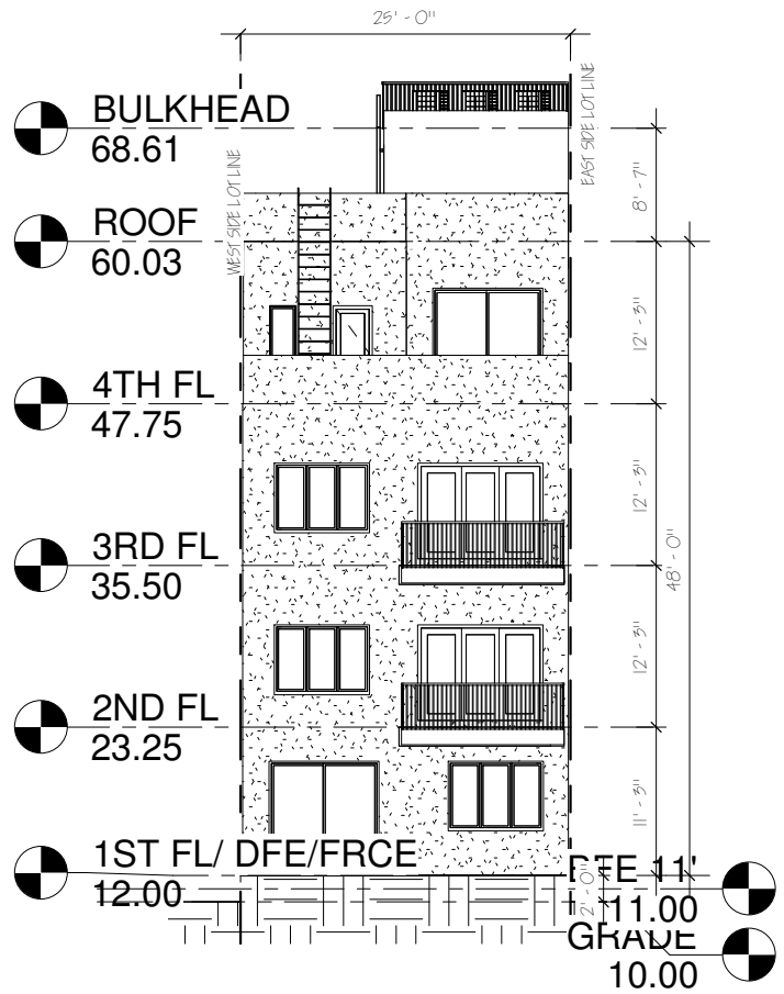
② CONDO - REAR (SOUTH) ELEVATION 1/16" = 1'-0"
