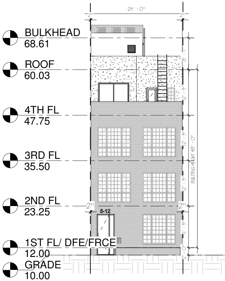
④ CONDO- FRONT (NORTH) ELEVATION 1/16" = 1'-0"
