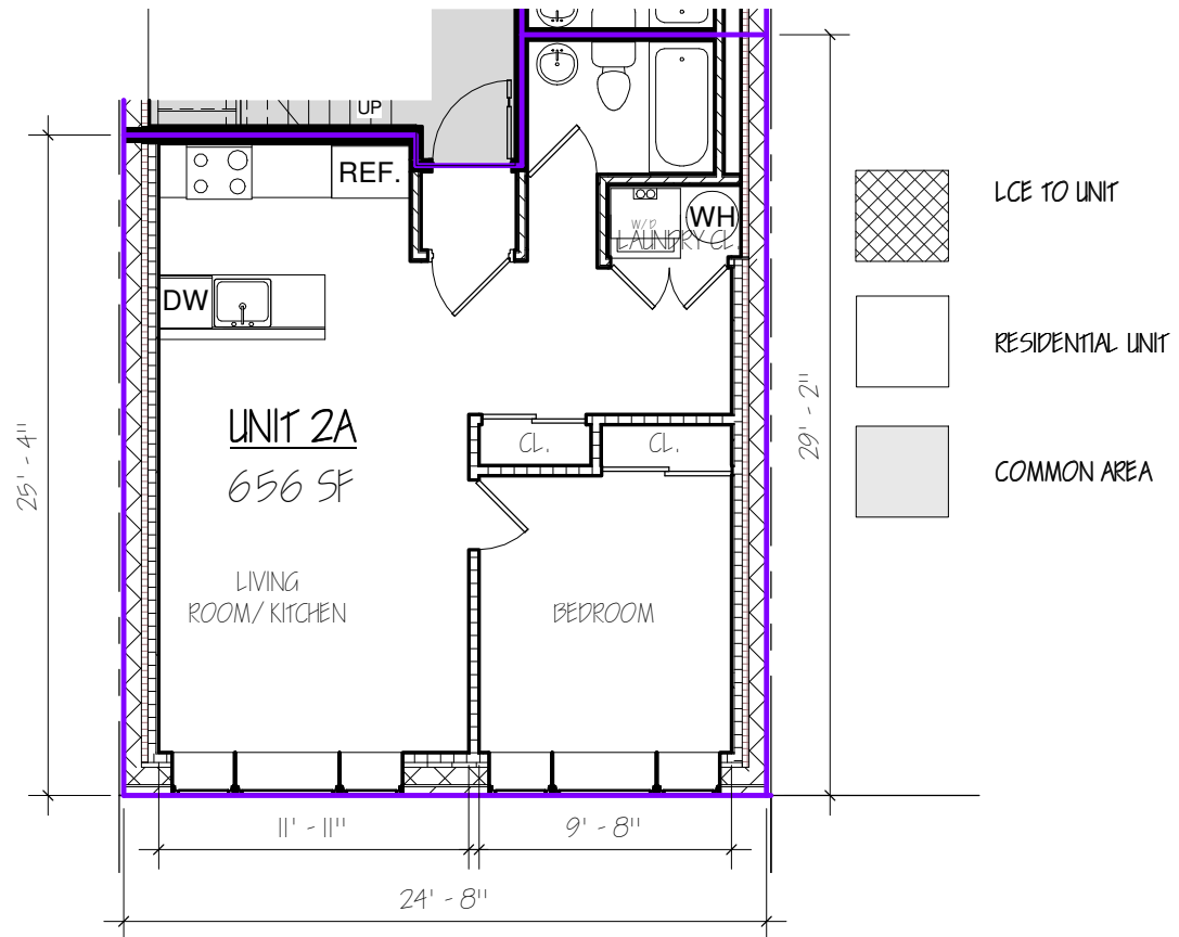
3 UNIT 2A - SECOND FL. 1/8" = 1'-0"
