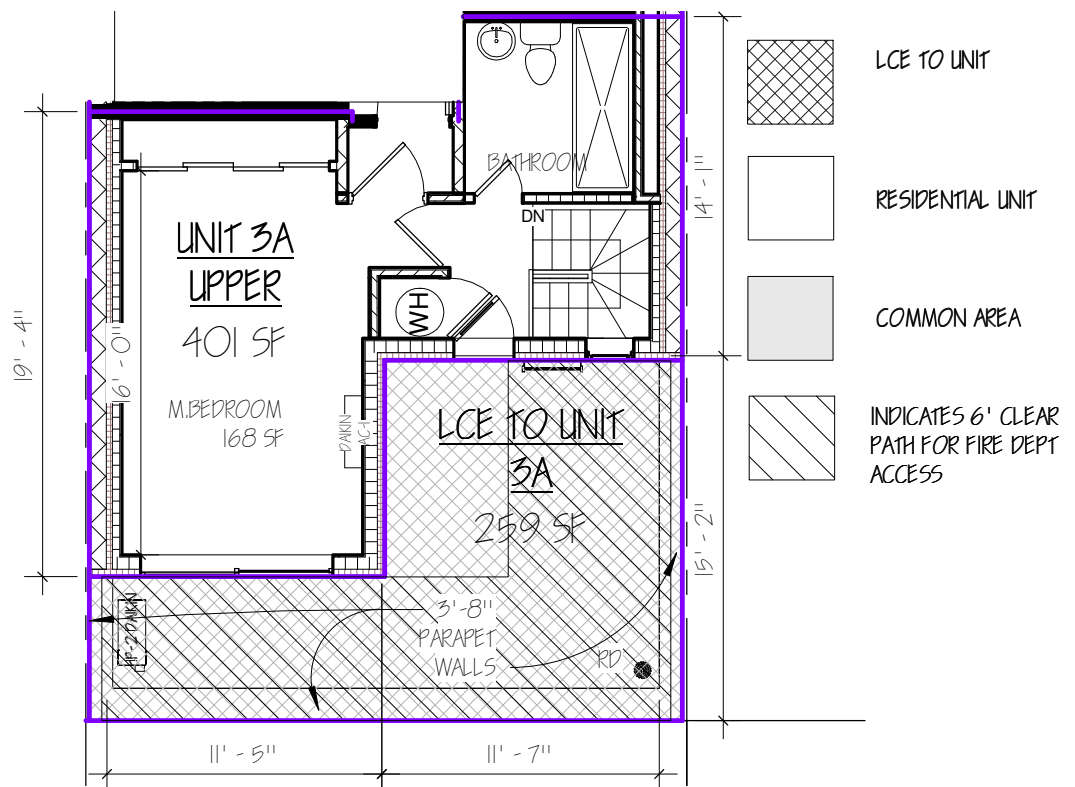
② UNIT 3A - FOURTH FLOOR 1/8" = 1'-0"
