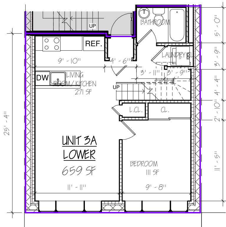
① UNIT 3A - THIRD FLOOR 1/8" = 1'-0"
