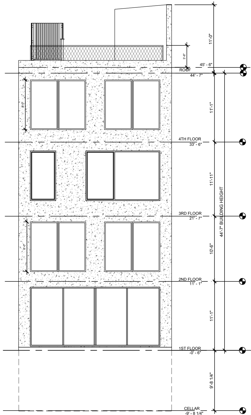
REAR ELEVATION
