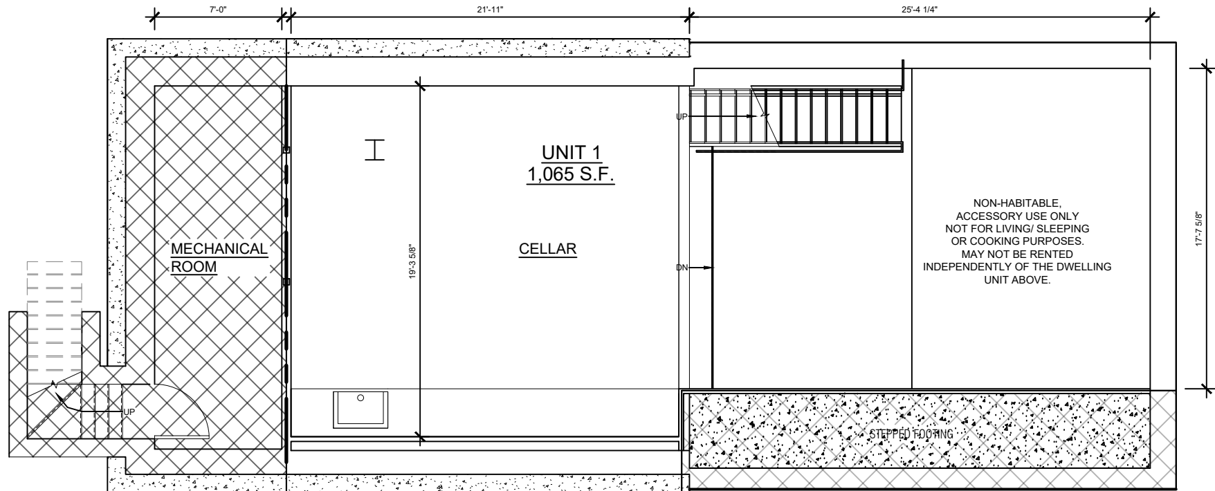
CELLAR FLOOR PLAN
