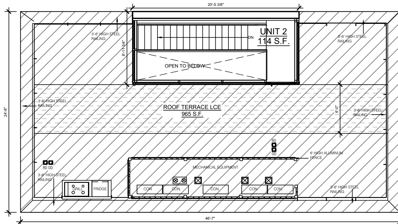
ROOF FLOOR PLAN
