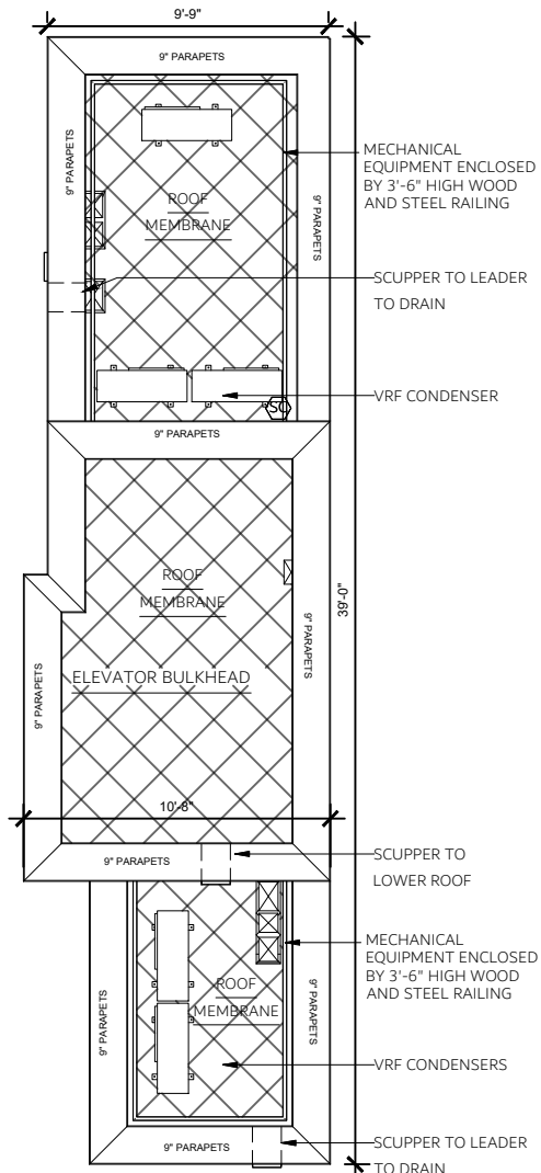
BULKHEAD FLOOR PLAN
