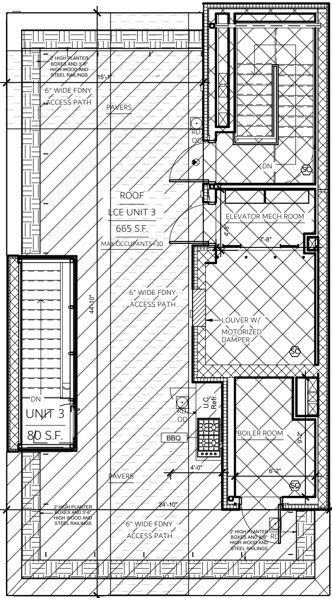
ROOF FLOOR PLAN
