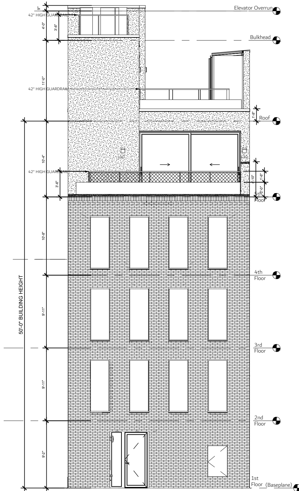
FRONT ELEVATION
