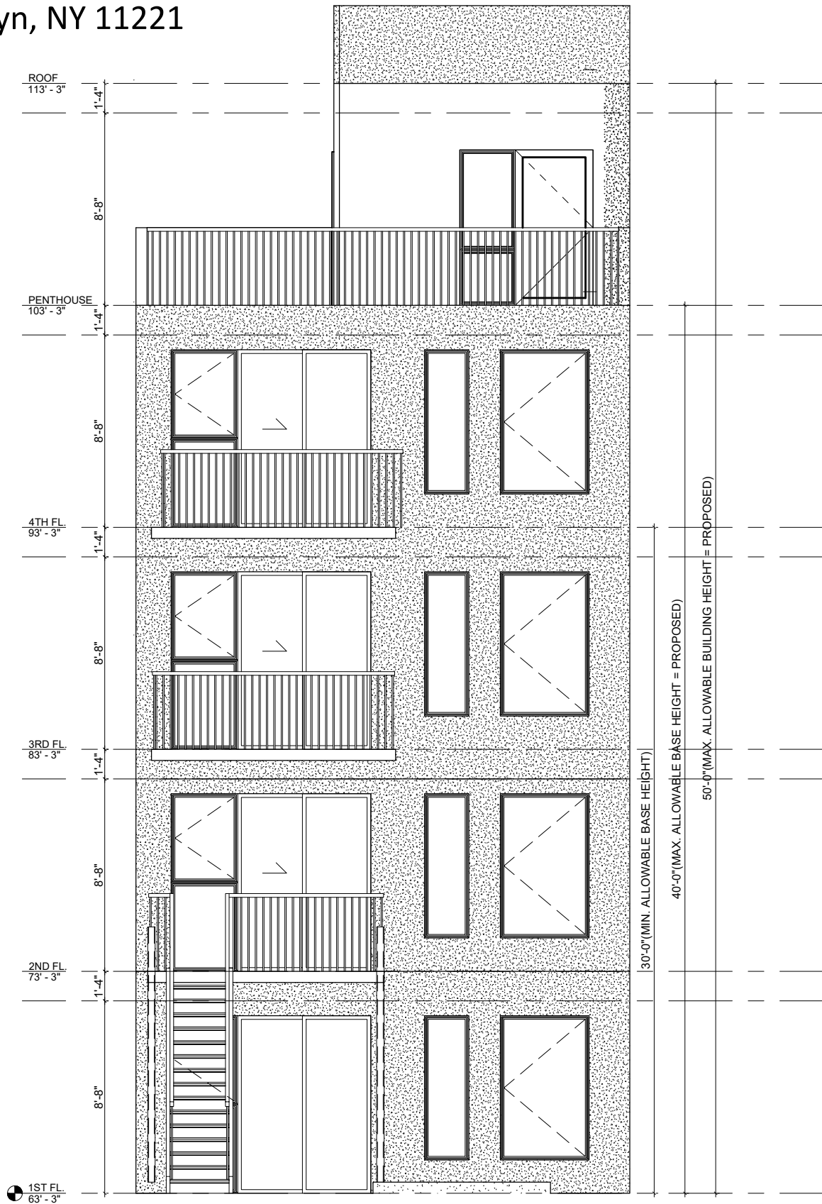
REAR ELEVATION PLAN
