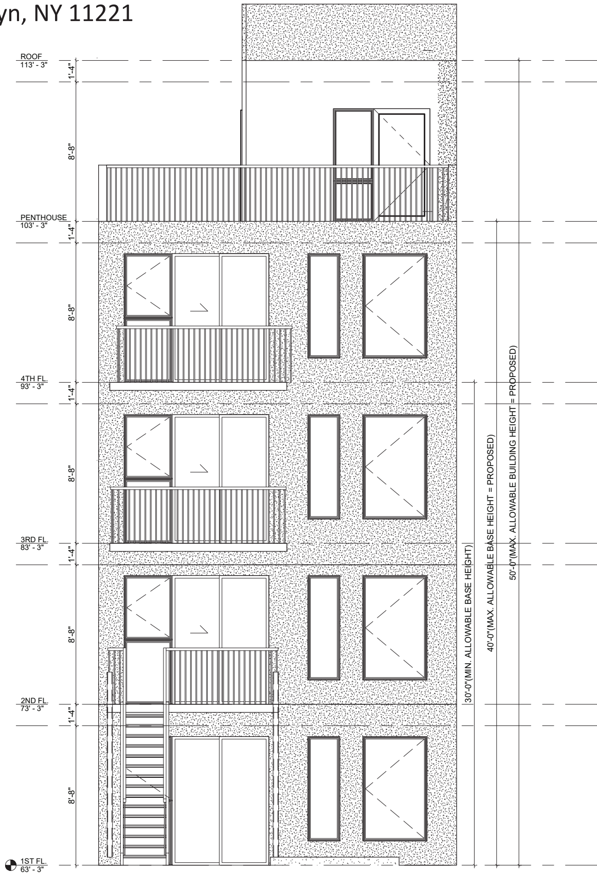
REAR ELEVATION PLAN
