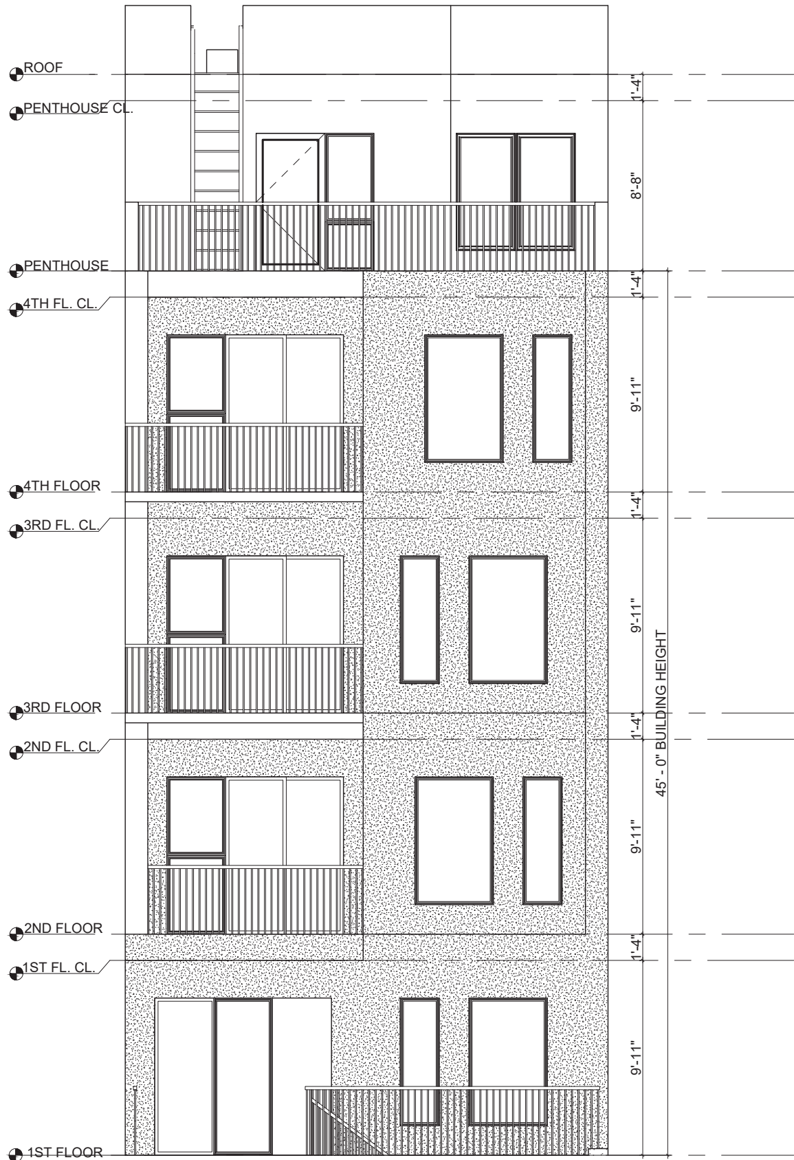
REAR ELEVATION
