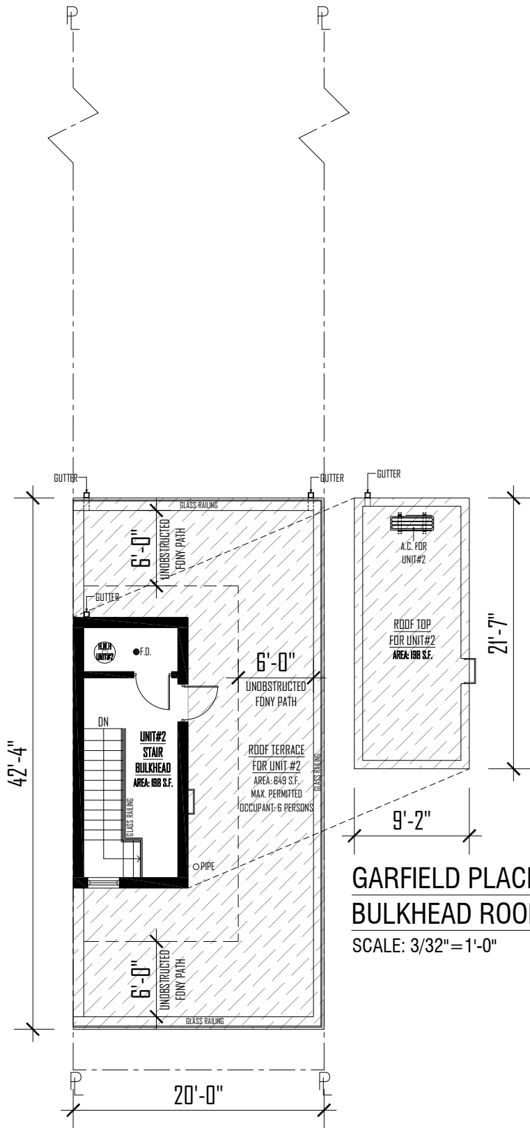
GARFIELD PLACE STAIR BULKHEAD & ROOF PLAN SCALE: 3/32"=1'-0"
