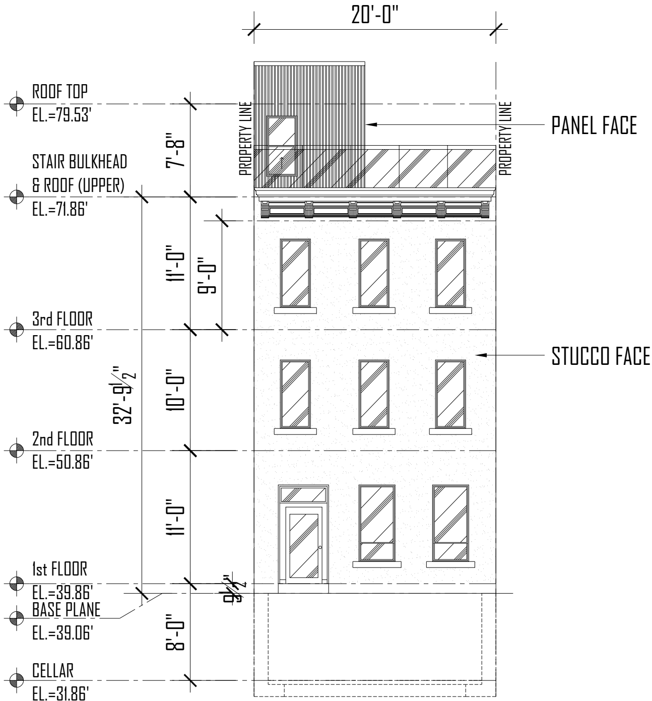
GARFIELD PLACE FRONT ELEVATION PLAN SCALE: 1/8"=1'-0"
