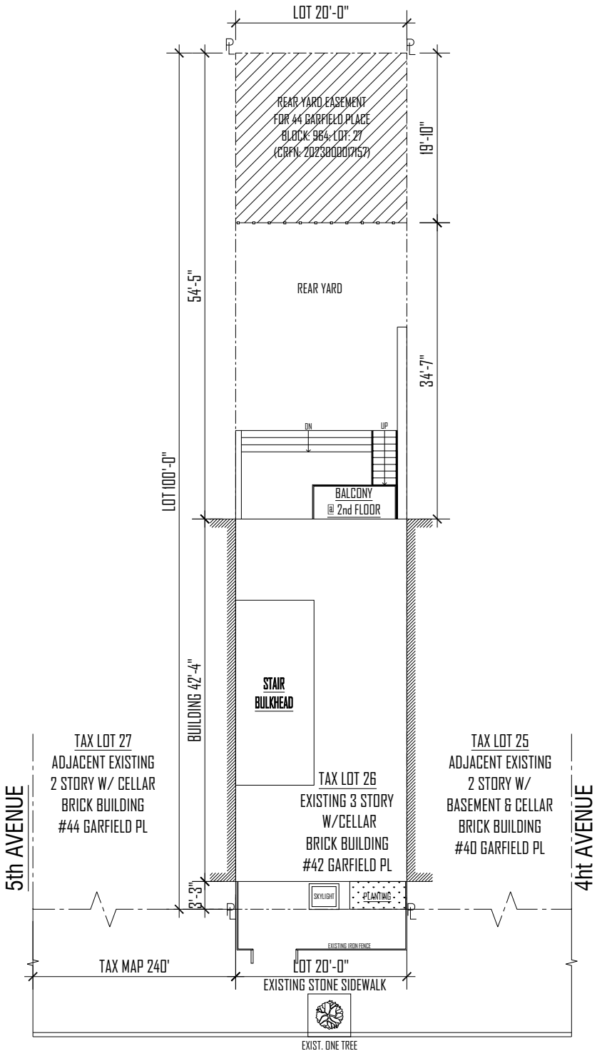
GARFIELD PLACE PLOT PLAN SCALE: 1/16" = 1'-0" BLOCK: 964 LOT: 26 ZONE: R6B MAP: 16C
