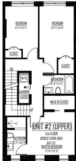
3rd FLOOR PLAN
