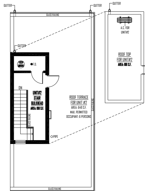
ROOF PLAN
