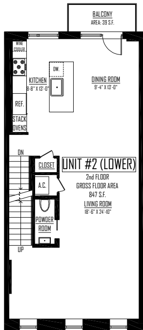
2nd FLOOR PLAN
