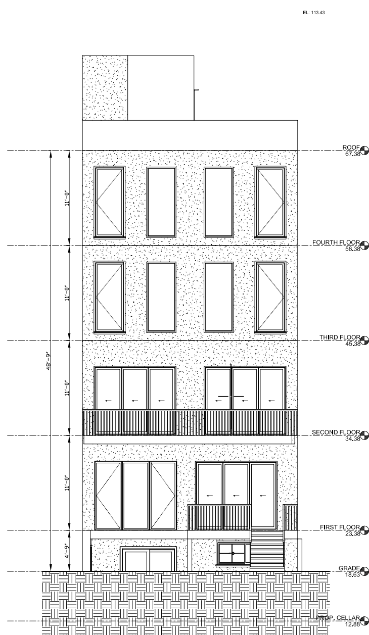
REAR ELEVATION
