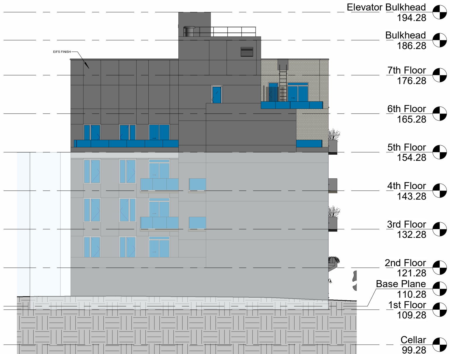
① SOUTH ELEVATION 1/16" = 1'-0"
