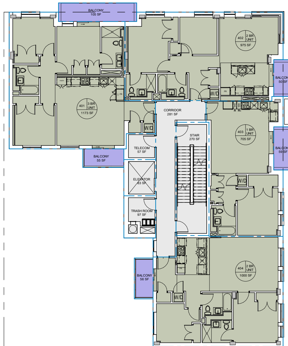
1 4TH FLOOR PLAN 1/16" = 1'-0"
