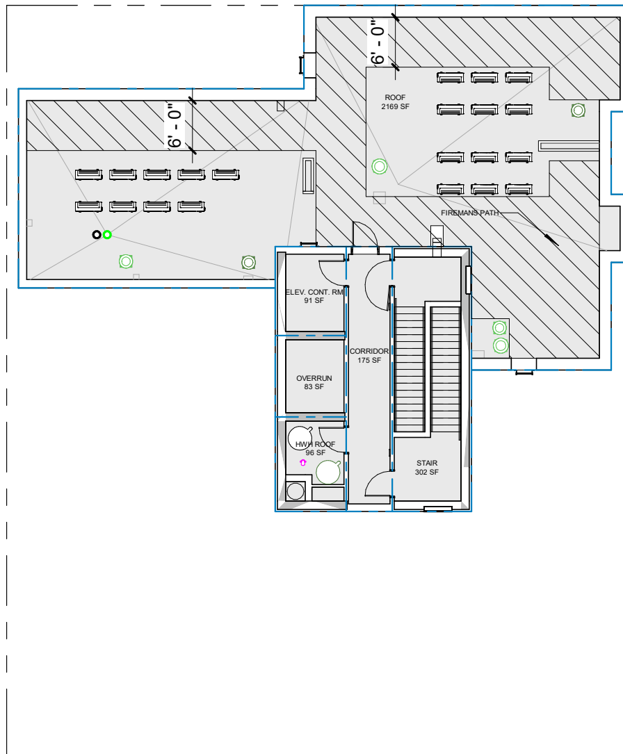
1 ROOF PLAN 1/16" = 1'-0"
