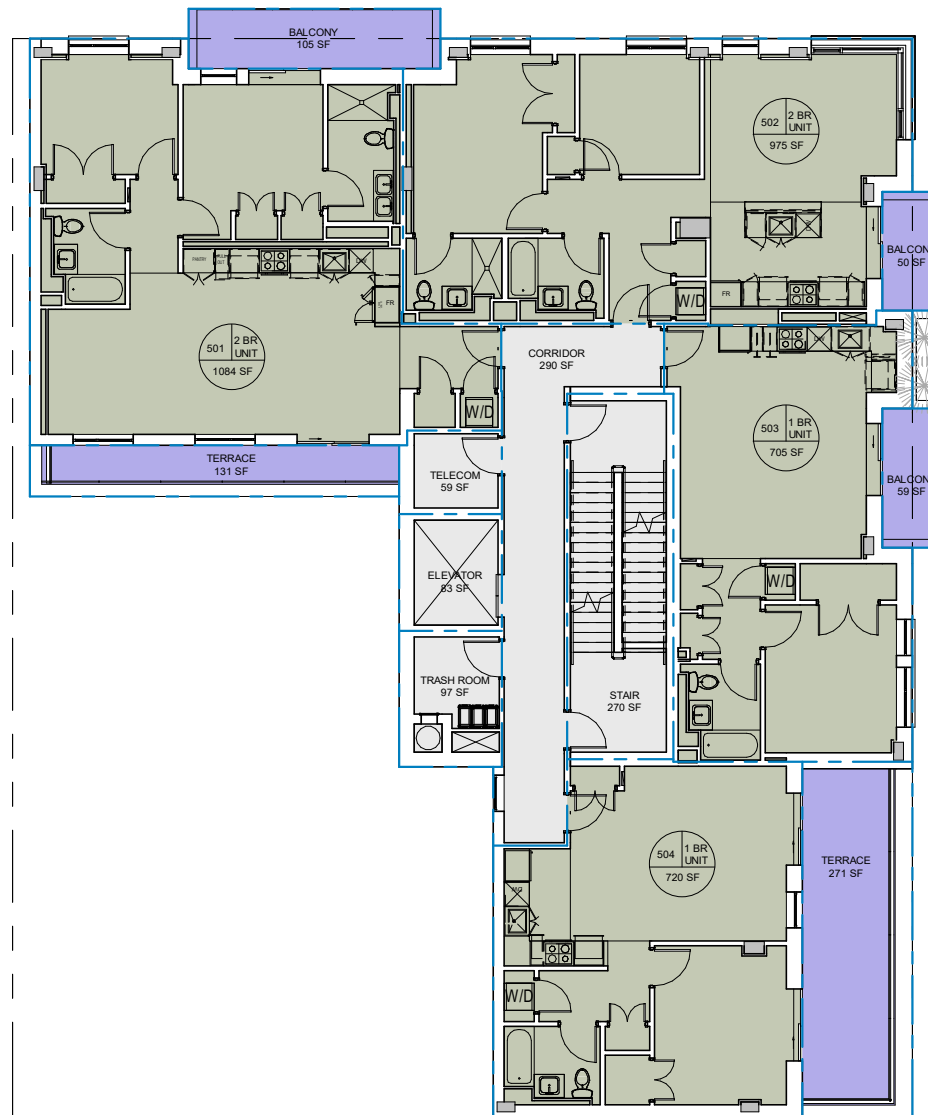
1 5TH FLOOR PLAN 1/16" = 1'-0"
