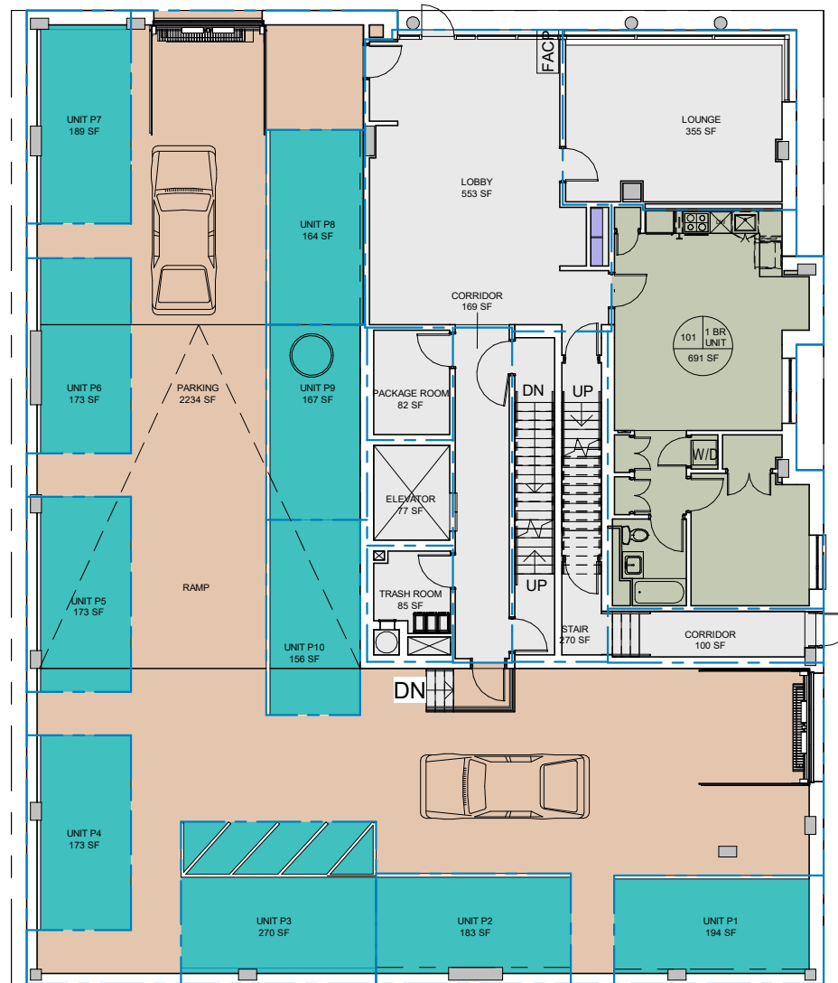
1 1ST FLOOR PLAN 1/16" = 1'-0"
