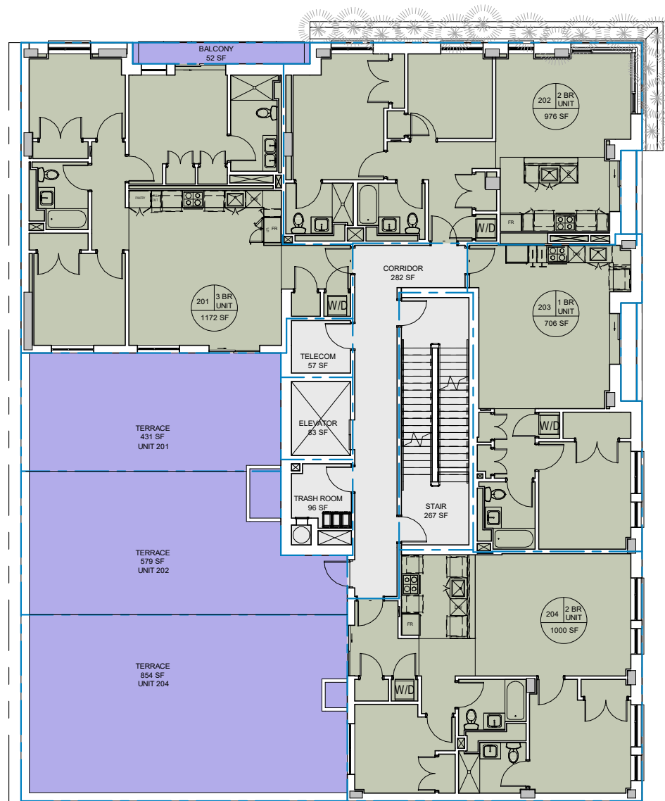
1 2ND FLOOR PLAN 1/16" = 1'-0"
