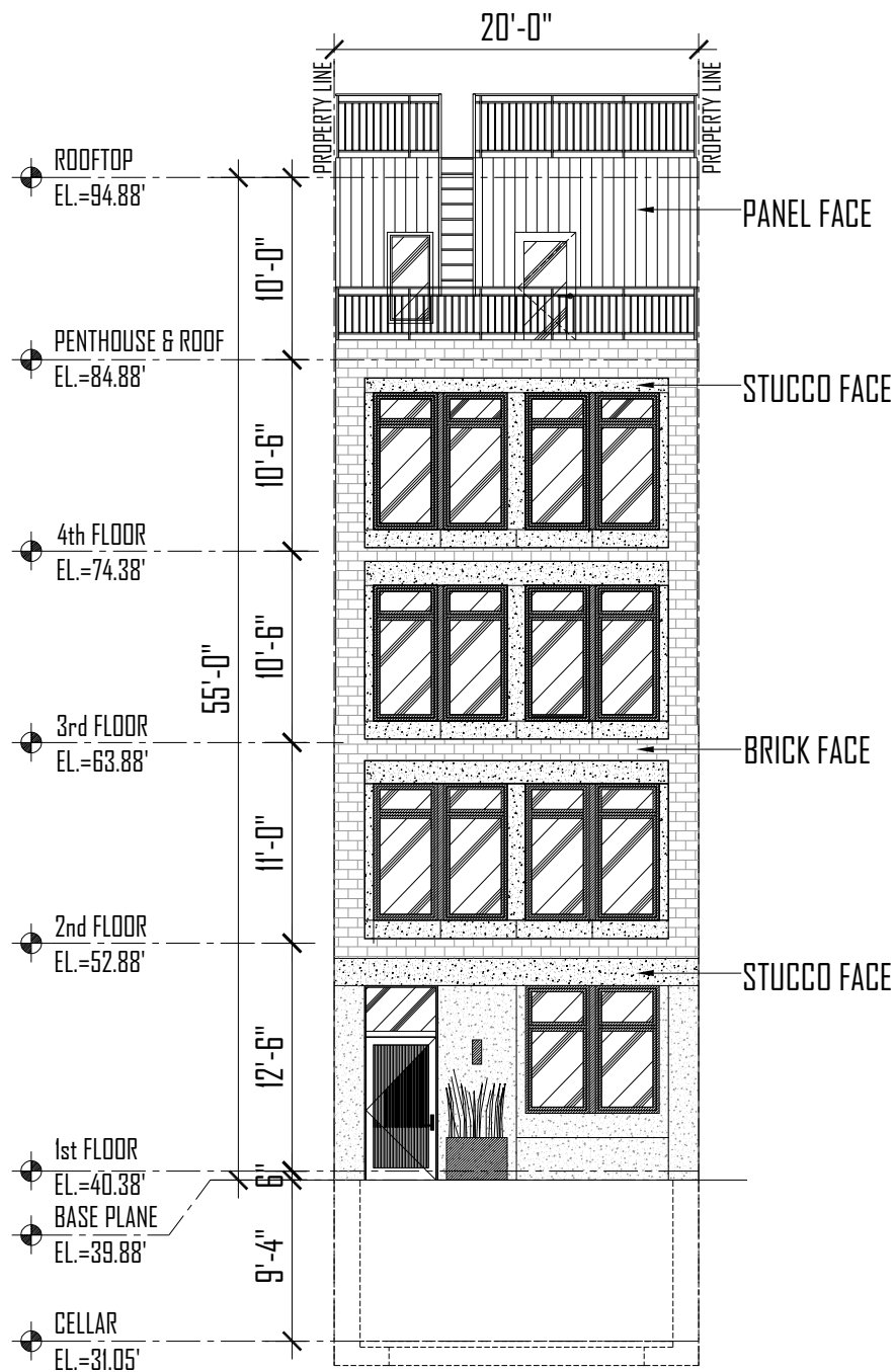
GARFIELD PLACE FRONT ELEVATION PLAN SCALE: 3/32" = 1'-0"
