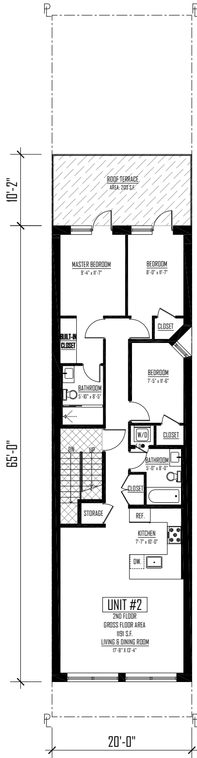
GARFIELD PLACE 2nd FLOOR PLAN SCALE: 3/40"=1'-0"
