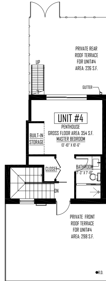
PENTHOUSE & ROOF PLAN
