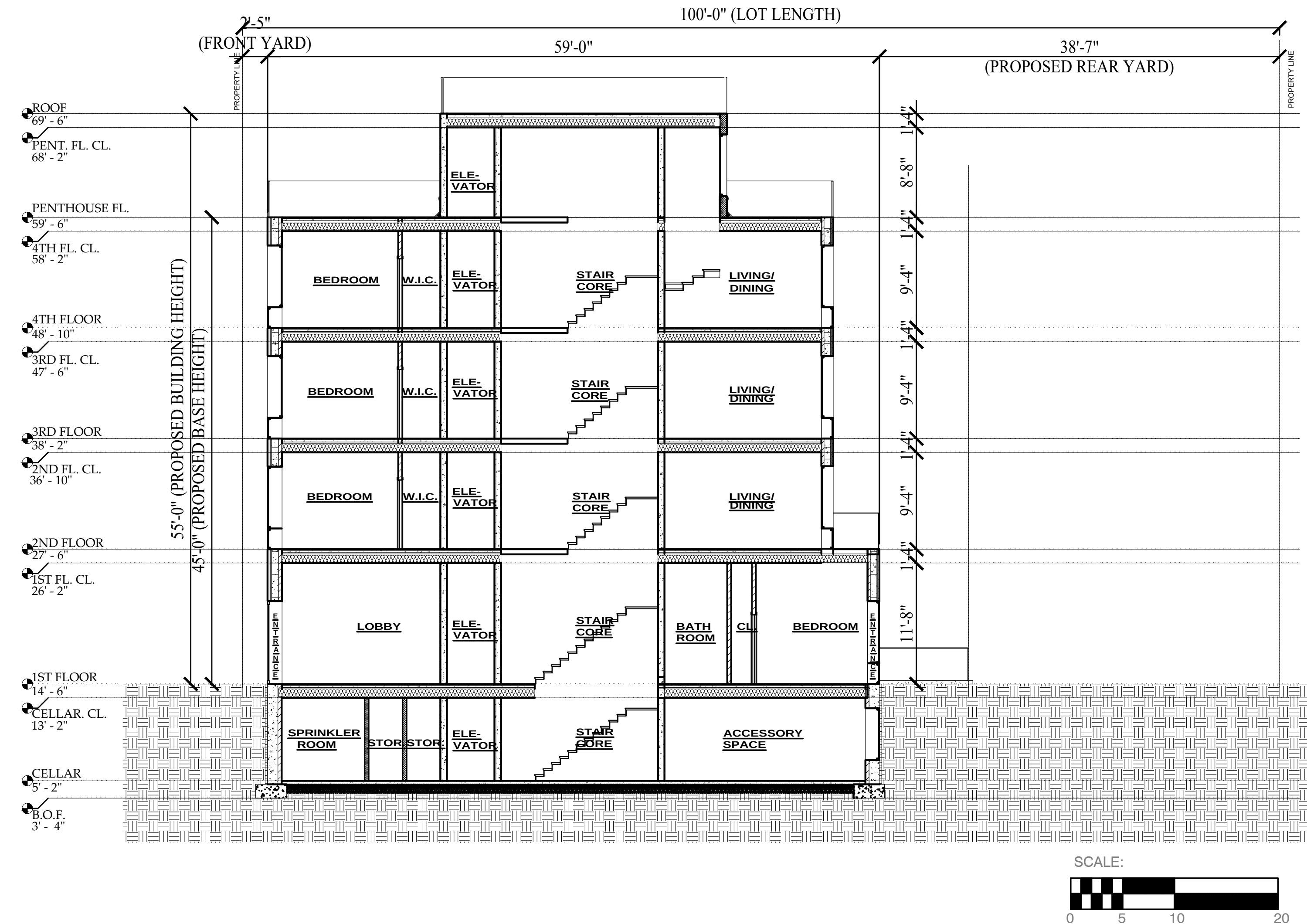
SECTION PLAN
