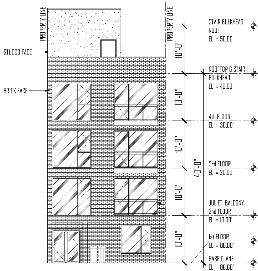
FRONT ELEVATION SCALE: 3/32" = 1'-0"
