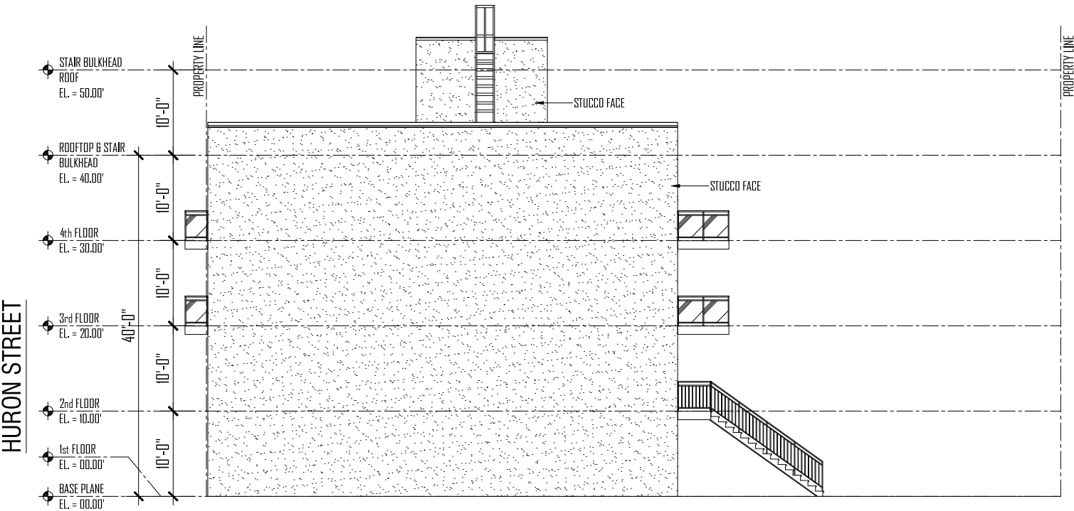
SIDE ELEVATION-RIGHT SCALE: 1/16" = 1'-0"
