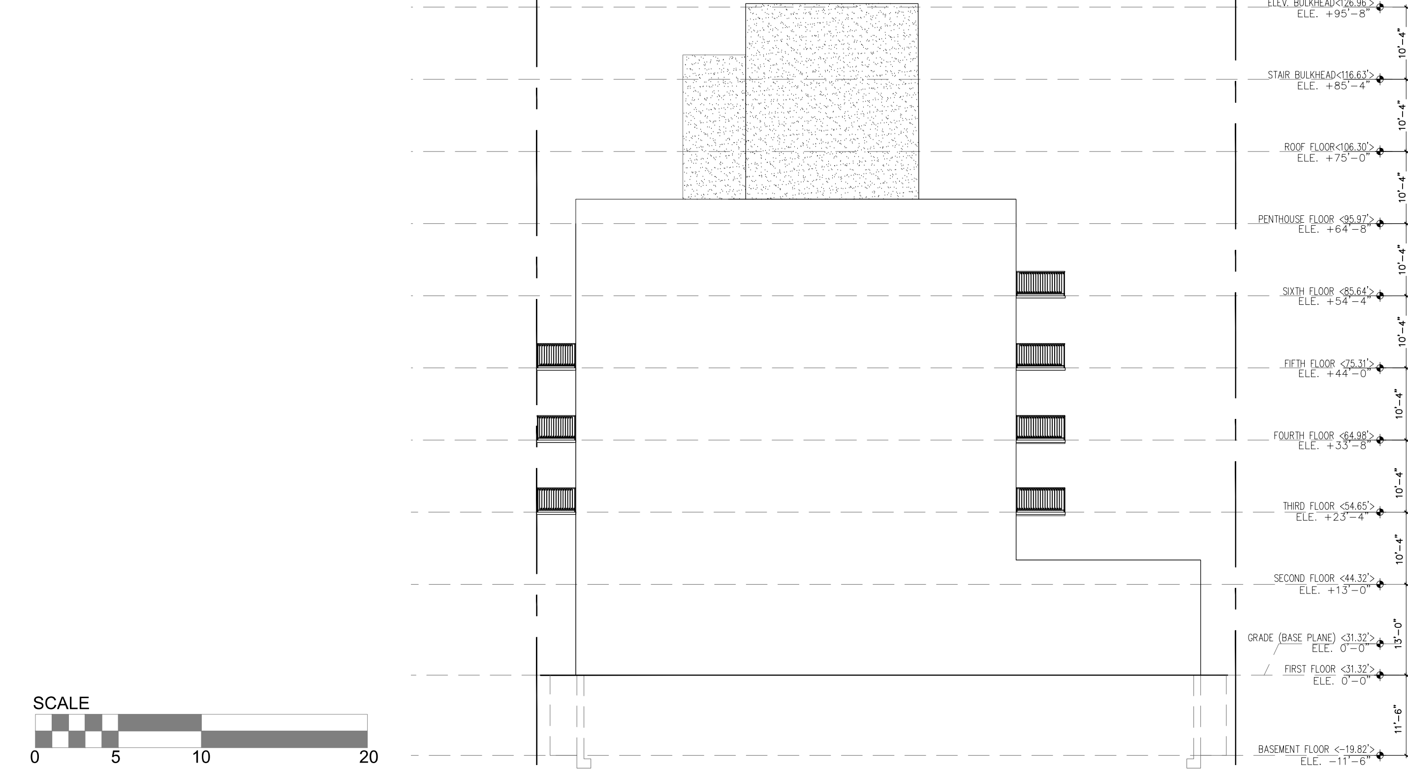
A15 RIGHT SIDE ELEVATION
