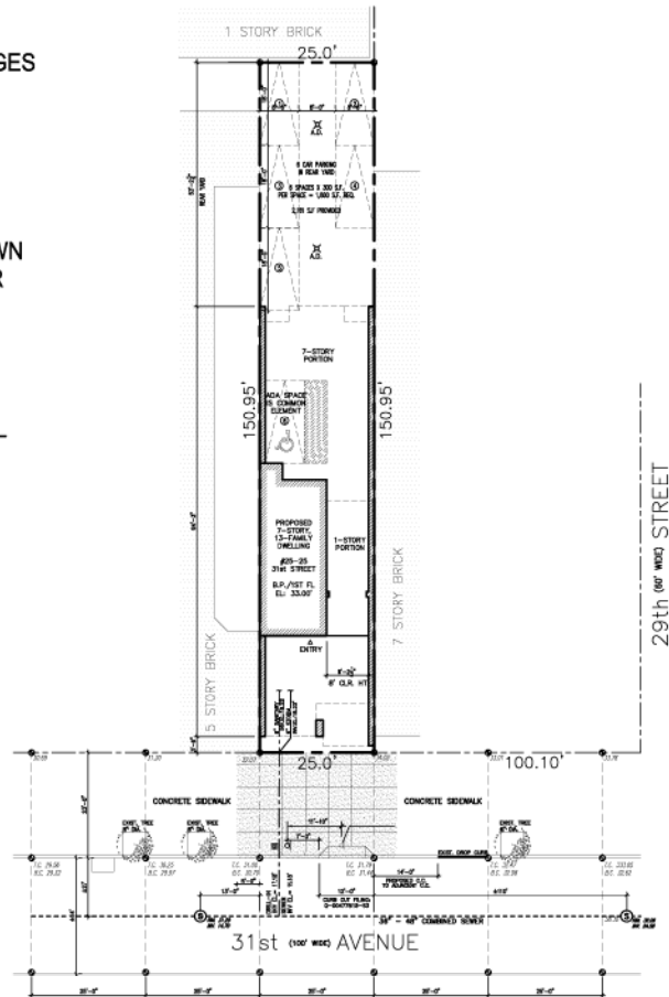
PLOT PLAN SCALE: 1" = 30'-0"
