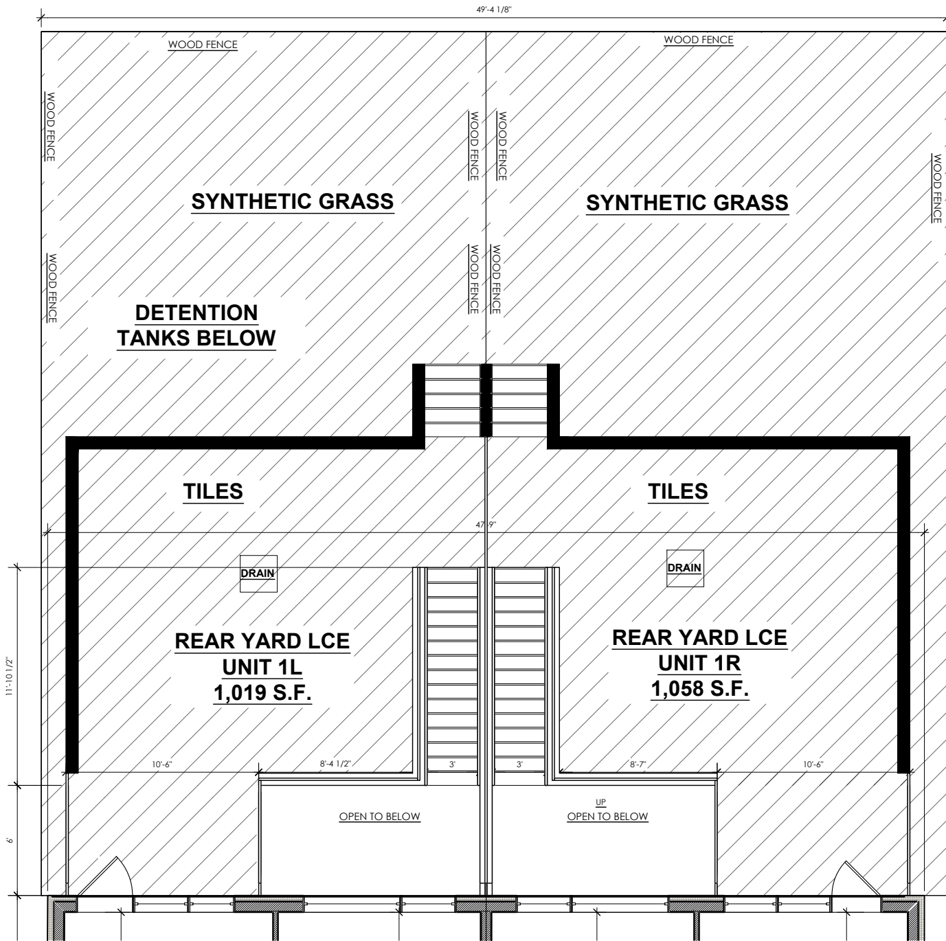
FIRST FLOOR PLAN REAR YARD CONTINUED
