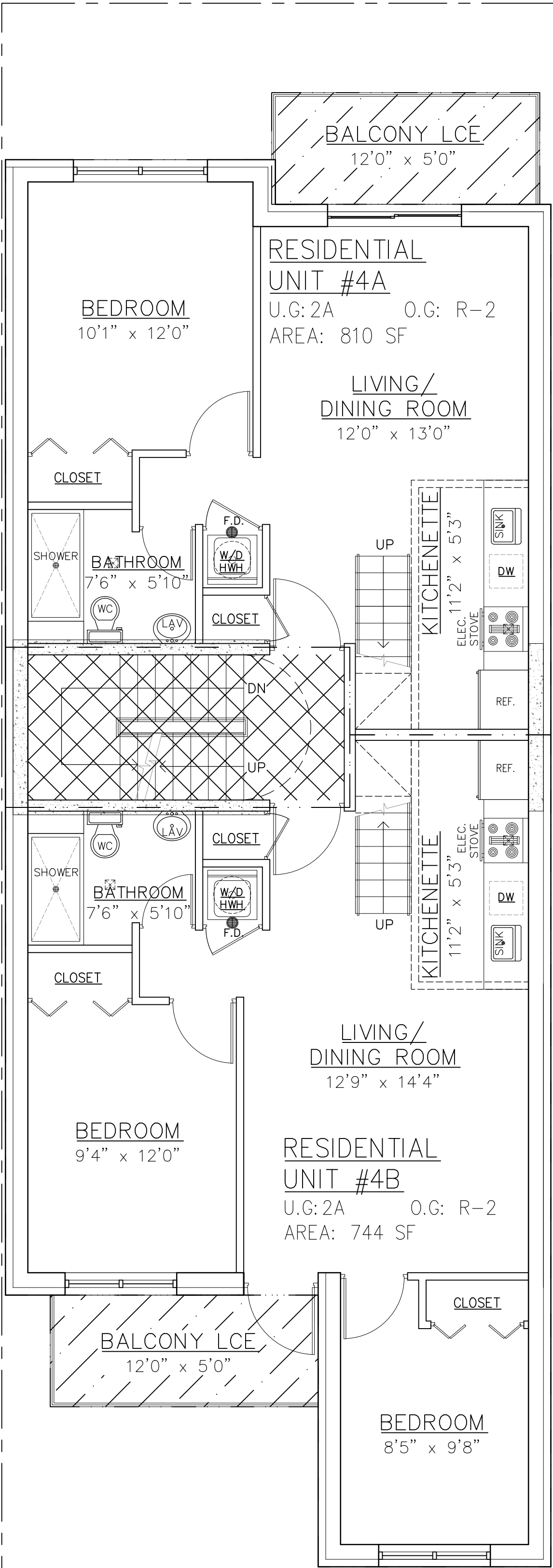
PROPOSED 4th FLOOR PLAN SCALE: 1/8" = 1'-0"
