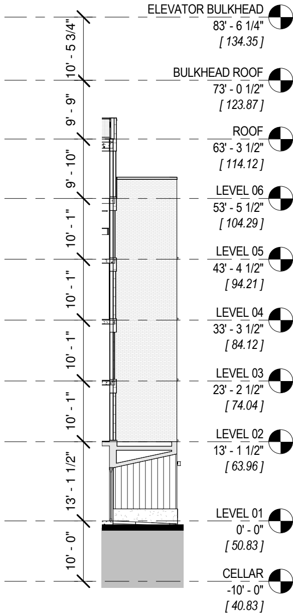
NORTH COURTYARD ELEVATION
