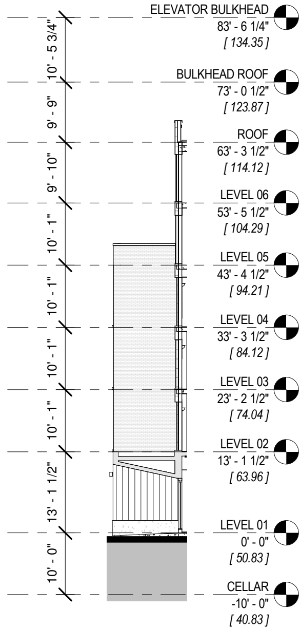
SOUTH COURTYARD ELEVATION
