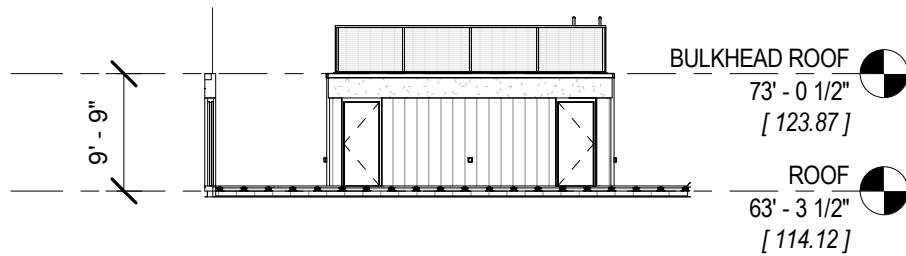
WEST STAIR BULKHEAD ELEVATION
