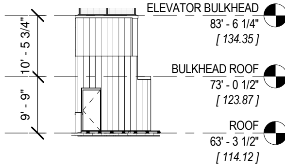
ELEVATOR BULKHEAD ELEVATION
