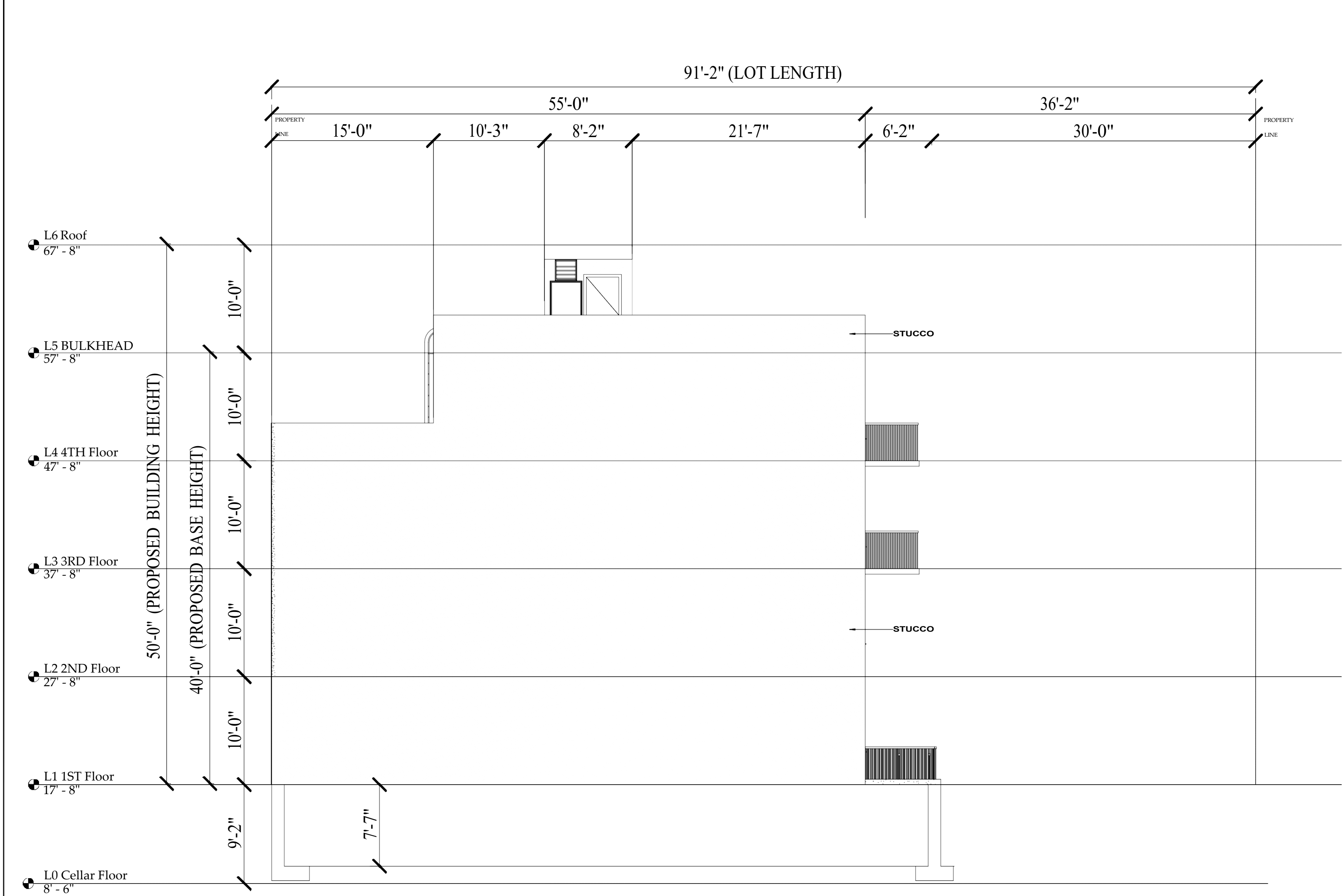
SIDE ELEVATION (WEST)
