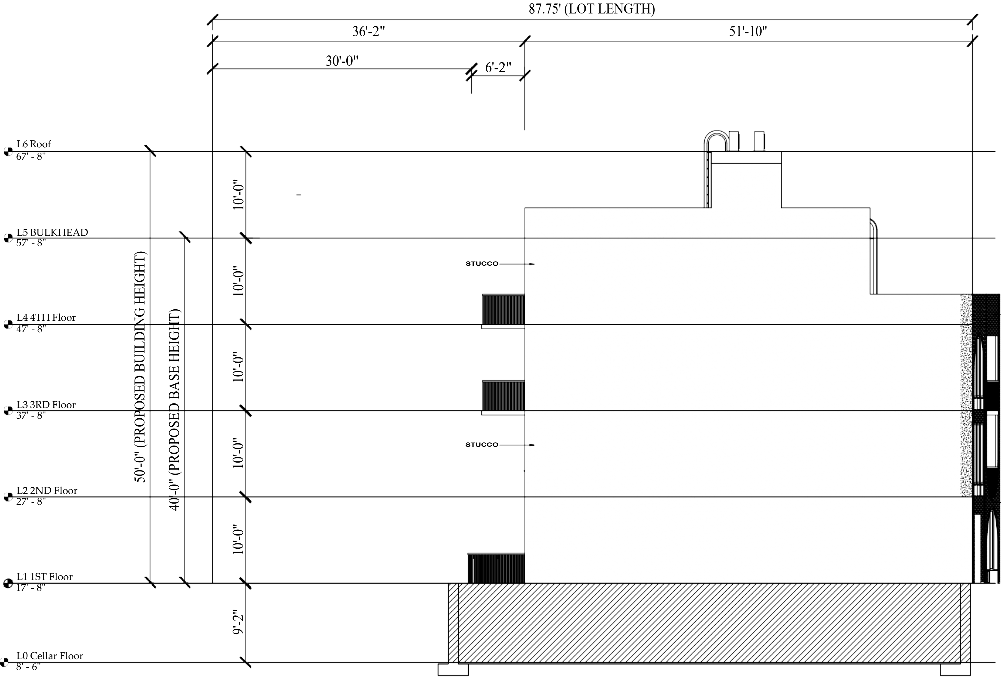
SIDE ELEVATION (EAST)
