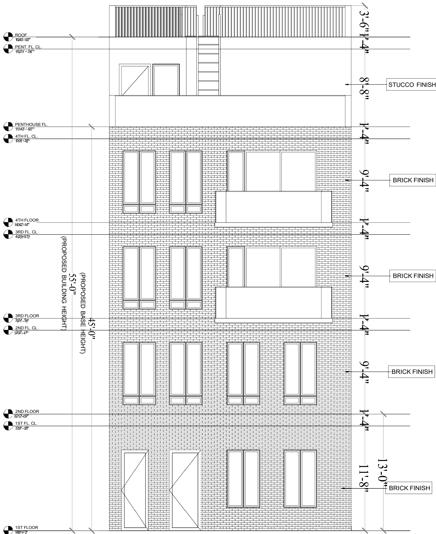
FRONT ELEVATION (NORTH)
