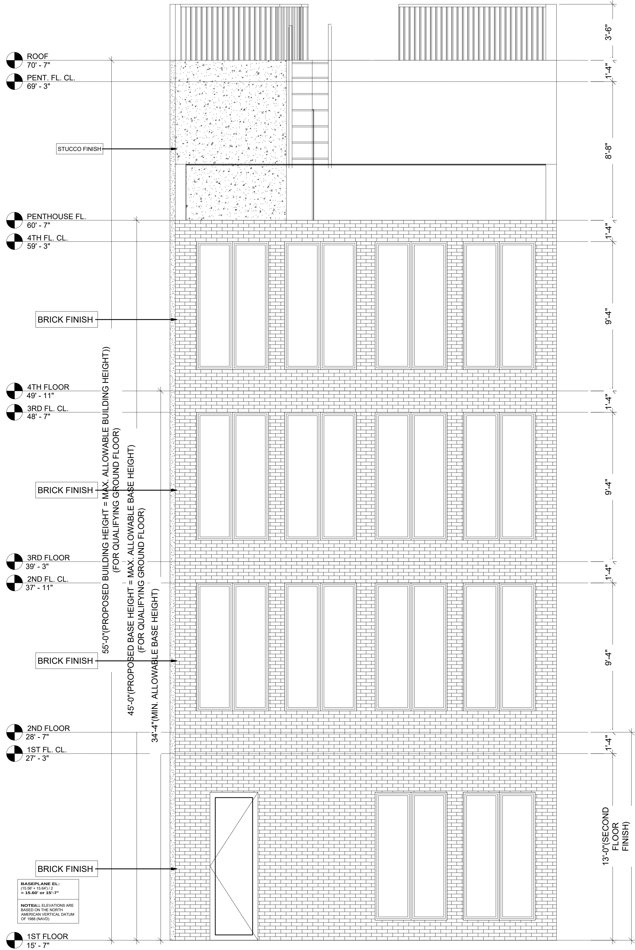
FRONT ELEVATION (NORTH)
