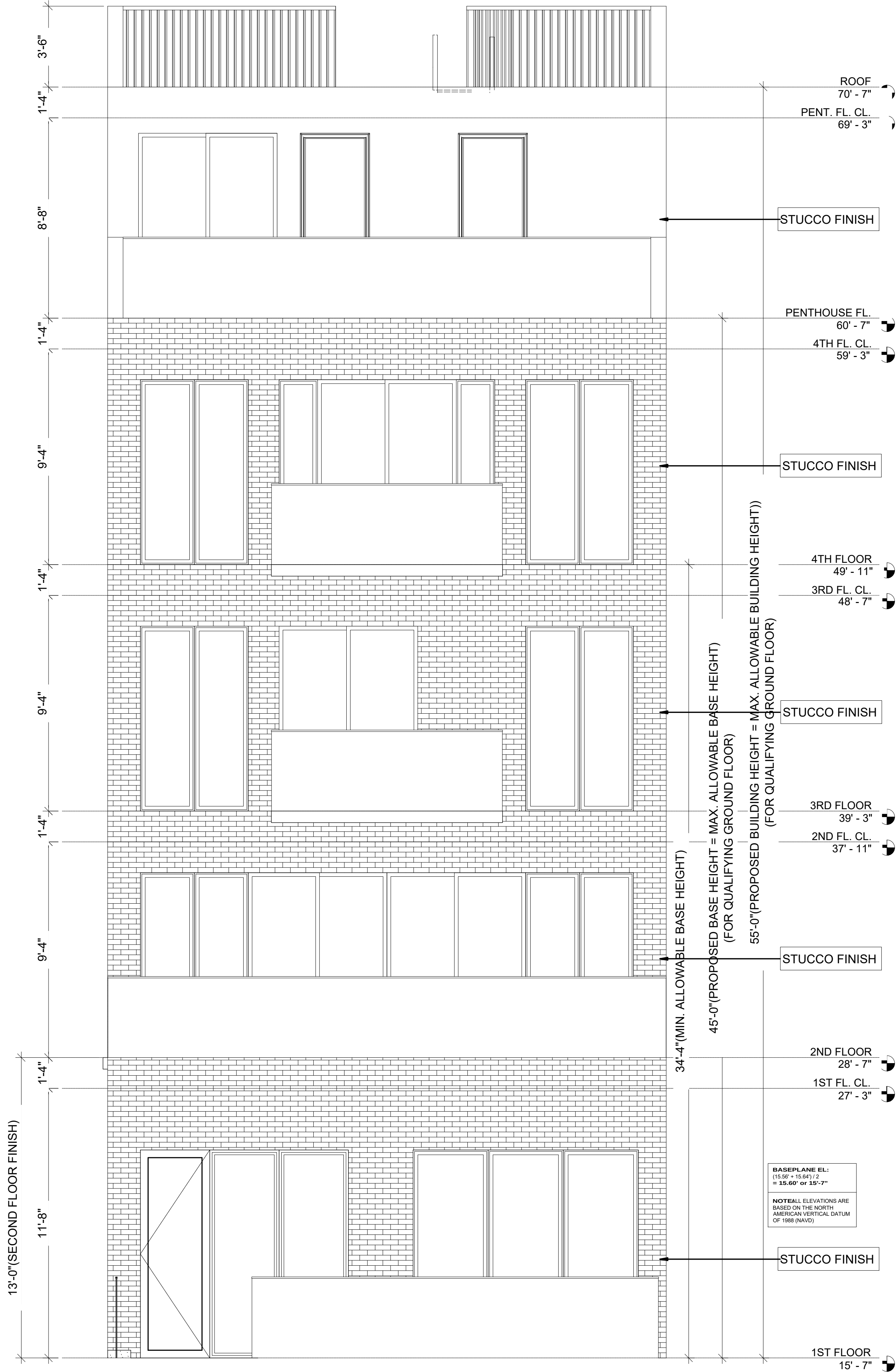
BACK ELEVATION (SOUTH)
