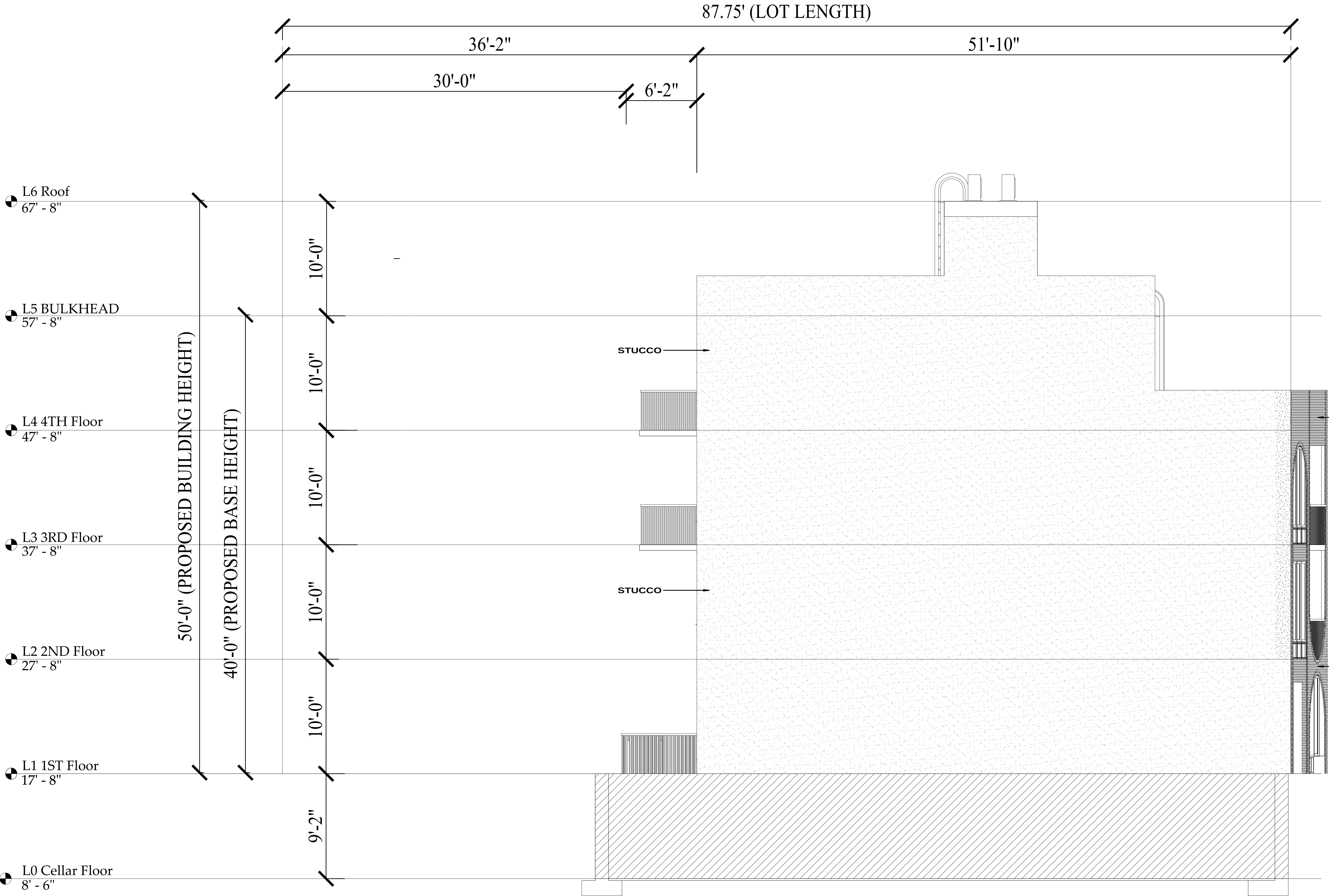
SIDE ELEVATION (EAST)
