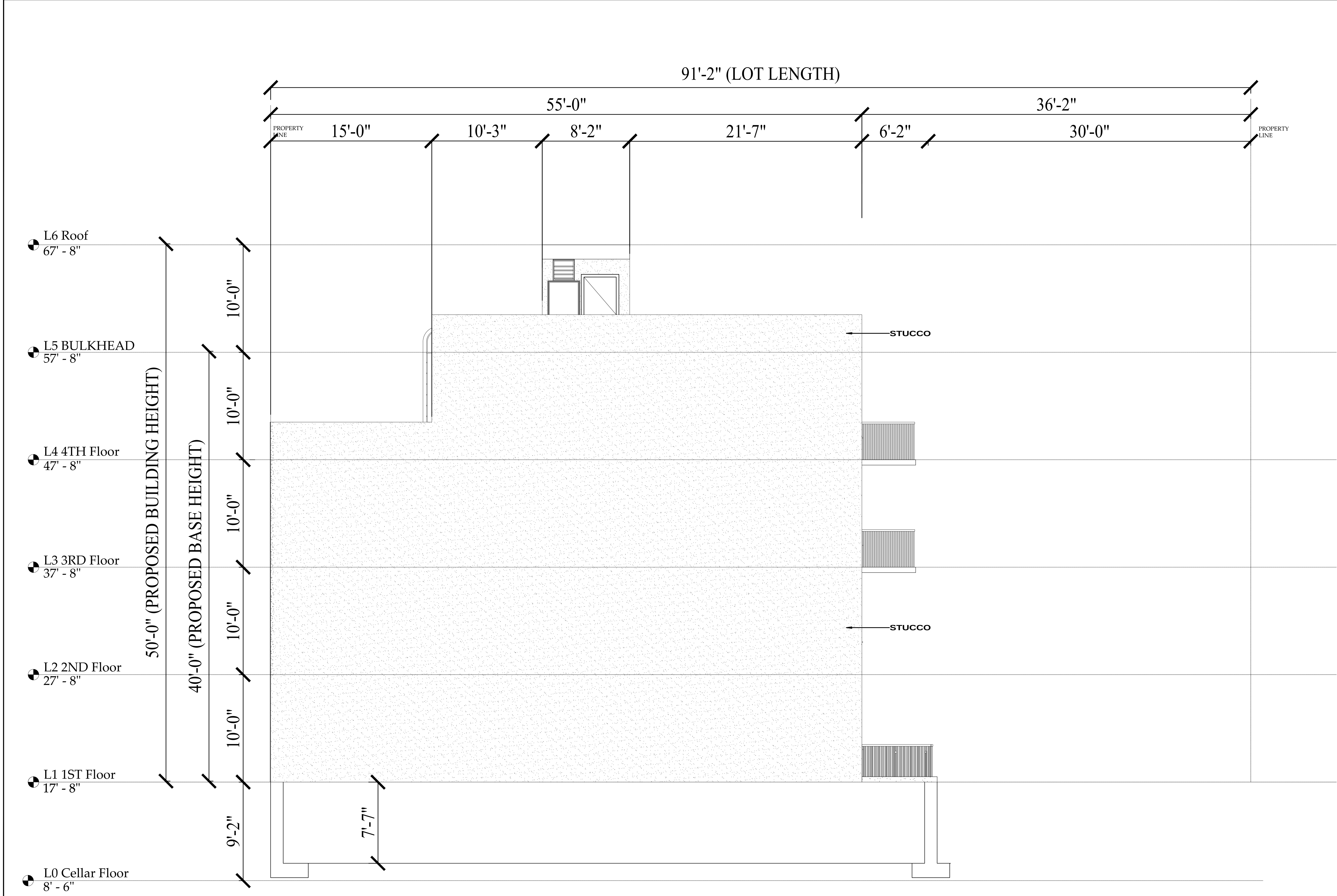
SIDE ELEVATION (WEST)
