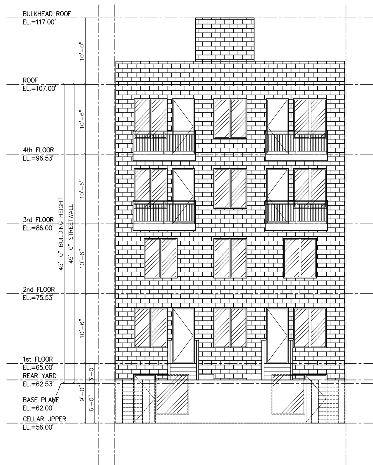
REAR ELEVATION PLAN SCALE: 1/4"=1'-0" BASE PLANE CALCULATION: (AS PER ZR 12-10) (61.55' + 62.45') / 2 = 62.00'
