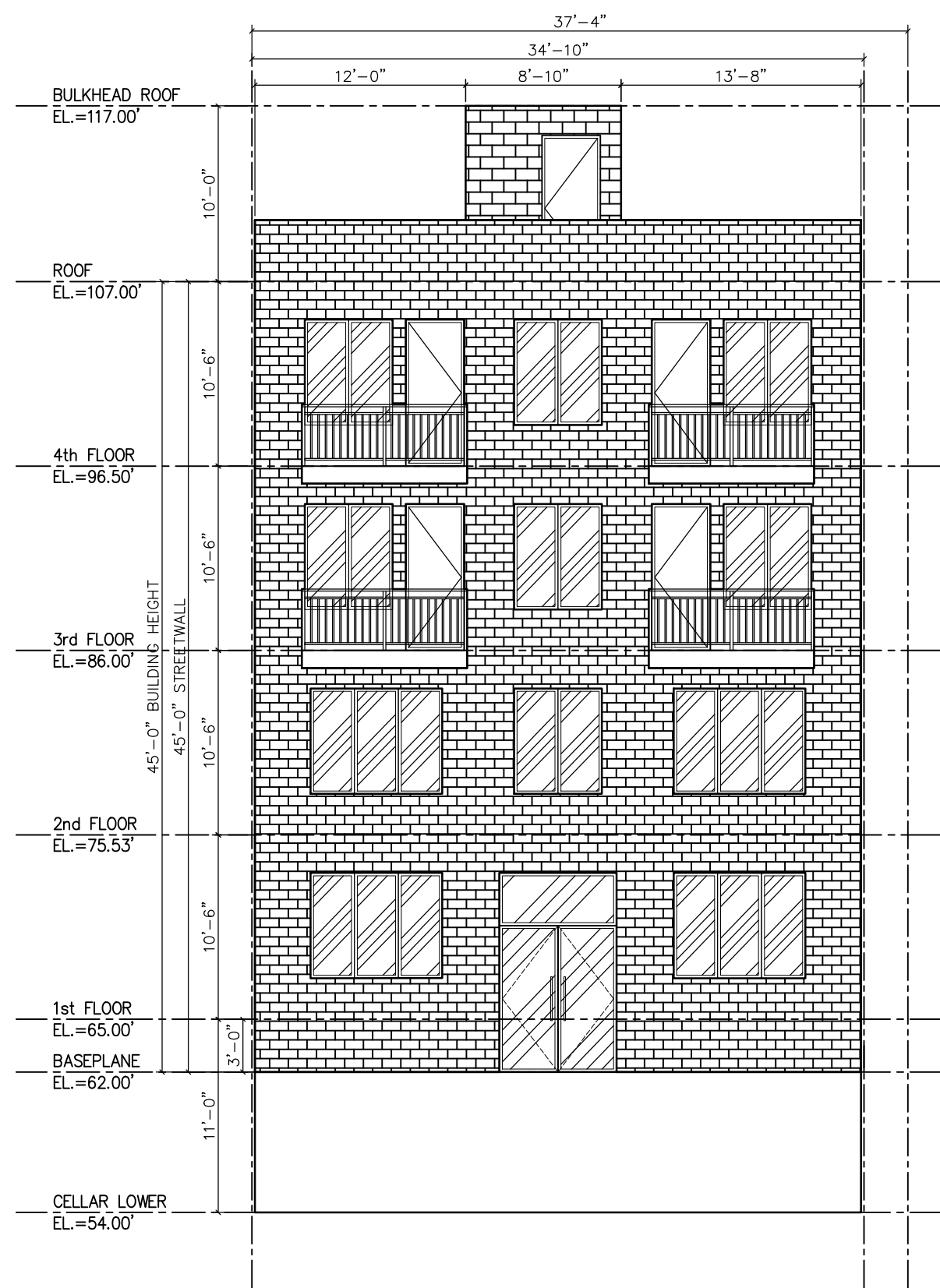
FRONT ELEVATION PLAN SCALE: 1/4"=1'-0" BASE PLANE CALCULATION: (AS PER ZR 12-10) (61.54' + 62.45') / 2 = 62.00'
