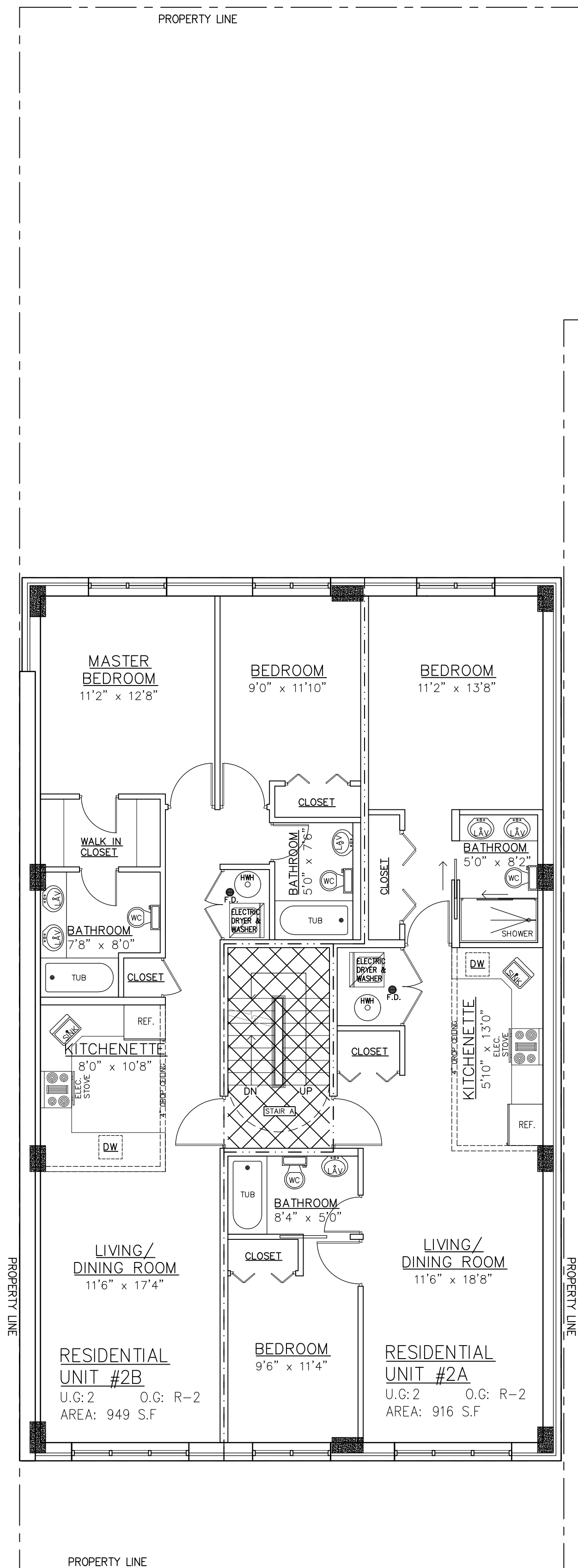
PROPOSED 2ND FLOOR PLAN SCALE: 3/32" = 1'-0"
