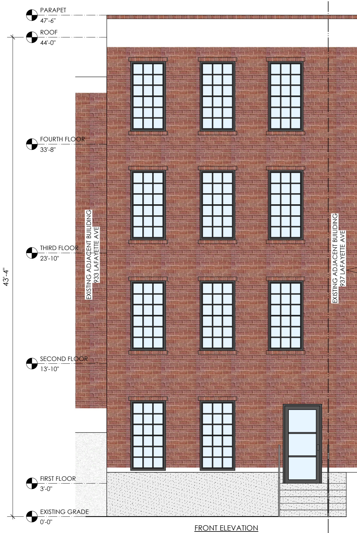
FRONT ELEVATION
