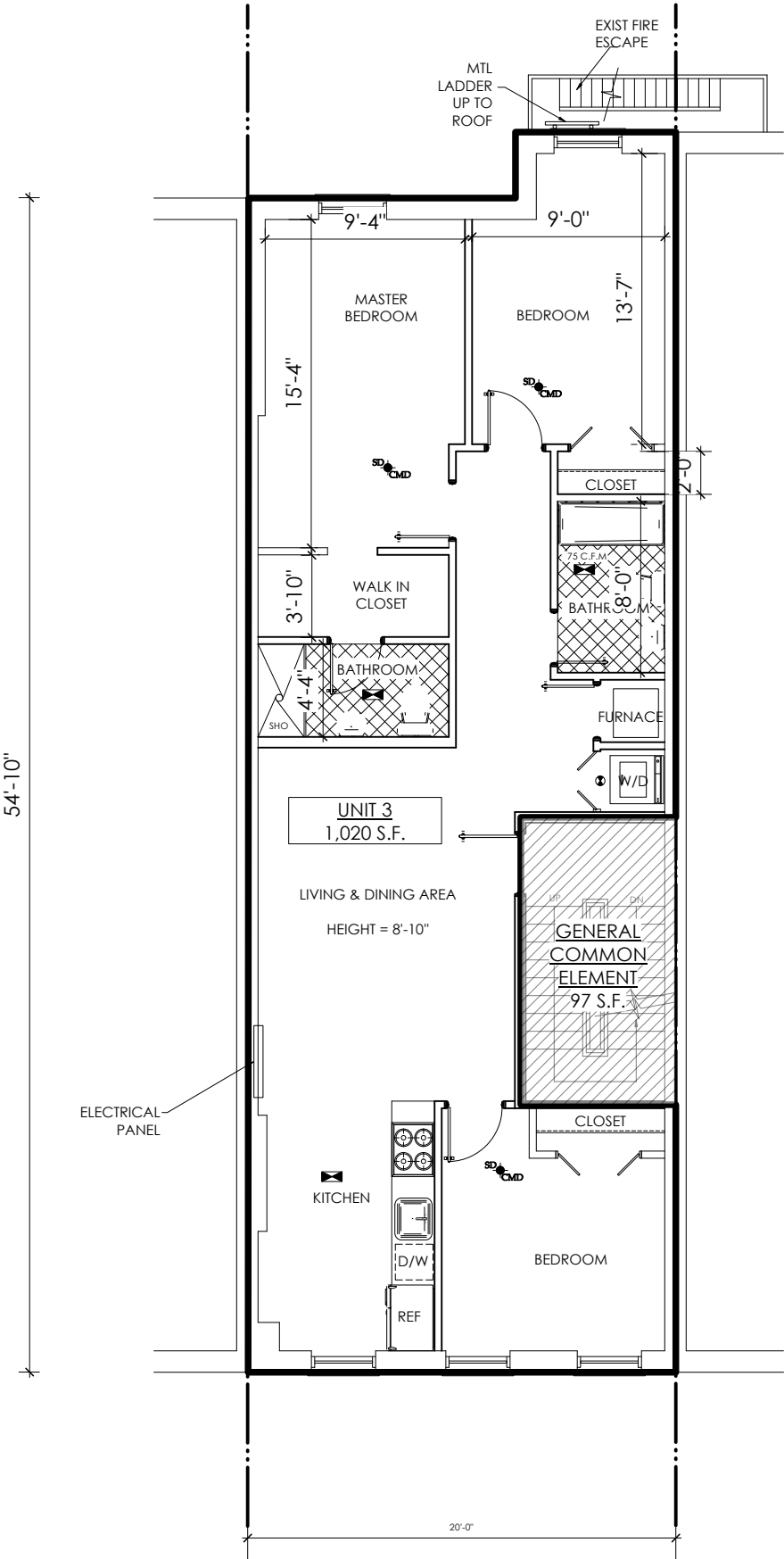
1 THIRD FLOOR PLAN Scale: 1/8" = 1'-0"
