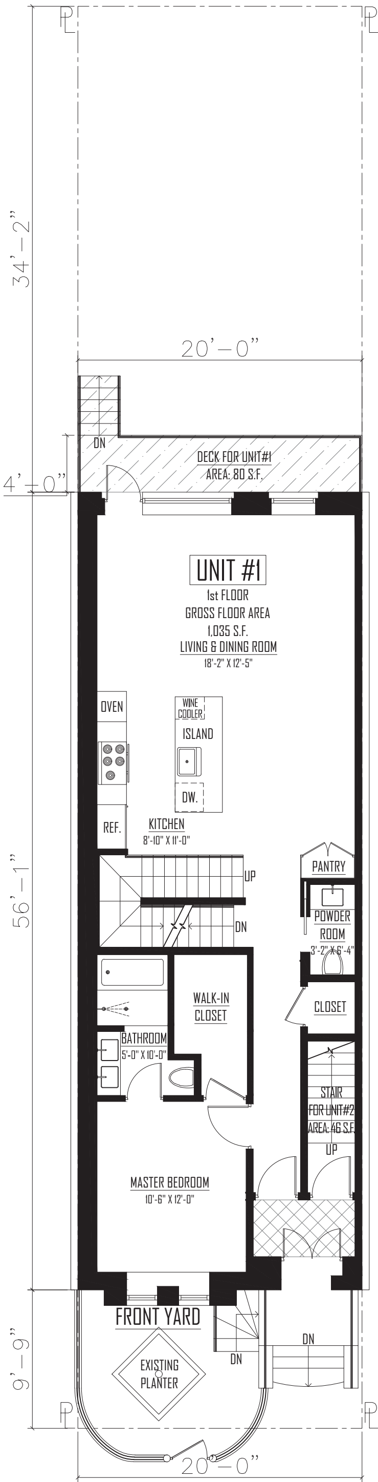
10th STREET 1st FLOOR PLAN SCALE: 3/40" = 1'-0"
