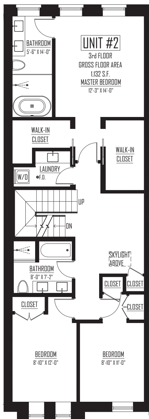
3rd FLOOR PLAN
