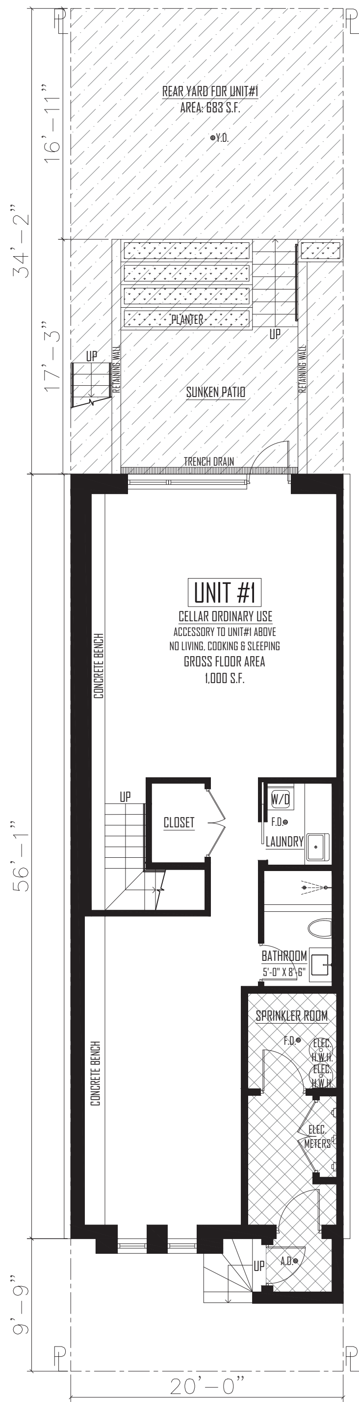
10th STREET CELLAR PLAN SCALE: 3/40" = 1'-0"
