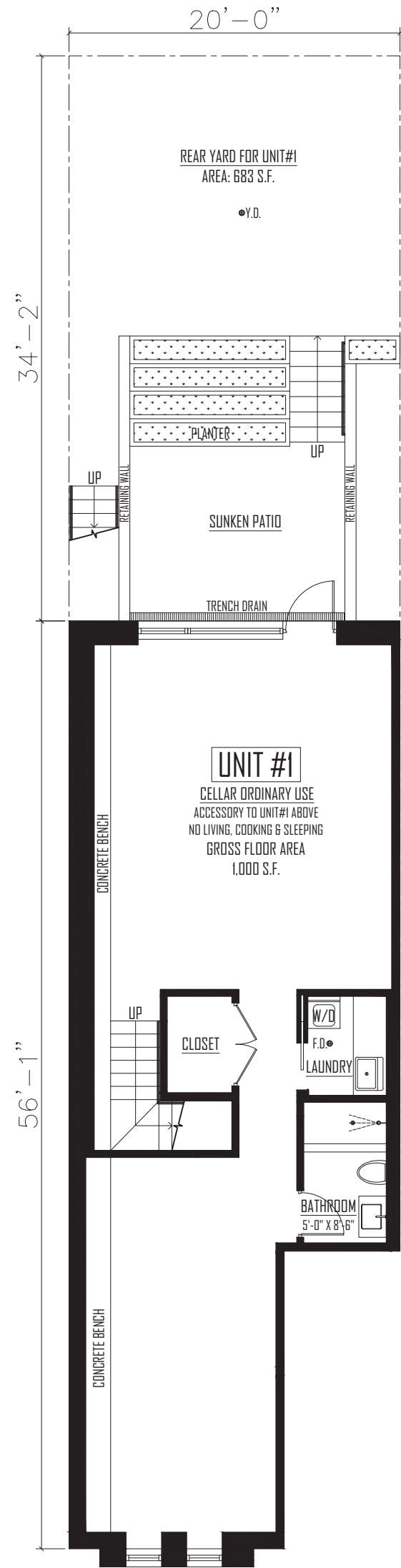
CELLAR PLAN
