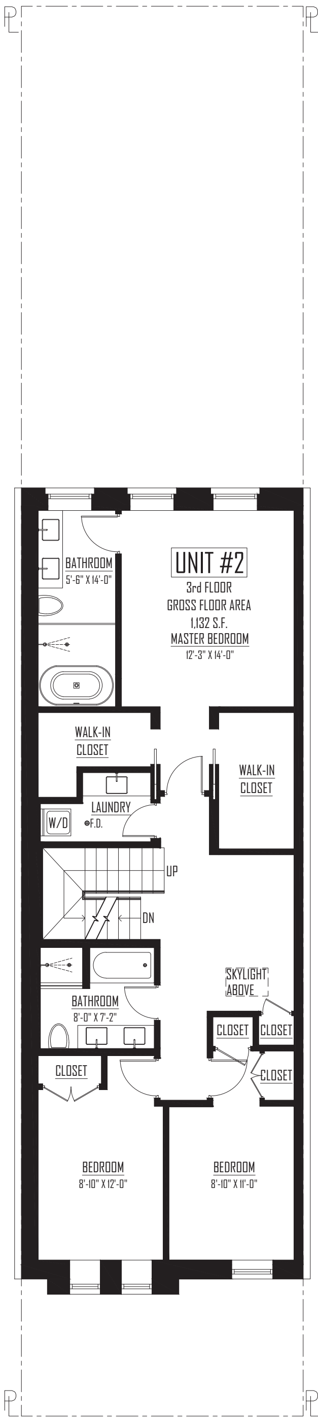
10th STREET 3rd FLOOR PLAN SCALE: 3/40" = 1'-0"
