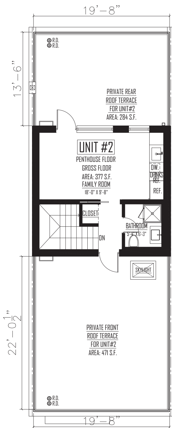
PENTHOUSE & ROOF PLAN
