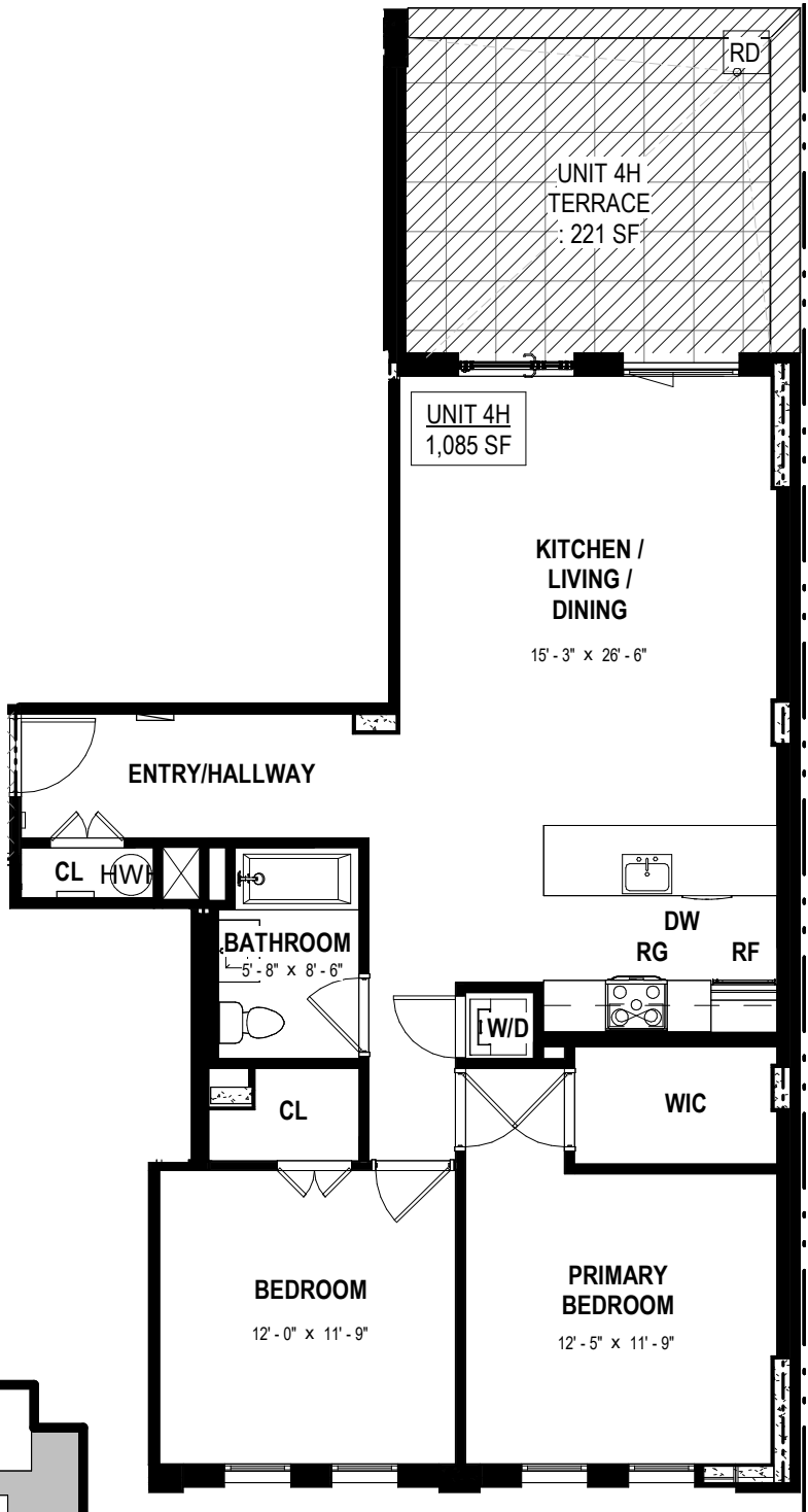
LEVEL 04 - UNIT 4H
