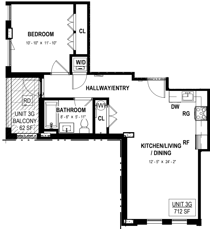
LEVEL 03 - UNIT 3G
