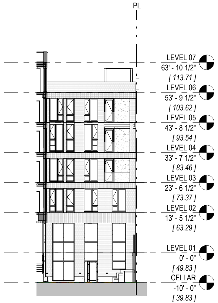
INNER COURT ELEVATION 02
