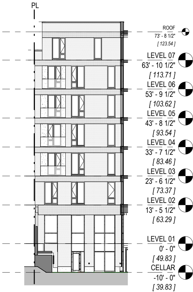
INNER COURT ELEVATION 01
