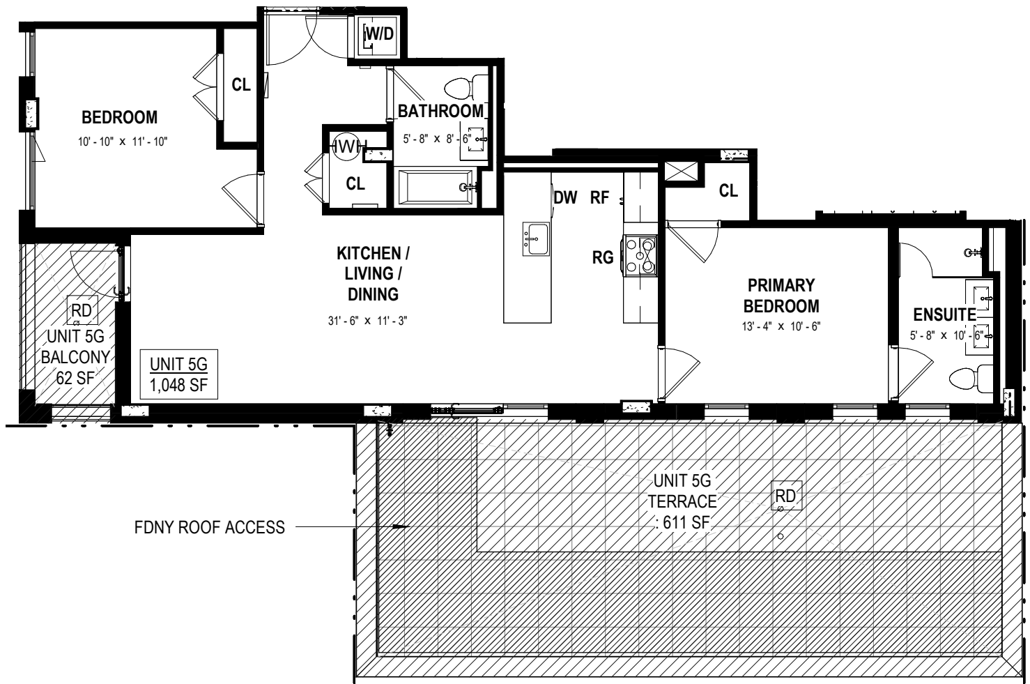
LEVEL 05 - UNIT 5G
