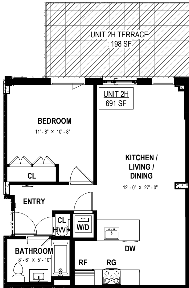
LEVEL 02 - UNIT 2H
