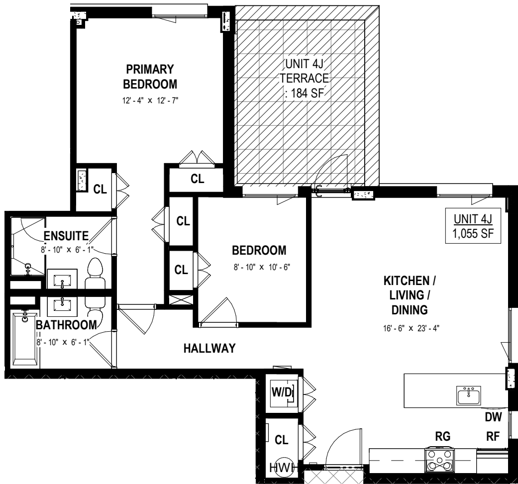
LEVEL 04 - UNIT 4J
