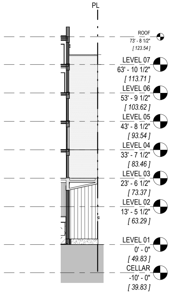
OUTER COURT ELEVATION 02
