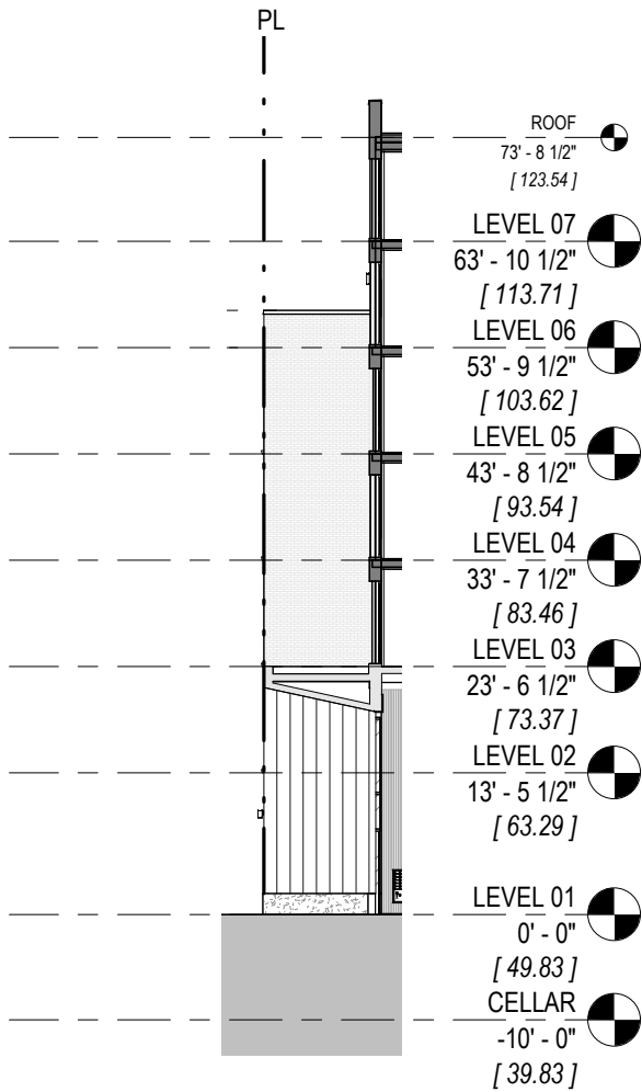
OUTER COURT ELEVATION 01
