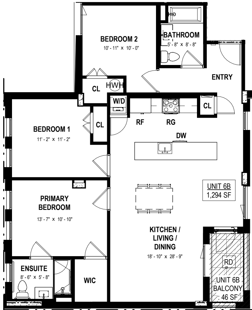
LEVEL 06 - UNIT 6B
