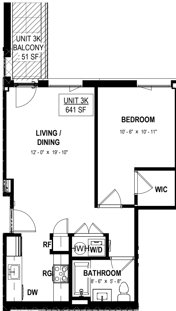
LEVEL 03 - UNIT 3K
